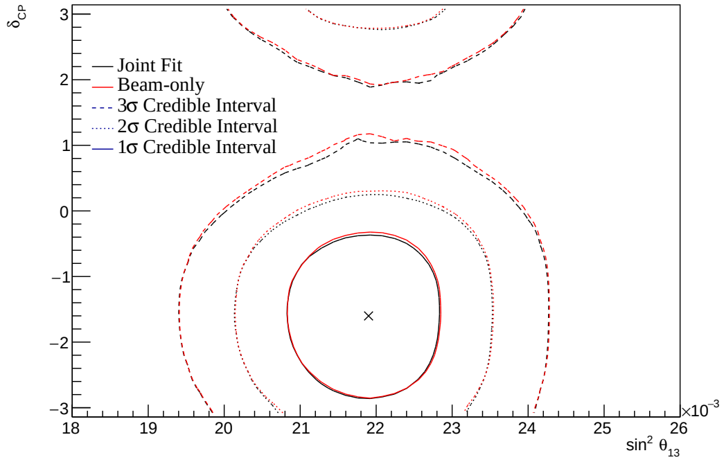
Figure 8.40: The two-dimensional posterior probability density distribution in \delta_{CP}-\sin^2(\theta_{13}) compared between the joint beam-atmospheric fit (Black) and the latest T2K sensitivities (Red) [2, 212]. The reactor constraint is applied in both fits. The distributions are marginalised over both hierarchies. The marker represents the known value of \delta_{CP}-\sin^2(\theta_{13}) .
