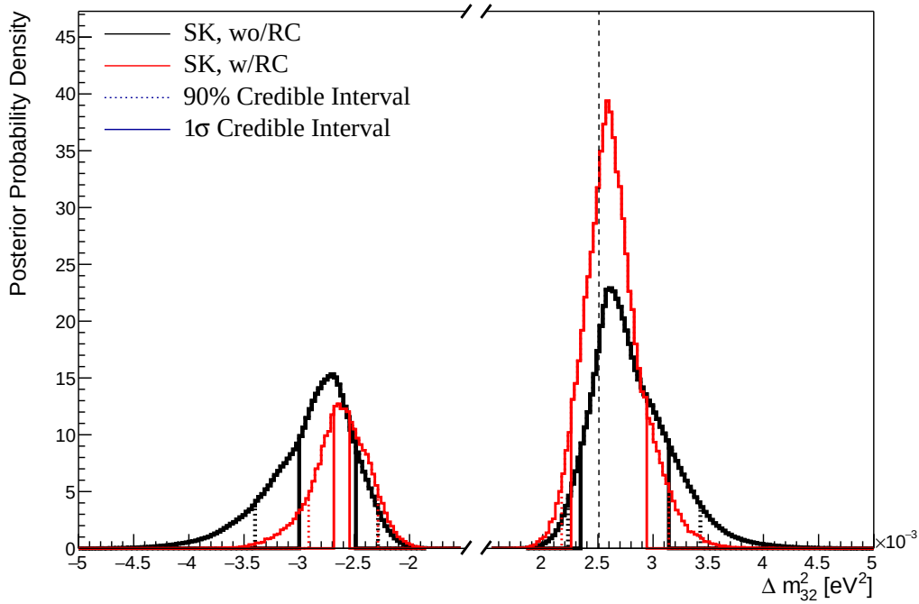
Figure 8.13: The one-dimensional posterior probability density distribution in \Delta m_{32}^2 compared between the SK atmospheric-only fit (Black) and the SK atmospheric fit with the reactor constraint applied (Red). The distributions are marginalised over both hierarchies. The vertical dashed line represents the known value of \Delta m_{32}^2 .
