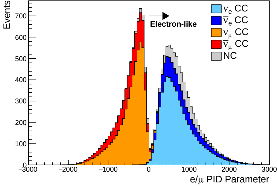
Figure 5.5: The electron/muon PID separation parameter for all sub-GeV single-ring events in SK-IV. The charged current (CC) component is broken down in four flavours of neutrino ( \nu_\mu , \bar{\nu}_\mu , \nu_e and \bar{\nu}_e ). Events with positive values of the parameter are determined to be electron-like.
