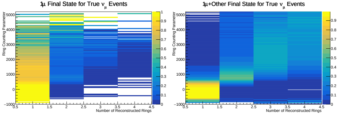
Figure 6.14: The ring counting parameter, defined in Equation 6.6, as a function of the number of reconstructed rings as found by the fitQun reconstruction algorithm. Left: true \nu_\mu events with only one muon above the Cherenkov threshold in the final state. Right: true \nu_\mu events with one muon and at least one other charged particle above the Cherenkov threshold in the final state.
