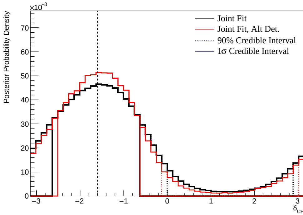
Figure 8.47: The one-dimensional posterior probability density distribution in \delta_{CP} compared between the joint beam-atmospheric fit described in subsection 8.3.4 (Black) and the joint beam-atmospheric fit using the correlated detector model (Red). The reactor constraint is not applied in either fit. The distributions are marginalised over both hierarchies. The vertical dashed line represents the known value of \delta_{CP} .
