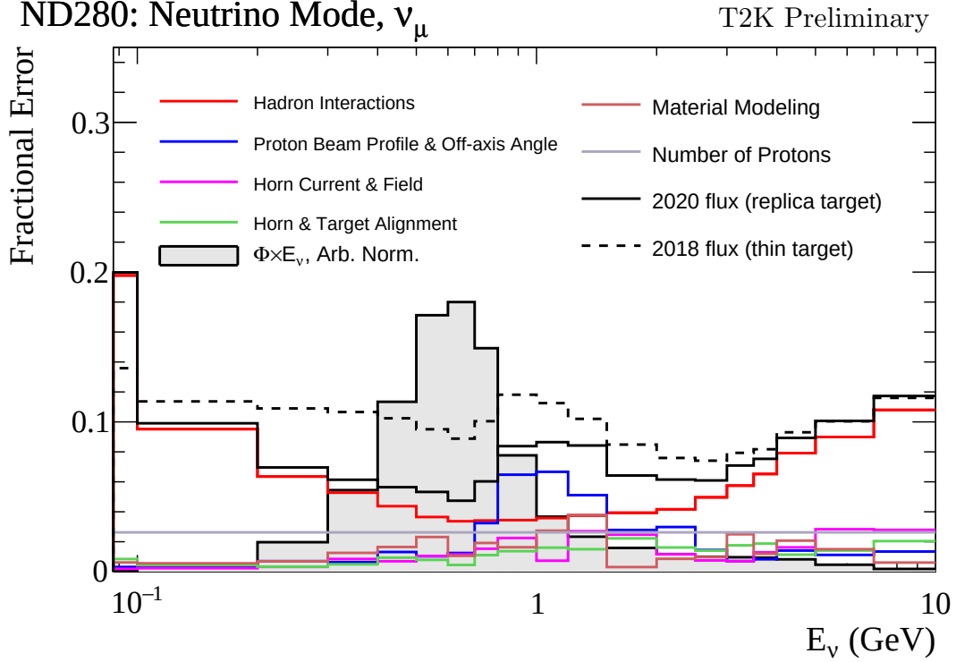
Figure 6.7: The total uncertainty evaluated on the near detector \nu_\mu flux prediction constrained by the replica-target data, illustrated as a function of neutrino energy. The solid(dashed) line indicates the uncertainty used within this analysis(the T2K 2018 analysis [191]). The solid histogram indicates the neutrino flux as a function of energy. Figure taken from [192].
