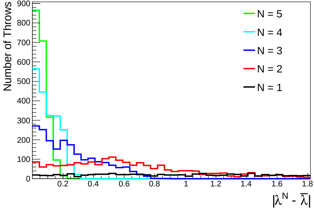
Figure 7.5: The distribution of |\lambda^N - \bar{\lambda}| for various values of N . As expected, the distribution gets narrower for larger values of N .
