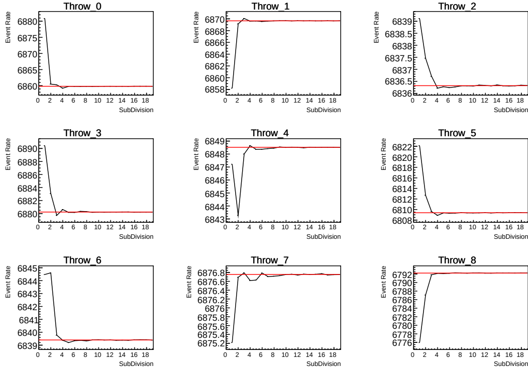
Figure 7.3: Event rate of the SubGeV_ellike_0dcy sample as a function of the number of sub-divisions per coarse bin. Each subplot represents the event rate of the sample at a different oscillation parameter set thrown from the PDG priors detailed in Table 2.1. The red line in each subplot represents the mean of the event rate over the different values of sub-divisions for that particular oscillation parameter throw.
