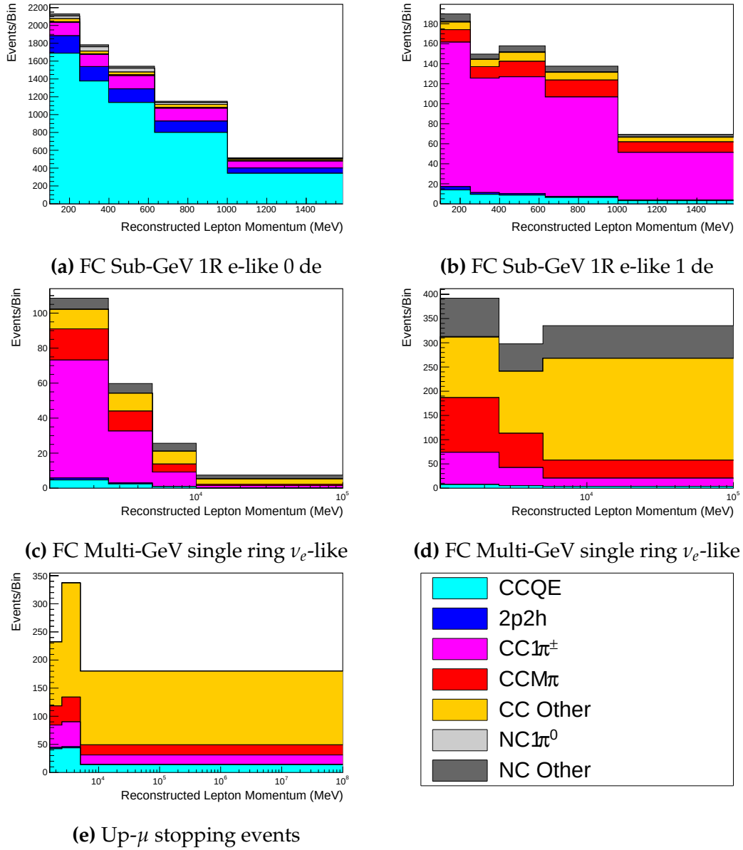
Figure 6.3: Breakdown by interaction mode of some representative atmospheric samples used within this analysis, illustrated as a function of reconstructed lepton momentum. The binning is provided in Table 6.5. Asimov A oscillation parameters are used to generate these plots. The interaction mode breakdown of all atmospheric samples used within this analysis can be found in [183].
