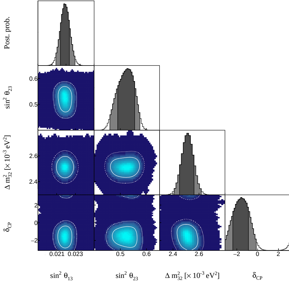
Figure 8.30: The posterior probability density distribution from the joint beam-atmospheric fit where the reactor constraint is applied. The distribution is given for each two-dimensional permutation of the oscillation parameters of interest where the solid(dashed) white lines represent the 1\sigma(2\sigma) contours. The one-dimensional distribution of each parameter is also given, where the dark(light) grey region represents the 1\sigma(2\sigma) credible intervals.
