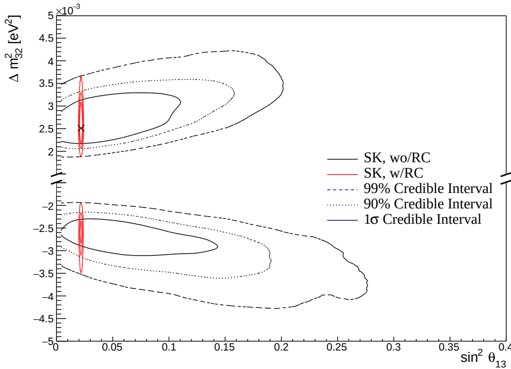
Figure 8.14: The two-dimensional posterior probability density distribution in \Delta m_{32}^2 - \sin^2(\theta_{13}) compared between the SK atmospheric-only fit (Black) and the SK atmospheric fit with the reactor constraint (Red). The distributions are marginalised over both hierarchies. The marker represents the known value of \Delta m_{32}^2 - \sin^2(\theta_{13}) .
