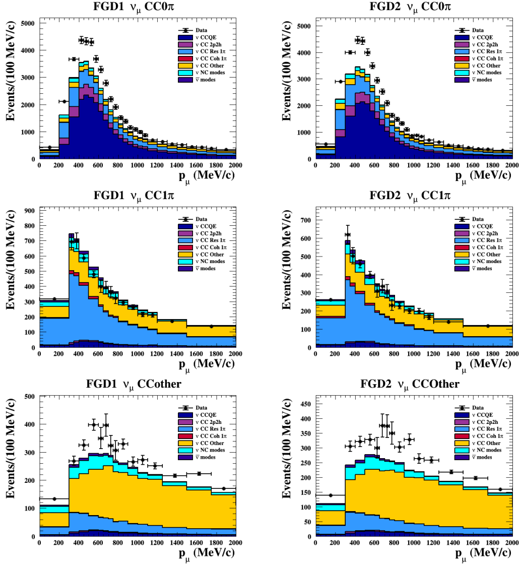
Figure 6.4: The nominal Monte Carlo predictions compared to data for the FGD1 and FGD2 samples in neutrino beam mode, broken down into the CC\nu_\mu 0\pi , CC\nu_\mu 1\pi and CC\nu_\mu Other categories. Figures taken from [184].
