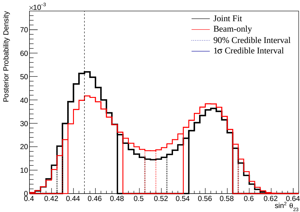
Figure 8.42: The one-dimensional posterior probability density distribution in \sin^2(\theta_{23}) compared between the joint beam-atmospheric fit (Black) and the latest T2K sensitivities (Red) [2, 212]. The reactor constraint is not applied in either fit. The distributions are marginalised over both hierarchies. The vertical dashed line represents the known value of \sin^2(\theta_{23}) .
