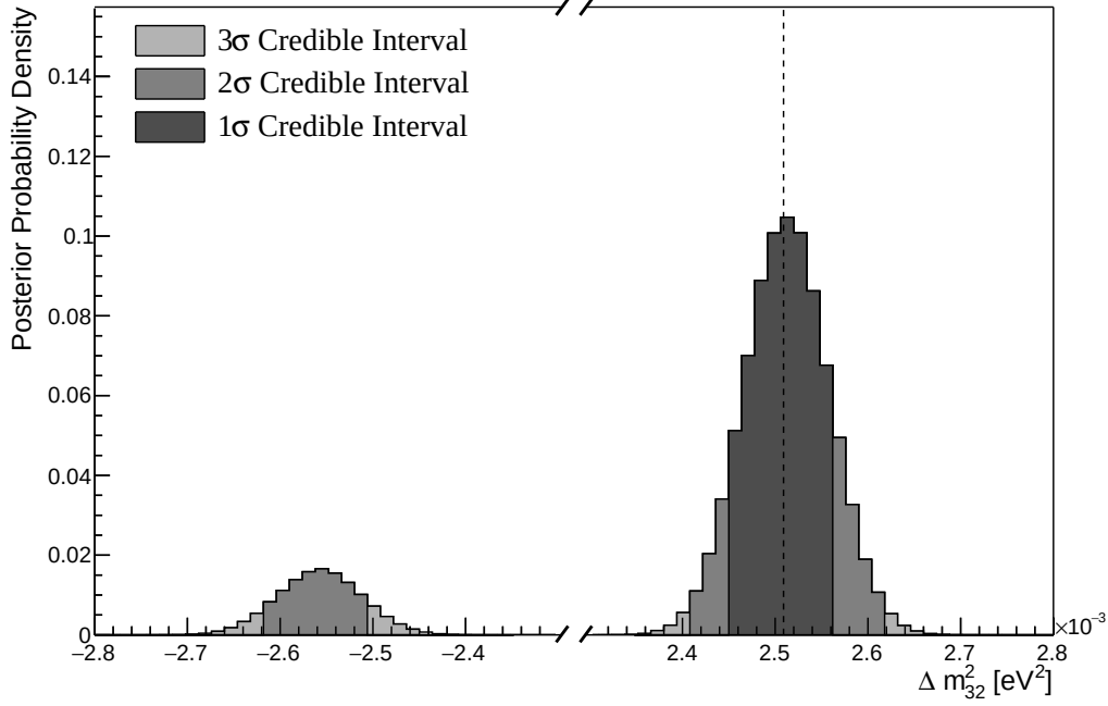
Figure 8.27: The one-dimensional posterior probability density distribution in \Delta m_{32}^2 from the joint beam-atmospheric fit where the reactor constraint is applied. The vertical dashed line represents the known value of \Delta m_{32}^2 .
