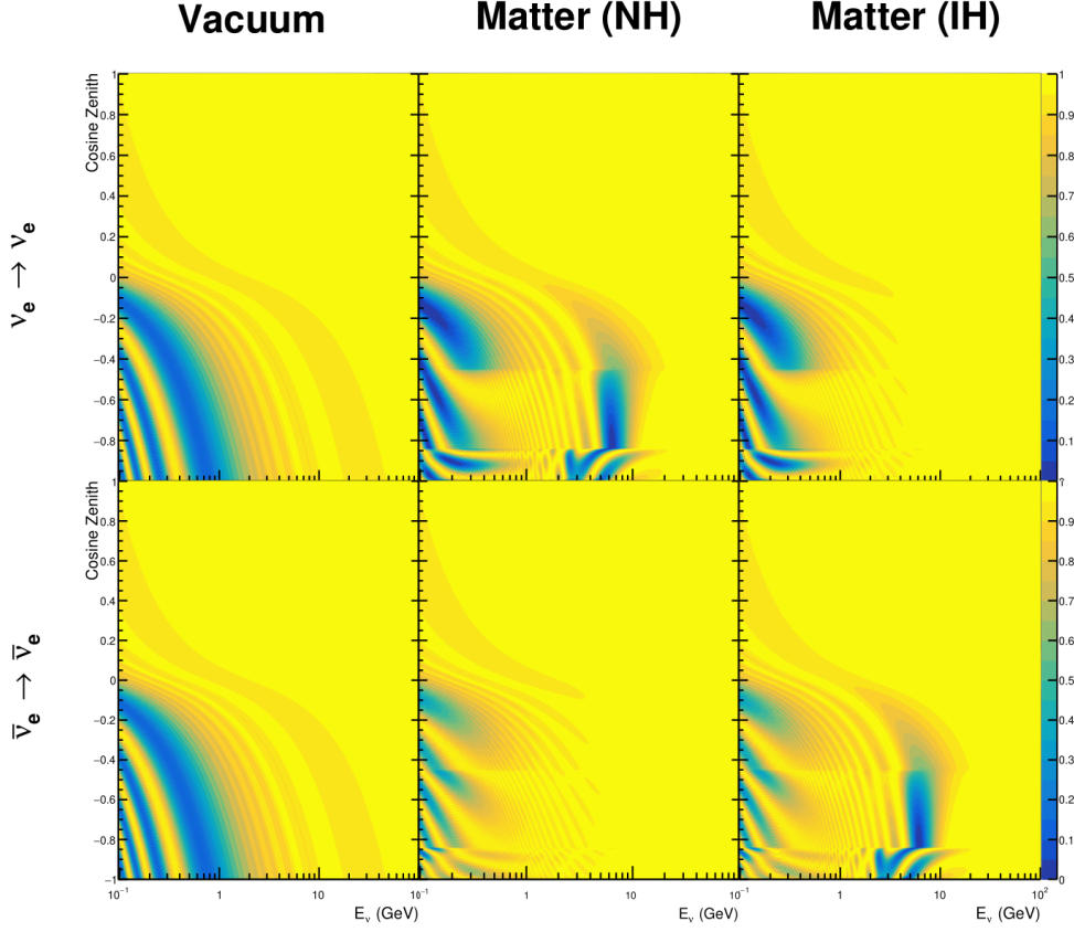
Figure 2.11: An illustration of the matter-induced effects on the oscillation probability, given as a function of neutrino energy and zenith angle. The top row of panels gives the P(\nu_e \rightarrow \nu_e) oscillation probability and the bottom row illustrates the P(\bar{\nu}_e \rightarrow \bar{\nu}_e) oscillation probability. The left column highlights the oscillation probability in a vacuum, whereas the middle and right column represents the oscillation probabilities when the four-layer fixed density PREM model is assumed. All oscillation probabilities assume the “Asimov A” set given in Table 2.2, but importantly, the right column sets an inverted mass hierarchy. The “matter resonance” effects at E_\nu \sim 5\text{GeV} can be seen in the P(\nu_e \rightarrow \nu_e) for normal mass hierarchy and P(\bar{\nu}_e \rightarrow \bar{\nu}_e) for inverted hierarchy.
