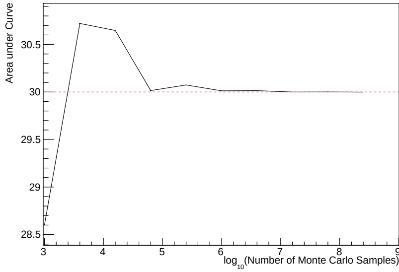
Figure 4.2: The area under a line of gradient 0.4 and intercept 1.0 for the range 0 \leq x \leq 10 as calculated using Monte Carlo techniques as a function of the number of samples used in each repetition. The analytical solution to the area is 30 units as given by the red line.
