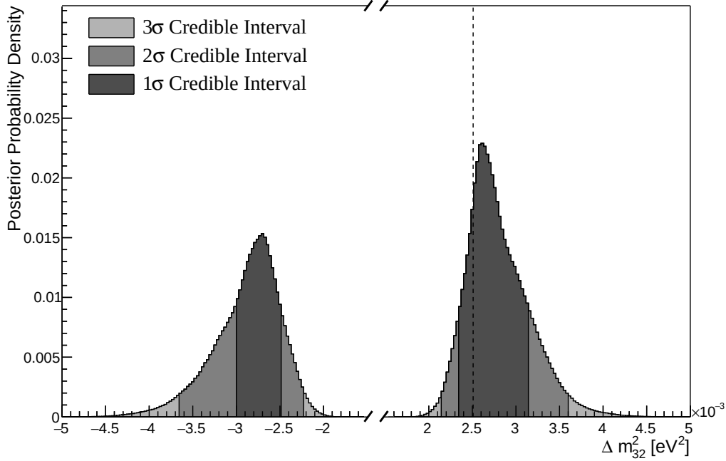
Figure 8.8: The one-dimensional posterior probability density distribution in \Delta m_{32}^2 , marginalised over both hierarchies, from the SK atmospheric-only fit. The reactor constraint is not applied. The vertical dashed line represents the known value of \Delta m_{32}^2 .
