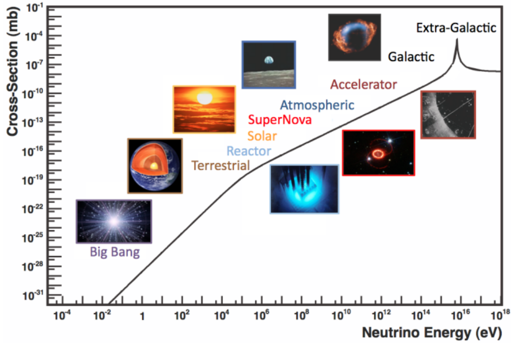
Figure 2.1: The electro-weak cross-section for \bar{\nu}_e + e^- \rightarrow \bar{\nu}_e + e^- scattering on free electrons from various natural and man-made neutrino sources, as a function of neutrino energy. Taken from [29].
