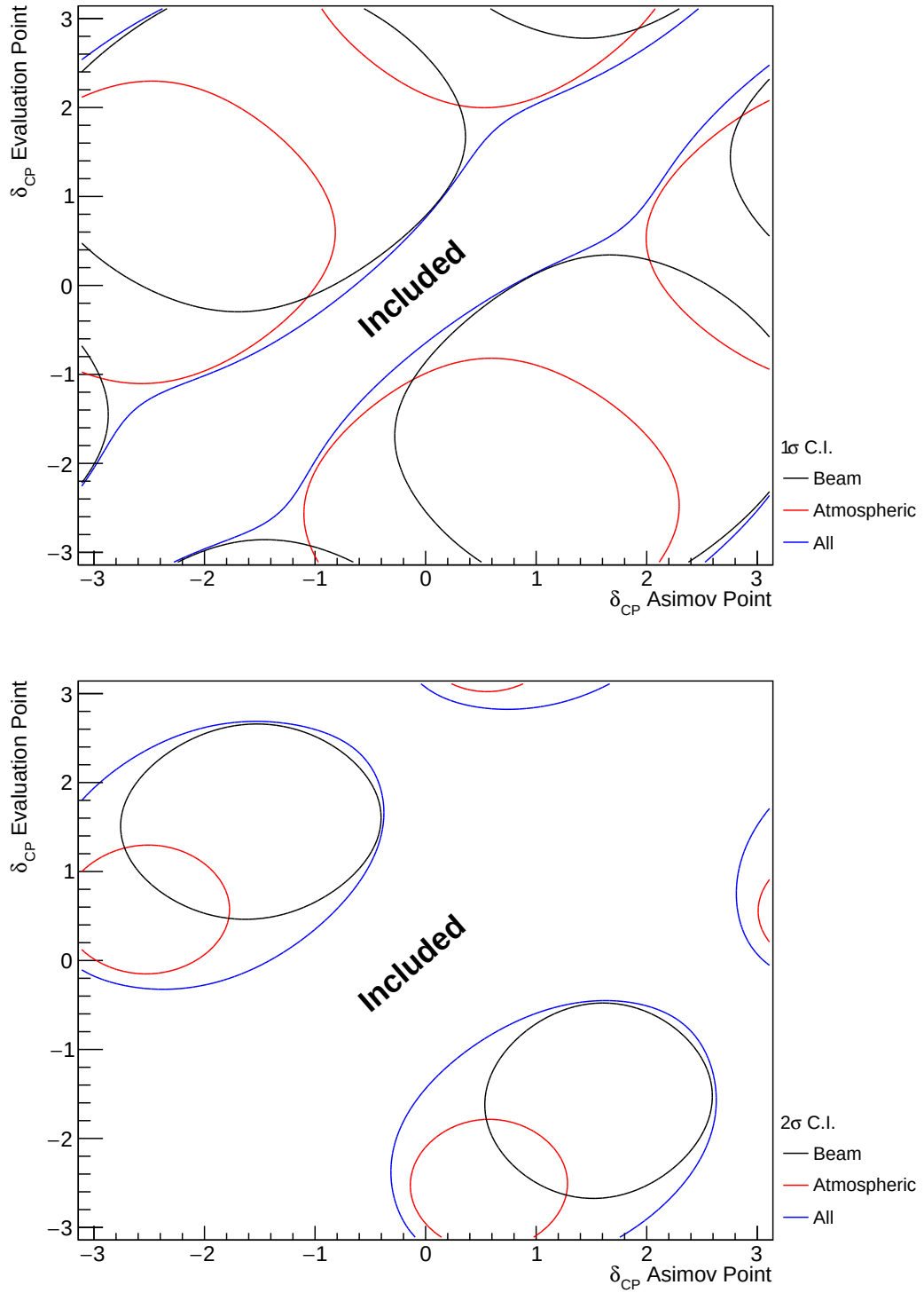
Figure 8.4: A series of one-dimensional likelihood scans over \delta_{CP} , where an Asimov data set is built for each value of \delta_{CP} on the x-axis and the likelihood is evaluated for each value of \delta_{CP} on the y-axis. The diagonal represents the minimum log-likelihood and defines the region included within the 1 \sigma (Top) and 2 \sigma (Bottom) confidence intervals. The beam (black) and atmospheric (red) samples are individually plotted and the joint fit (blue) is the sum of the two.
