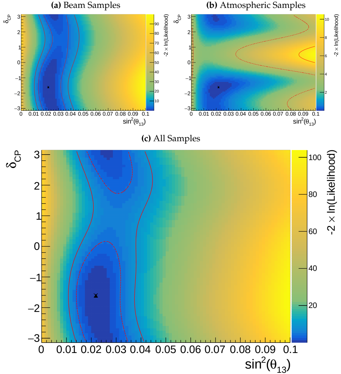
Figure 8.2: Two-dimensional log-likelihood scan of the appearance ( \sin^2(\theta_{13}) – \delta_{CP} ) parameters showing the response of the beam samples (top left), atmospheric samples (top right) and the summed response (bottom). The Asimov A oscillation parameters, defined in Table 2.2, are known to be the true point (Black Cross). The position of the smallest log-likelihood is highlighted with the triangle. Prior uncertainty terms of the oscillation parameters are neglected. The two(three) sigma contour levels are illustrated with the dashed(solid) red line.
