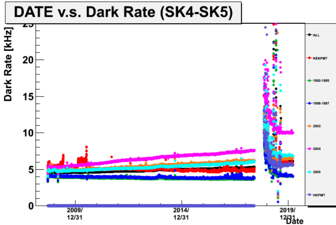
Figure 5.6: The variation of the measured dark rate as a function of date, broken down by PMT type. The SK-IV and SK-V periods span September 2008 to May 2018 and January 2019 to July 2020, respectively. The break in measurement in 2018 corresponds to the period of tank repair and refurbishment. Figure adapted from [176].
