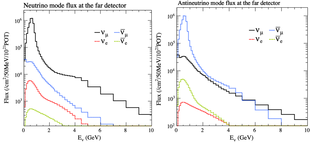
Figure 3.6: The Monte Carlo prediction of the energy spectrum for each flavour of neutrino ( \nu_e , \bar{\nu}_e , \nu_\mu and \bar{\nu}_\mu ) in the neutrino dominated beam FHC mode (Left) and antineutrino dominated beam RHC mode (Right) expected at SK. Taken from [78].
