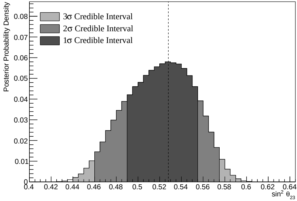
Figure 8.25: The one-dimensional posterior probability density distribution in \sin^2(\theta_{23}) , marginalised over both hierarchies, from the joint beam-atmospheric fit where the reactor constraint is applied. The vertical dashed line represents the known value.
