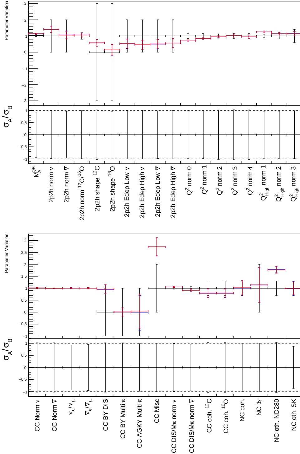
Figure 8.45: Central values and 1\sigma uncertainties for a select group of interaction systematics. The constraints from the prior uncertainty (Black), joint atmospheric-beam fit given in subsection 8.3.4 (Red) and beam-only analysis [2, 212] (Blue) are presented. The top part of each plot presents the parameter variation and the bottom part represents the ratio of the uncertainty between the joint beam-atmospheric and beam-only fits, where a value below 1.0 means the joint fit has a tighter constraint than the beam-only analysis.
