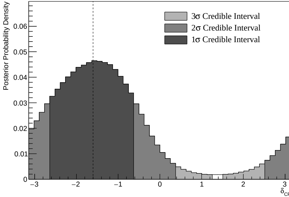
Figure 8.16: The one-dimensional posterior probability density distribution in \delta_{CP} , marginalised over both hierarchies, from the joint beam-atmospheric fit. The reactor constraint is not applied. The vertical dashed line represents the known value of \delta_{CP} .
