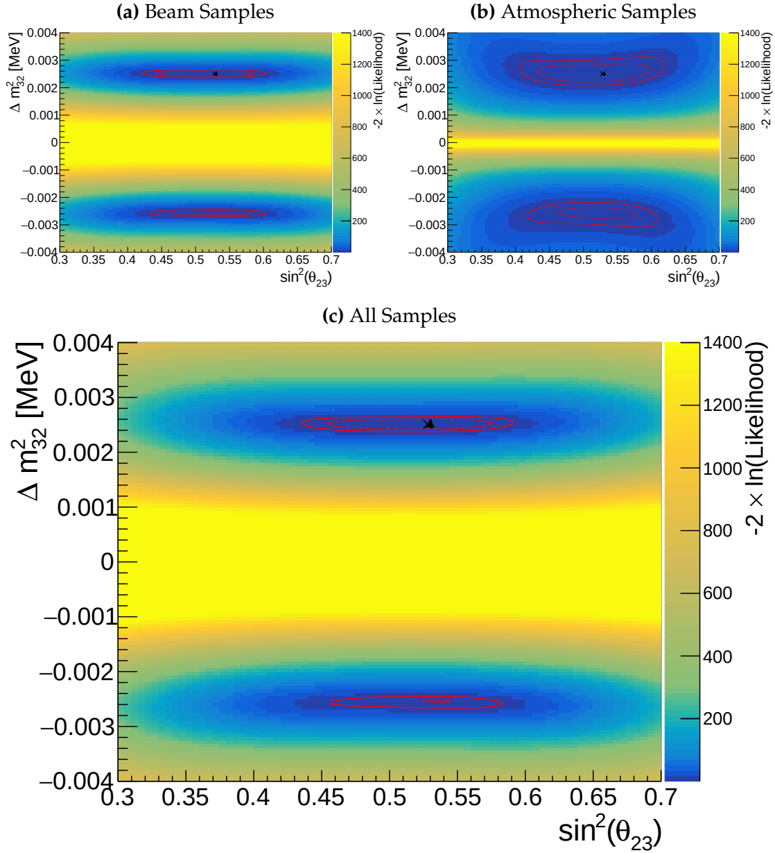
Figure 8.3: Two-dimensional log-likelihood scan of the disappearance ( \sin^2(\theta_{23}) - \Delta m_{32}^2 ) parameters showing the response of the beam samples (top left), atmospheric samples (top right) and the summed response (bottom). The Asimov A oscillation parameters, defined in Table 2.2, are known to be the true point (Black Cross). The position of the smallest log-likelihood is highlighted with the triangle. Prior uncertainty terms of the oscillation parameters are neglected. The two(three) sigma contour levels are illustrated with the dashed(solid) red line.
