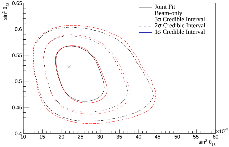
Figure 8.38: The posterior probability density distribution in \sin^2(\theta_{23}) - \sin^2(\theta_{13}) compared between the joint beam-atmospheric fit (Black) and the latest T2K sensitivities (Red) [2, 212]. The reactor constraint is not applied in either fit. The distributions are marginalised over both hierarchies. The marker represents the known value.
