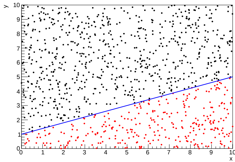
Figure 4.1: Example of using Monte Carlo techniques to find the area under the blue line. The gradient and intercept of the line are 0.4 and 1.0 respectively. The area found to be under the curve using one thousand samples is 29.9 units.
