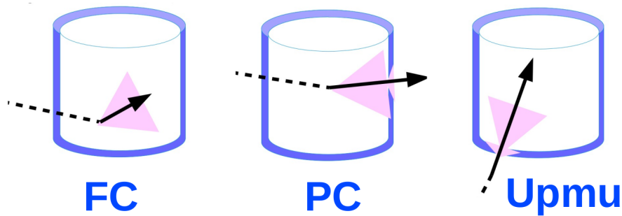
Figure 5.10: A depiction of the topology patterns for fully-contained (FC), partially-contained (PC), and up-going muon (Up- \mu ) samples included in this analysis.
