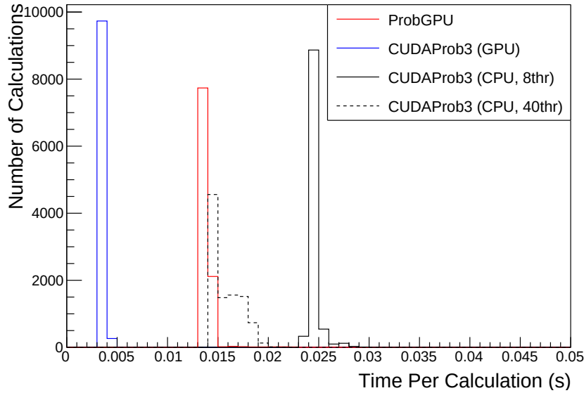
Figure 7.9: The calculation time taken to both calculate the oscillation probabilities and fill the “coarse” oscillograms, following the technique given in section 7.1, for the CUDAProb3 and ProbGPU (Red) calculation engines. CUDAProb3 has both a GPU (Blue) and CPU (Black) implementation, where the CPU implementation is multi-threaded. Therefore, 8-threads (solid) and 40-threads (dashed) configurations have been tested. Prob3, which is a CPU single-thread implementation has a mean step time of 1.142s.
