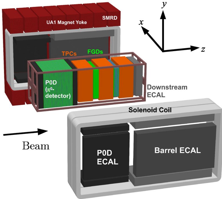
Figure 3.8: The components of the ND280 detector. The neutrino beam travels from left to right. Taken from [42].
