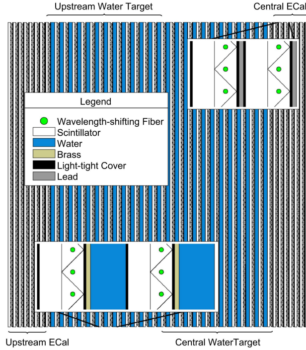
Figure 3.12: A schematic of the P0D side-view. Taken from [114].
