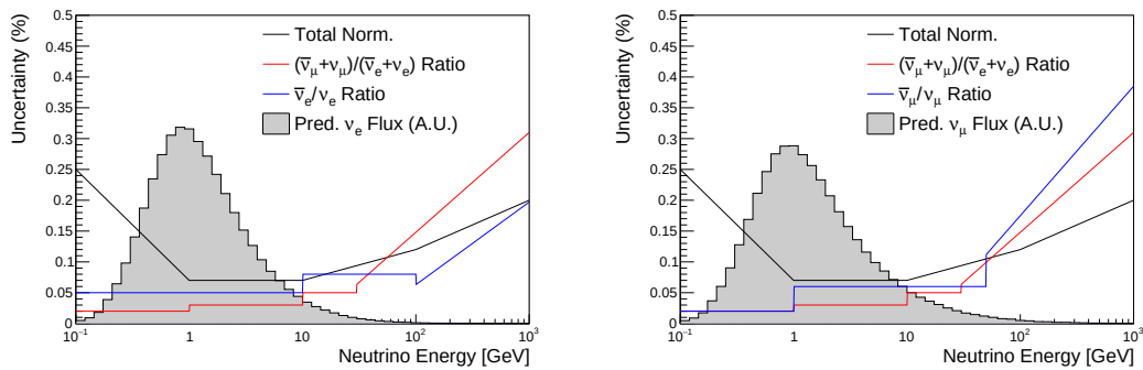
Figure 6.8: The uncertainty evaluated on the atmospheric \nu_e (left) and \nu_\mu (right) flux predictions. The absolute normalisation and flavour ratio uncertainties are given. The solid histogram indicates the neutrino flux as a function of energy.
