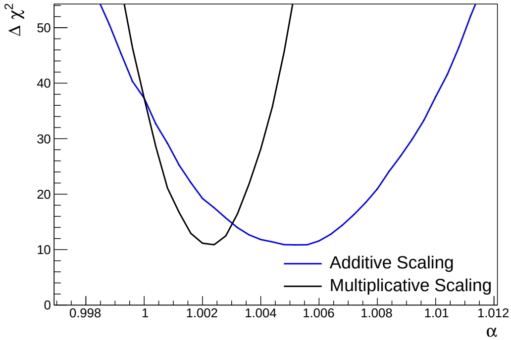
Figure 5.9: The \chi^2 difference between the SK-IV and SK-V reconstructed muon momentum divided by range when the SK-V is modified by the scaling parameter \alpha . Both additive (Blue) and multiplicative (Black) scaling factors have been considered. In practice, the additive scaling factor actually uses the value of (\alpha - 1.0) but is illustrated like this so the results can be shown on the same axis range.
