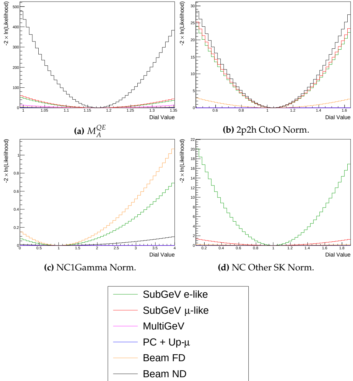
Figure 8.6: The response of the likelihood, as defined in section 8.2, illustrating the response of the samples to the various cross-section systematic parameters.
