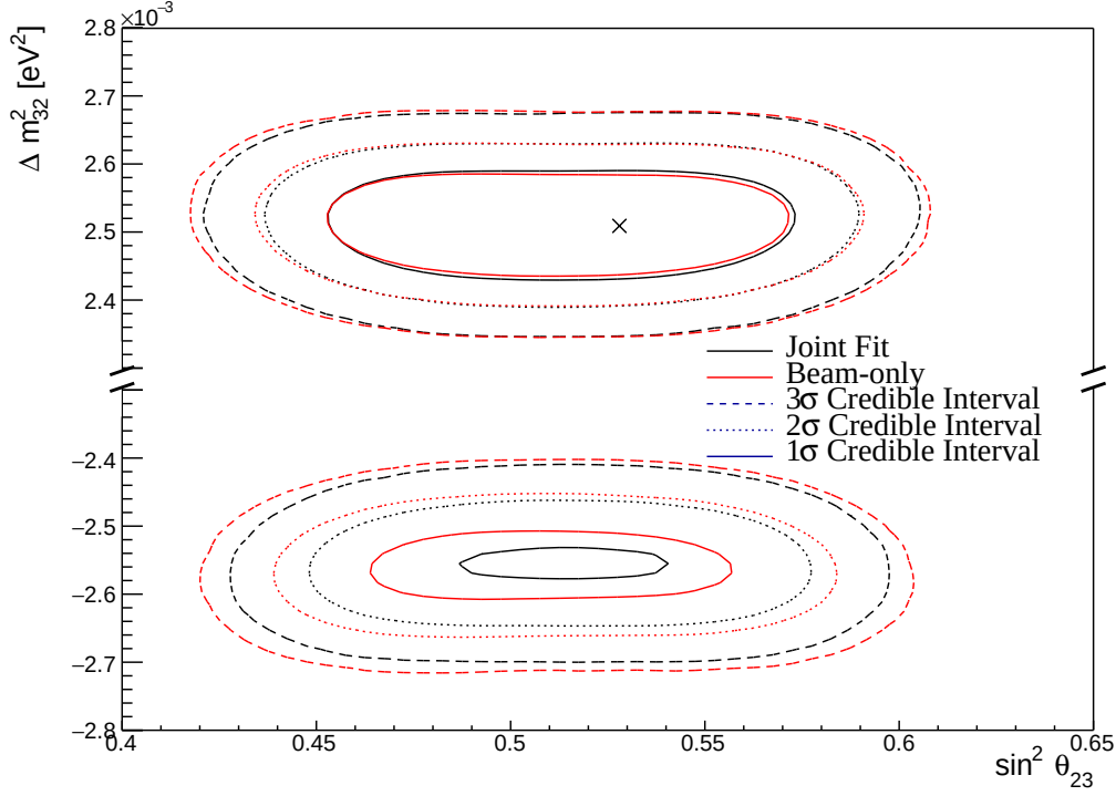
Figure 8.35: The two-dimensional posterior probability density distribution in \Delta m_{32}^2 - \sin^2(\theta_{23}) compared between the joint beam-atmospheric fit (Black) and the latest T2K sensitivities (Red) [2, 212]. The reactor constraint is not applied in either fit. The marker represents the known value of \Delta m_{32}^2 - \sin^2(\theta_{23}) .
