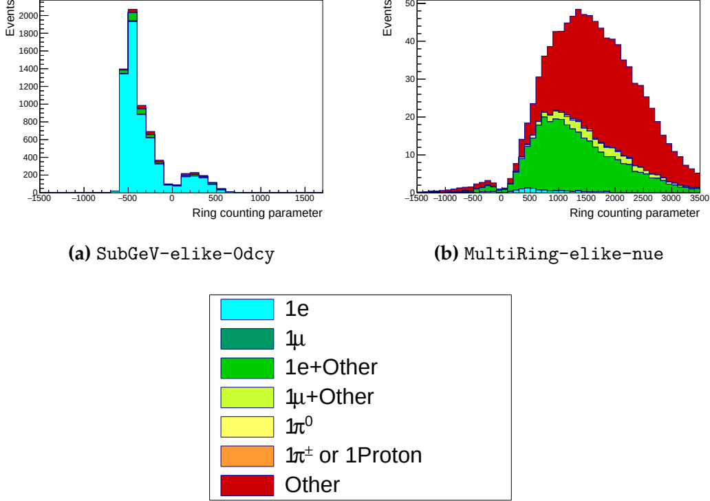
Figure 6.13: The ring counting parameter as defined in Equation 6.6 for the SubGeV-elastic-0dcy and MultiRing-elastic-nue samples.
