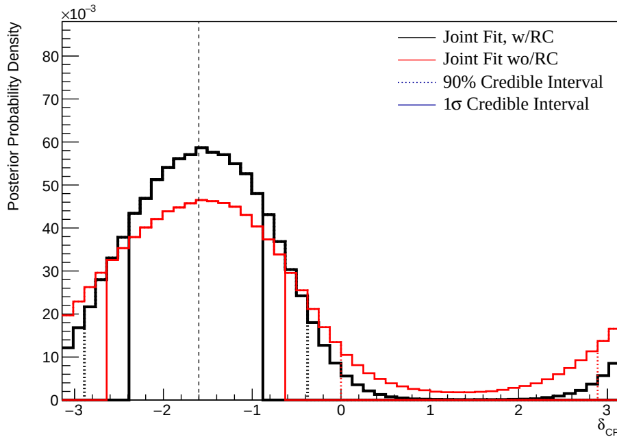
Figure 8.24: The one-dimensional posterior probability density distribution in \delta_{CP} compared between the joint beam-atmospheric fit (Red) and the joint beam-atmospheric fit with the reactor constraint (Black). The distributions are marginalised over both hierarchies. The vertical dashed line represents the known value.
