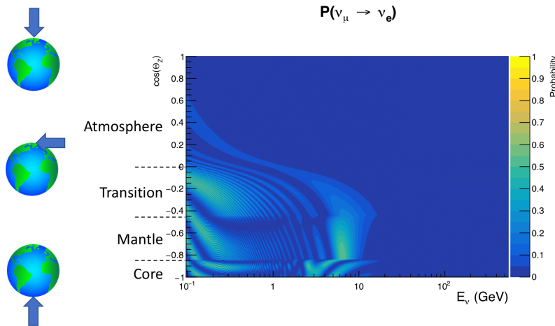
Figure 2.9: An “oscillogram” that depicts the P(\nu_\mu \rightarrow \nu_e) oscillation probability as a function of neutrino energy and cosine of the zenith angle. The zenith angle is defined such that \cos(\theta_Z) = 1.0 represents neutrinos that travel from directly above the detector. The four-layer constant density PREM model approximation is used and Asimov A oscillation parameters are assumed (Table 2.2).
