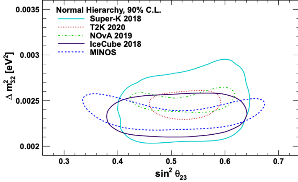
Figure 2.6: Constraints on the atmospheric oscillation parameters, \sin^2(\theta_{23}) and \Delta m_{32}^2 , from atmospheric and long-baseline experiments: SK [59], T2K [60], NOvA [61], IceCube [62] and MINOS [63]. Figure taken from [64].
