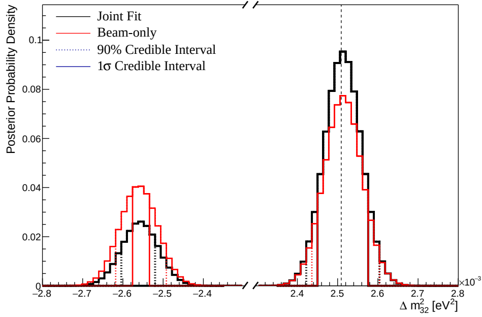
Figure 8.32: The one-dimensional posterior probability density distribution in \Delta m_{32}^2 compared between the joint beam-atmospheric fit (Black) and the latest T2K sensitivities (Red) [2, 212]. The reactor constraint is not applied in either fit. The vertical dashed line represents the known value.
