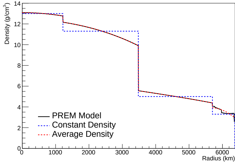
Figure 7.11: The density of the Earth given as a function of the radius, as given by the PREM model (Black), the constant density four-layer approximation (Blue), as used in the official SK-only analysis, and the quadratic approximation of the PREM model (Red).
