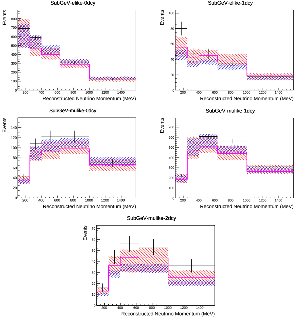
Figure 6.11: Down-going atmospheric subGeV single-ring samples comparing the mean and error of the pre-fit and post-fit Monte Carlo predictions in red and blue, respectively. The magenta histogram illustrates the Monte Carlo prediction using the generated dial values. The black points illustrate the down-going data with statistical errors given. The mean and errors of the Monte Carlo predictions are calculated by the techniques documented in subsection 4.3.4. The pre-fit spectrum is calculated by throwing the cross-section and atmospheric flux dial values from the pre-fit covariance matrix. The post-fit spectrum is calculated by sampling the cross-section dial values from an ND fit MCMC chain, whilst still throwing the atmospheric flux dials from the pre-fit covariance.
