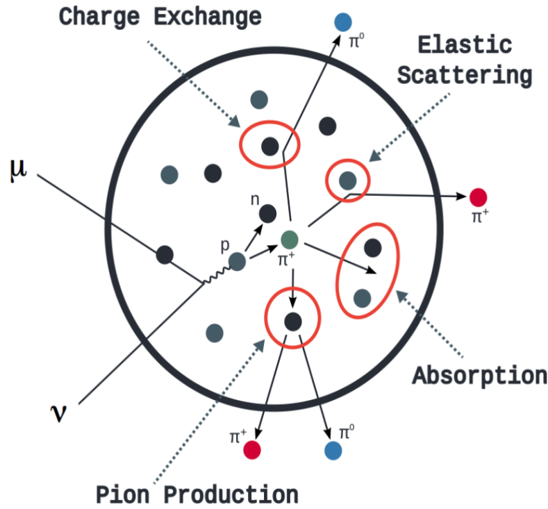
Figure 5.2: Illustration of the various processes which a pion can undergo before exiting the nucleus. Taken from [163].
