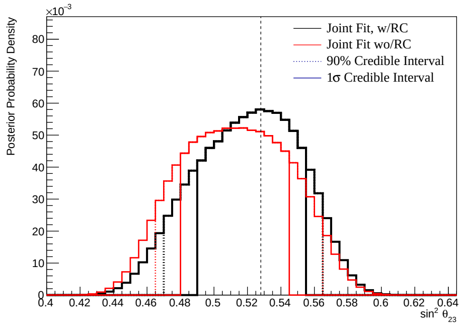
Figure 8.26: The one-dimensional posterior probability density distribution in \sin^2(\theta_{23}) compared between the joint beam-atmospheric fit (Red) and the joint beam-atmospheric fit with the reactor constraint (Black). The distributions are marginalised over both hierarchies. The vertical dashed line represents the known value.
