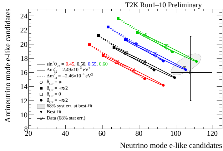
Figure 2.13: The number of electron-like events in the FHC and RHC operating mode of the beam, as a function of the oscillation probabilities. Both normal hierarchy (Solid)) and inverse hierarchy (Dashed) values of \Delta m_{32}^2 are given.
