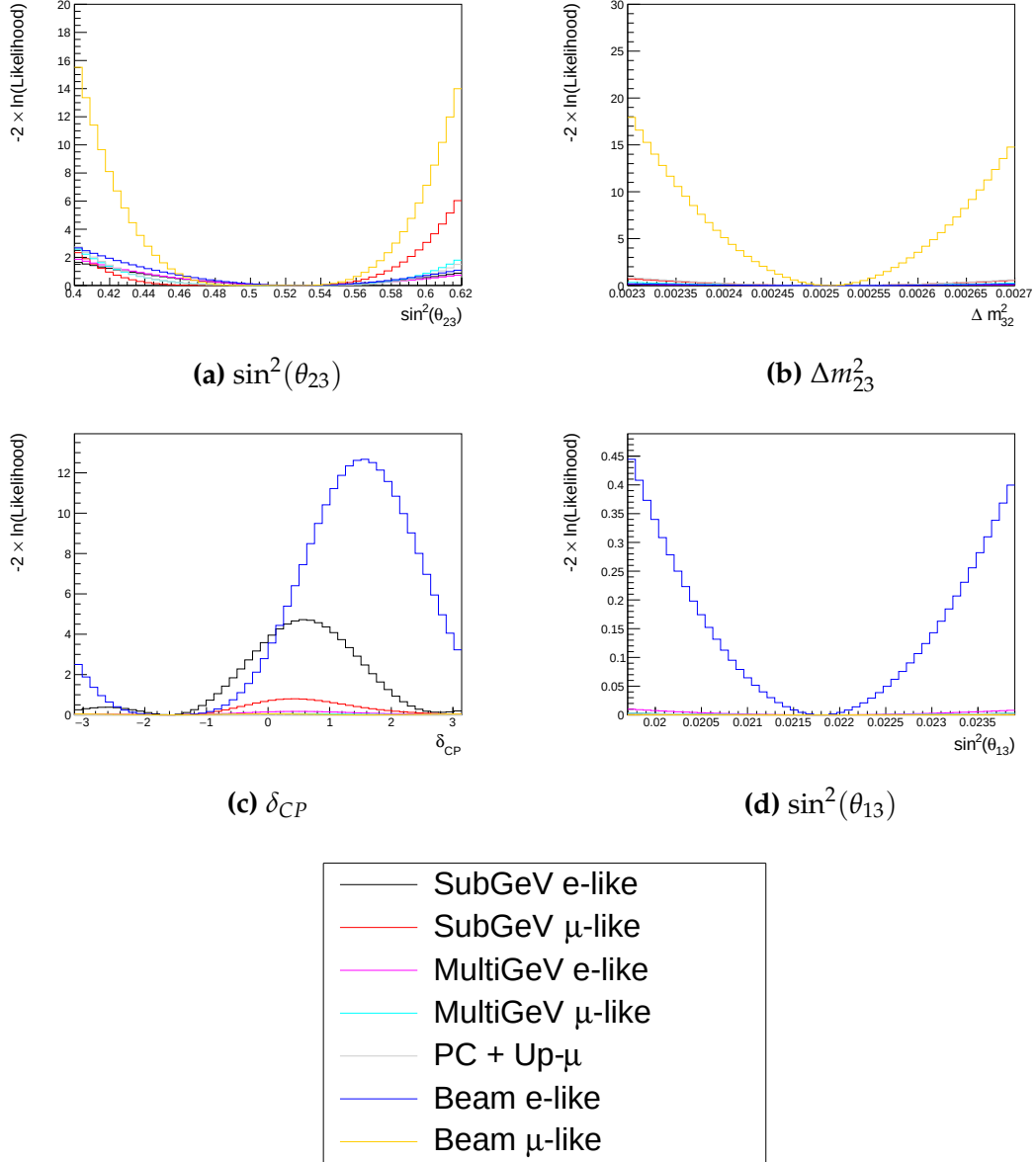
Figure 8.1: The response of the likelihood, as defined in section 6.5, illustrating the response of the samples to a variation of an oscillation parameter.
