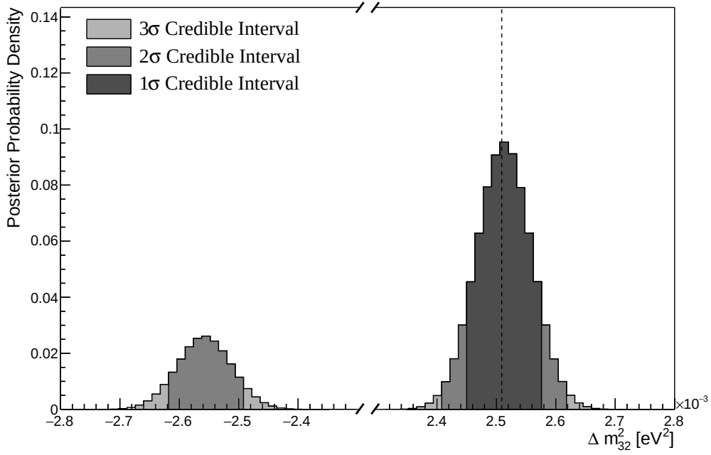
Figure 8.17: The one-dimensional posterior probability density distribution in \Delta m_{32}^2 , marginalised over both hierarchies, from the joint beam-atmospheric fit. The reactor constraint is not applied. The vertical dashed line represents the known value of \Delta m_{32}^2 .
