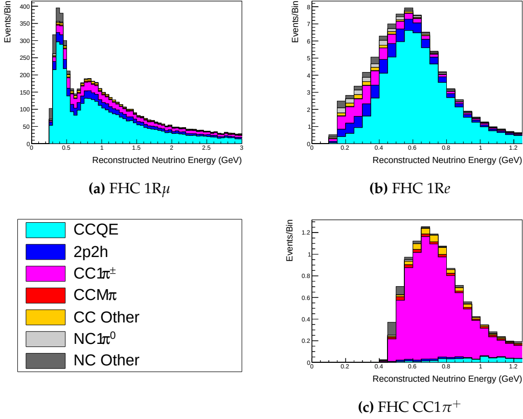
Figure 6.5: The reconstructed neutrino energy, as defined by Equation 6.2 and Equation 6.3, for the 1R \mu -like, 1Re-like, and CC1 \pi^+ -like samples. The AsimovA oscillation parameters are assumed (given in Table 2.2). These samples are the FHC mode samples. For ease of viewing, the 1R \mu sample only shows the 0. \leq E_\nu^{rec} < 3.0\text{GeV} but the binning extends to 30.0GeV.
