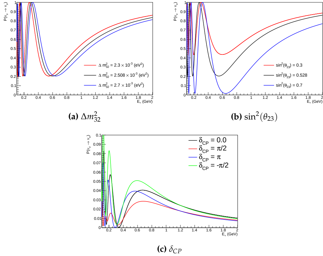
Figure 2.12: The oscillation probability for beam neutrino events given as a function of neutrino energy. All oscillation parameters assume the “Asimov A” set given in Table 2.2 unless otherwise stated. A path-length of 295km is assumed. Each panel represents a change in one of the oscillation parameters whilst keeping the remaining parameters fixed.
