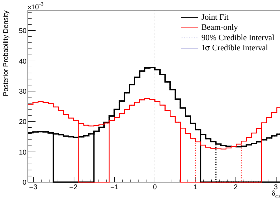
Figure 8.41: The one-dimensional posterior probability density distribution in \delta_{CP} compared between the joint beam-atmospheric fit (Black) and the latest T2K sensitivities (Red) [2, 212]. The reactor constraint is not applied in either fit. The distributions are marginalised over both hierarchies. The vertical dashed line represents the known value of \delta_{CP} .
