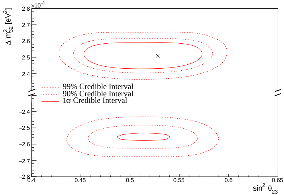
Figure 8.20: The two-dimensional posterior probability density distribution in \Delta m^2_{32}-\sin^2(\theta_{23}) , marginalised over both hierarchies, from the joint beam-atmospheric fit. The reactor constraint is not applied. The marker represents the input value.
