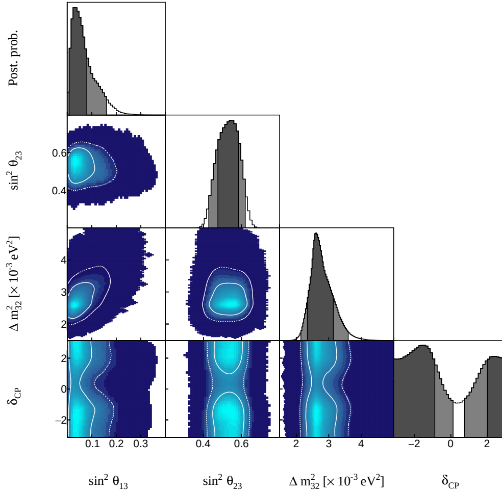
Figure 8.12: The posterior probability density distribution from the SK atmospheric-only fit. The reactor constraint is not applied. The distribution is given for each two-dimensional permutation of the oscillation parameters of interest where the solid(dashed) white lines represent the 1\sigma(2\sigma) contours. The one-dimensional distribution of each parameter is also given, where the dark(light) grey region represents the 1\sigma(2\sigma) credible intervals.
