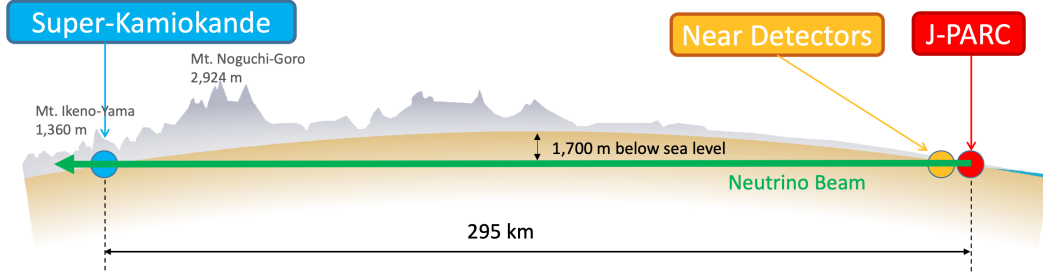
Figure 3.3: The cross-section view of the Tokai to Kamioka experiment illustrating the beam generation facility at J-PARC, the near detector situated at a baseline of 280m and the Super Kamiokande far detector situated 295km from the beam target.
