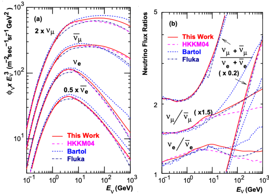
Figure 2.3: Left panel: The atmospheric neutrino flux for different neutrino flavours as a function of neutrino energy as predicted by the 2007 Honda model (“This work”) [50], the 2004 Honda model (“HKKM04”)[51], the Bartol model [49] and the FLUKA model [53]. Right panel: The ratio of the muon to electron neutrino flux as predicted by all the quoted models. Both figures taken from [50].
