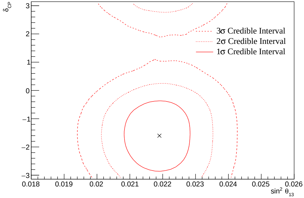
Figure 8.28: The two-dimensional posterior probability density distribution in \delta_{CP} - \sin^2(\theta_{13}) , marginalised over both hierarchies, from the joint beam-atmospheric fit where the reactor constraint is applied. The marker represents the known value.
