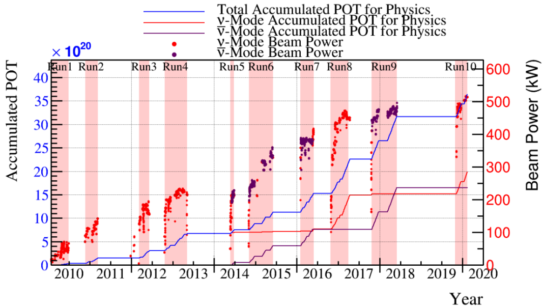
Figure 6.1: The accumulated beam data, measured as the number of protons on target (POT). The total data (blue) is given which comprises of the neutrino beam (red) and antineutrino (purple) components. The beam power for neutrino and antineutrino beams is given as the markers using the same colour scheme. The timescale runs from Run 1 which started in January 2010 until Run 10 which ended in February 2020. The ratio of accumulated data in neutrino and antineutrino beam is 54.7% : 45.3%.
