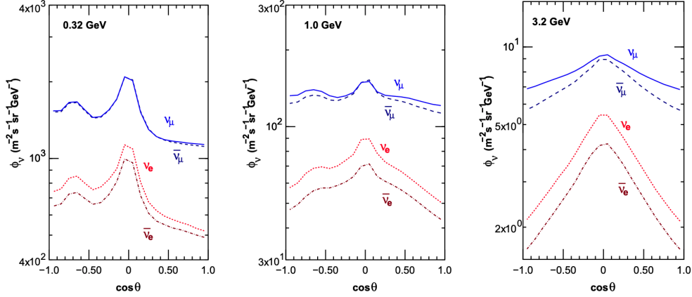
Figure 2.5: Prediction of \nu_e, \bar{\nu}_e, \nu_\mu, \bar{\nu}_\mu fluxes as a function of zenith angle as calculated by the HKKM model [52]. The left, middle and right panels represent three values of neutrino energy, 0.32 GeV, 1.0 GeV and 3.2 GeV respectively. Predictions for other models including Bartol [49], Honda [50] and FLUKA [53] are given in [54].
