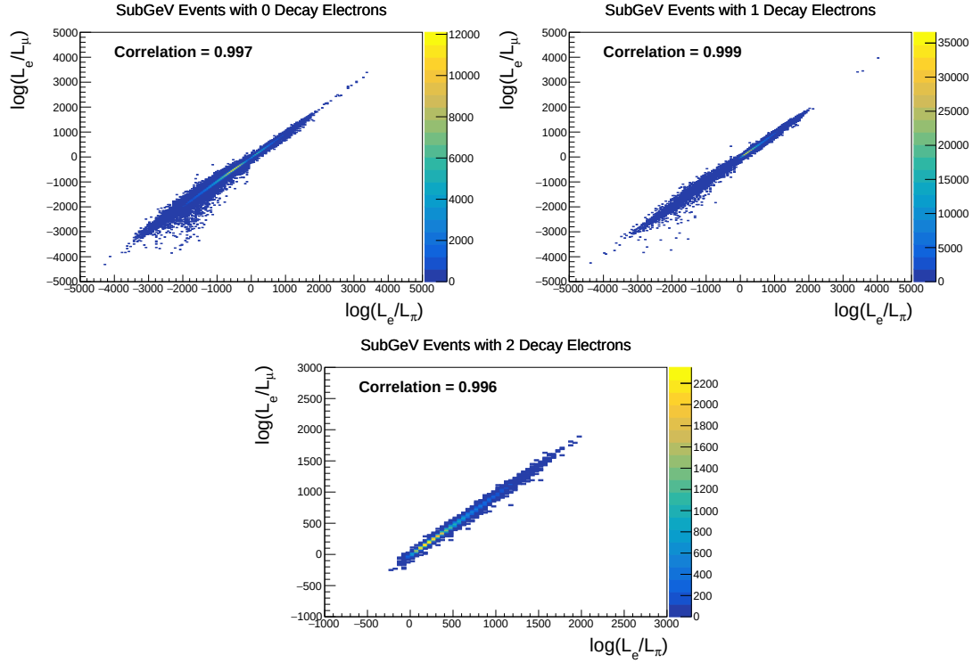
Figure 6.16: The distribution of \log(L_e/L_\mu) compared to \log(L_e/L_\pi) for subGeV events with zero (top left), one (top right) or two (bottom) decay electrons. The correlation in the distribution is calculated as 0.997, 0.999 and 0.996, respectively.
