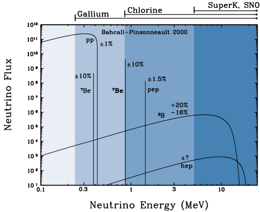
Figure 2.2: The solar neutrino flux as a function of neutrino energy for various fusion reactions and decay chains as predicted by the Standard Solar Model. Taken from [31].
