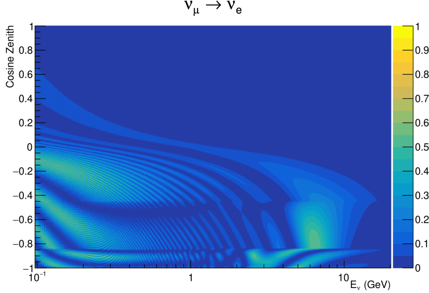
Figure 7.1: The oscillation probability P(\nu_\mu \rightarrow \nu_e) , given as a function of neutrino energy and zenith angle, which highlights an example of the “fast” oscillations in the sub-GeV upgoing region.
