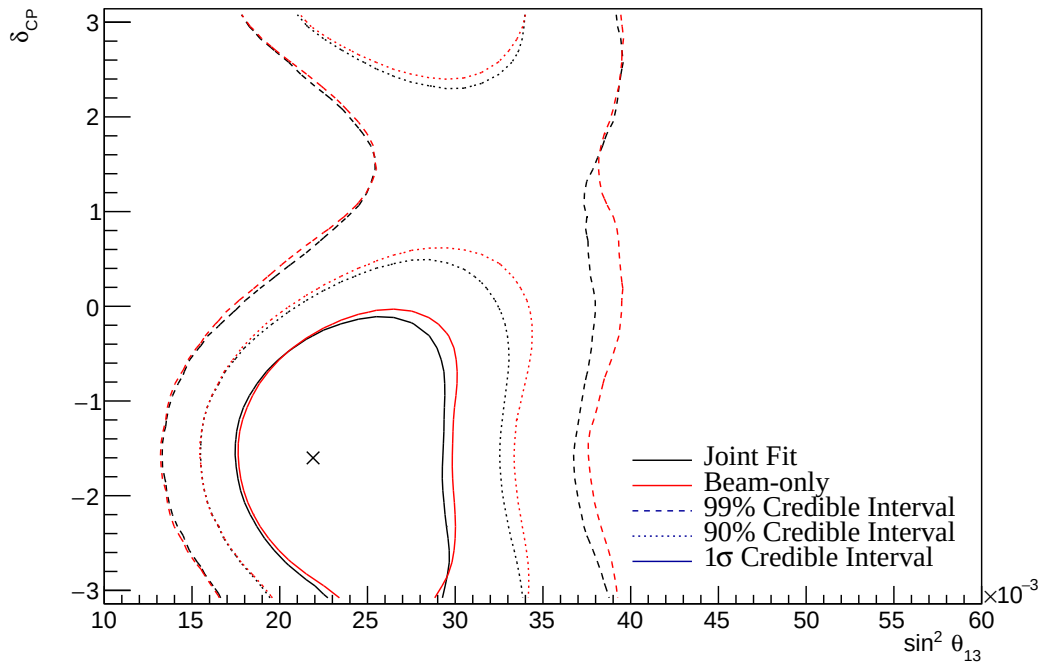
Figure 8.34: The two-dimensional posterior probability density distribution in \delta_{CP}-\sin^2(\theta_{13}) compared between the joint beam-atmospheric fit (Black) and the latest T2K sensitivities (Red) [2, 212]. The reactor constraint is not applied in either fit. The distributions are marginalised over both hierarchies. The marker represents the known value of \delta_{CP}-\sin^2(\theta_{13}) .
