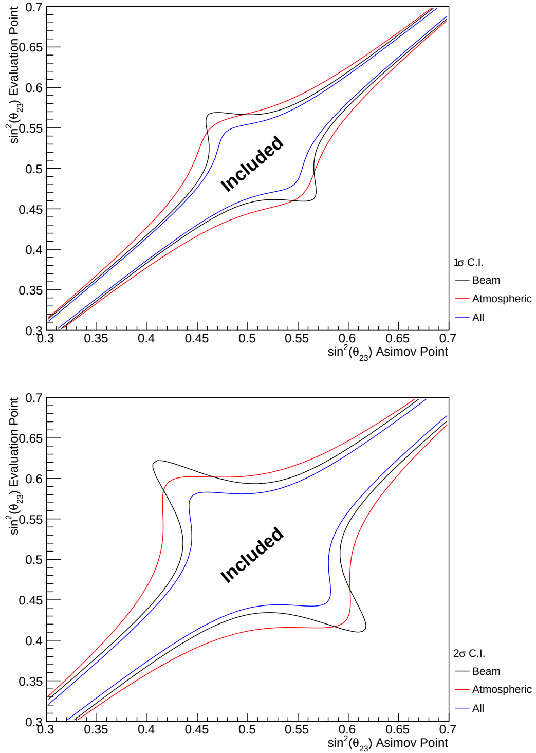
Figure 8.5: A series of one-dimensional likelihood scans over \sin^2(\theta_{23}) , where an Asimov data set is built for each value of \sin^2(\theta_{23}) on the x-axis and the likelihood is evaluated for each value of \sin^2(\theta_{23}) on the y-axis. The diagonal represents the minimum log-likelihood and defines the region included within the 1 \sigma (Top) and 2 \sigma (Bottom) confidence intervals. The beam (black) and atmospheric (red) samples are individually plotted and the joint fit (blue) is the sum of the two.
