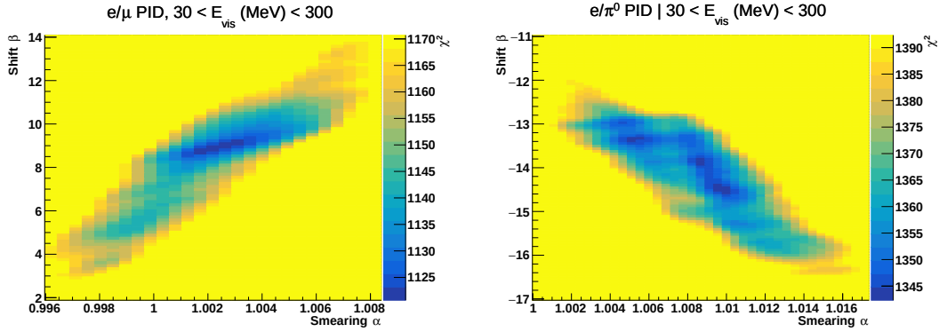
Figure 6.15: The \chi^2 between the hybrid- \pi^0 Monte Carlo and data samples, as a function of smear ( \alpha ) and shift ( \beta ) parameters, for events which have 1\pi^0 final state topology. Left: Electron-muon separation PID parameter for events with 30 \leq E_{vis} \text{ (MeV)} < 300 . Right: Electron- \pi^0 separation PID parameter for events with 30 \leq E_{vis} \text{ (MeV)} < 300 .
