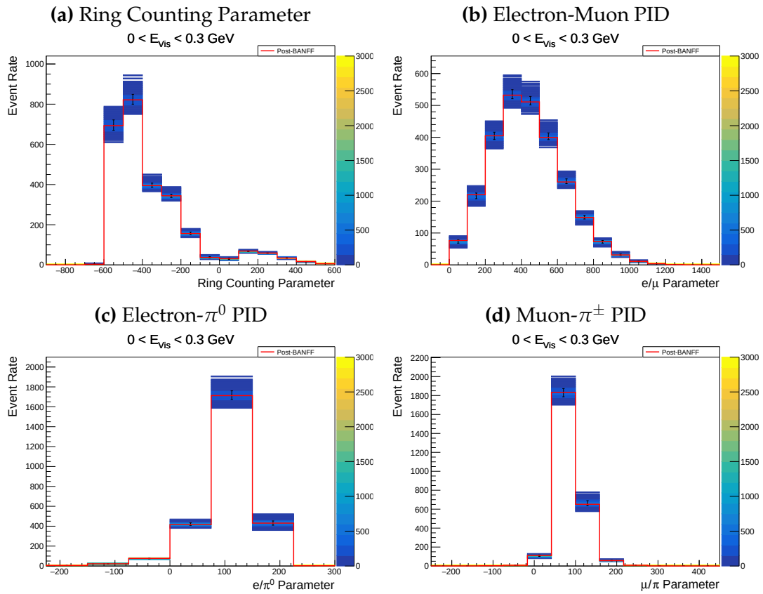
Figure 8.46: Result of the posterior predictive method for the SubGeV_e1ike_0dcy sample after sampling 2000 steps from the joint beam-atmospheric chain (Coloured histogram). It is presented in the four particle identification parameters listed in Table 6.7 for events with visible energy, 0 \leq E_{vis}(\text{MeV}) \leq 300 . The mean and uncertainty is presented for each bin using the highest posterior predictive method. The Asimov data prediction (denoted 'Post BANFF Spectra', Red) assumes the post-BANFF tune and Asimov A oscillation parameters.
