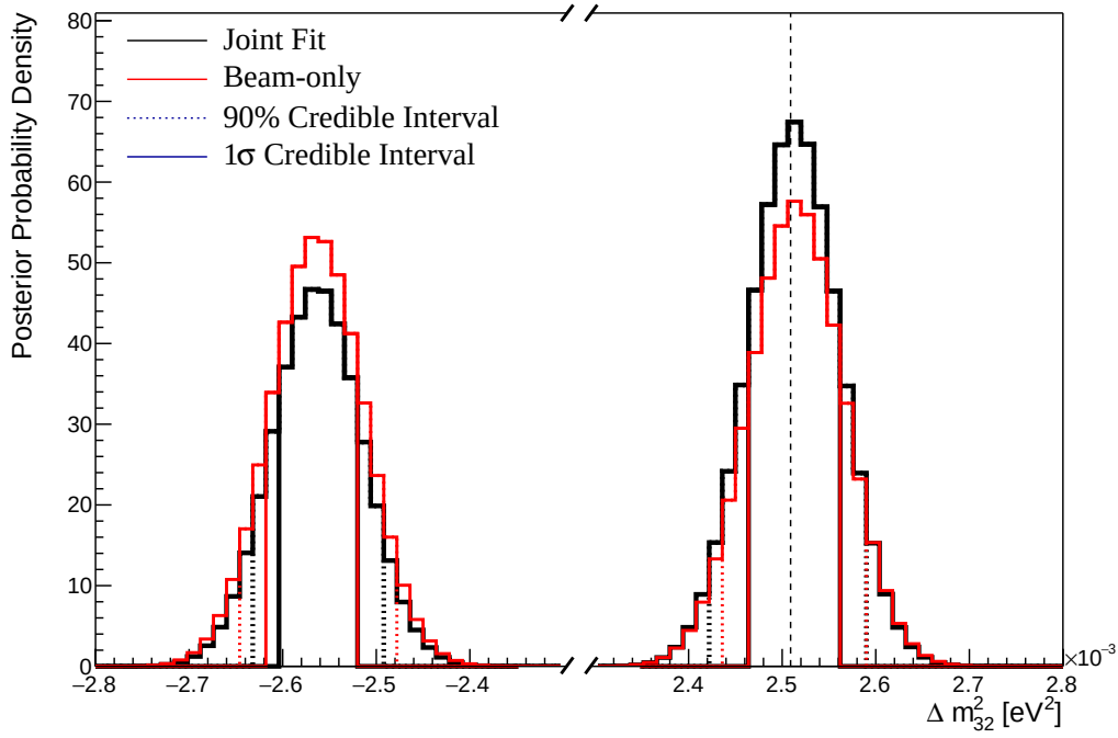
Figure 8.43: The one-dimensional posterior probability density distribution in \Delta m_{32}^2 compared between the joint beam-atmospheric fit (Black) and the latest T2K sensitivities (Red) [2, 212]. The reactor constraint is not applied in either fit. The vertical dashed line represents the known value of \Delta m_{32}^2 .
