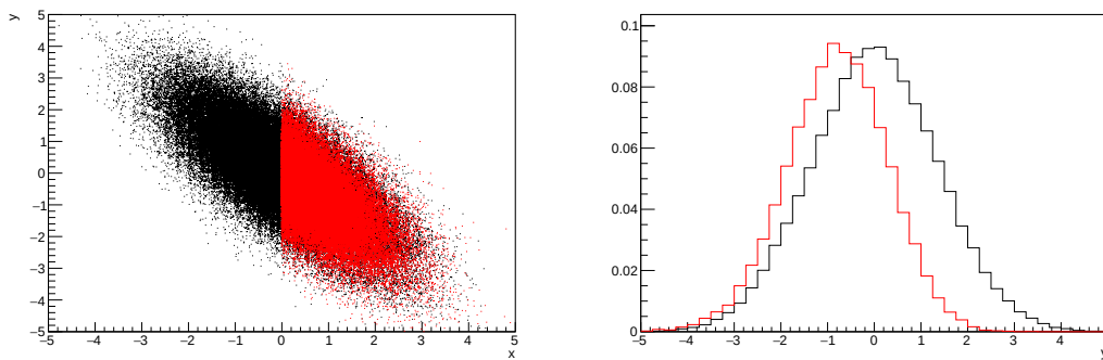
Figure 4.5: Left: The two-dimensional probability distribution for two correlated parameters x and y . The red distribution shows the two-dimensional probability distribution when 0 \leq x \leq 5 . Right: The marginalised probability distribution for the y parameter found when requiring the x to be bound between -5 \leq x \leq 5 and 0 \leq x \leq 5 for the black and red distribution, respectively.
