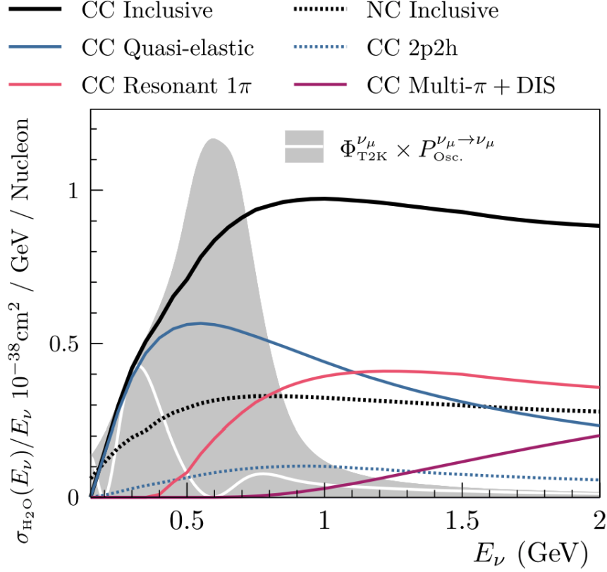
Figure 5.1: The NEUT prediction of the \nu_\mu -H 2 O cross-section overlaid on the T2K \nu_\mu flux. The charged current (black, solid) and neutral current (black, dashed) inclusive, charged current quasi-elastic (blue, solid), charged current 2p2h (blue, dashed), charged current single pion production (pink), and charged current multi- \pi and DIS (Purple) cross-sections are illustrated. Figure taken from [148].
