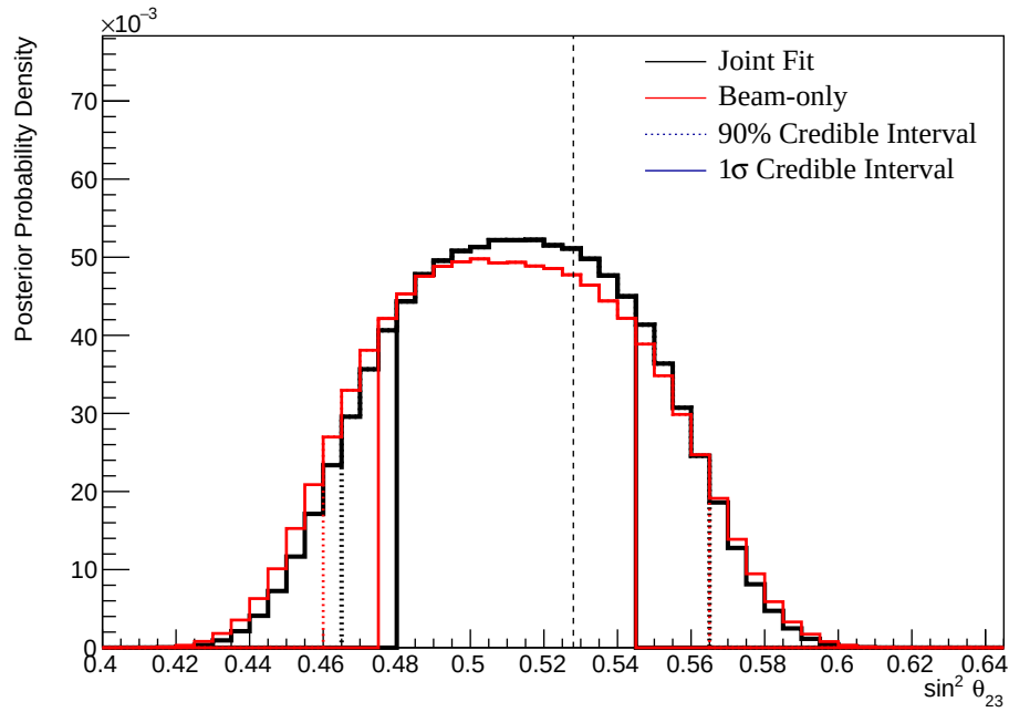
Figure 8.33: The one-dimensional posterior probability density distribution in \sin^2(\theta_{23}) compared between the joint beam-atmospheric fit (Black) and the latest T2K sensitivities (Red) [2, 212]. The reactor constraint is not applied in either fit. The distributions are marginalised over both hierarchies. The vertical dashed line represents the known value.
