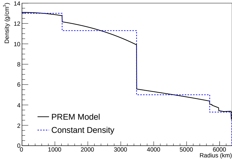
Figure 2.8: The density of the Earth given as a function of the radius, as provided by the PREM model (Black), and the constant density four-layer approximation (Blue), as used in the official SK-only analysis.
