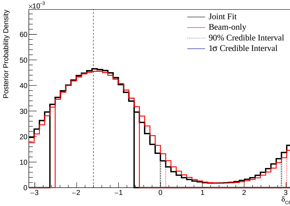
Figure 8.31: The one-dimensional posterior probability density distribution in \delta_{CP} compared between the joint beam-atmospheric fit (Black) and the latest T2K sensitivities (Red) [2, 212]. The reactor constraint is not applied in either fit. The distributions are marginalised over both hierarchies. The vertical dashed line represents the known value of \delta_{CP} .
