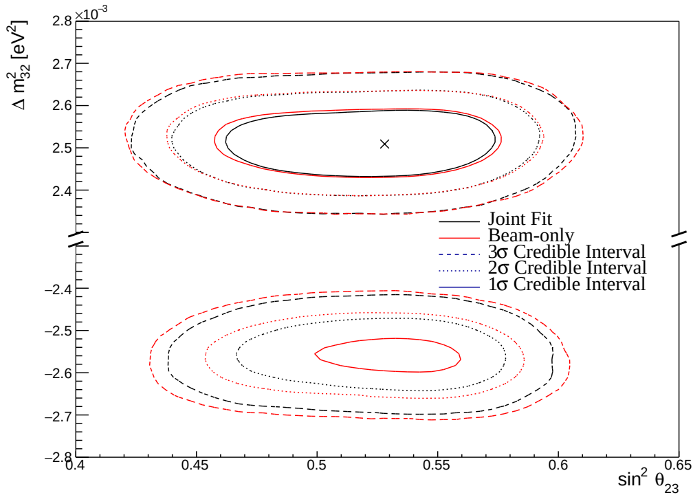
Figure 8.39: The two-dimensional posterior probability density distribution in \Delta m_{32}^2 - \sin^2(\theta_{23}) compared between the joint beam-atmospheric fit (Black) and the latest T2K sensitivities (Red) [2, 212]. The reactor constraint is applied in both fits. The marker represents the known value of \Delta m_{32}^2 - \sin^2(\theta_{23}) .
