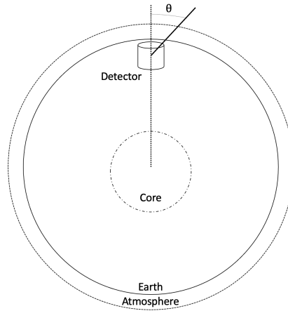
Figure 2.4: A diagram illustrating the definition of zenith angle as used in the Super Kamiokande experiment [54].
