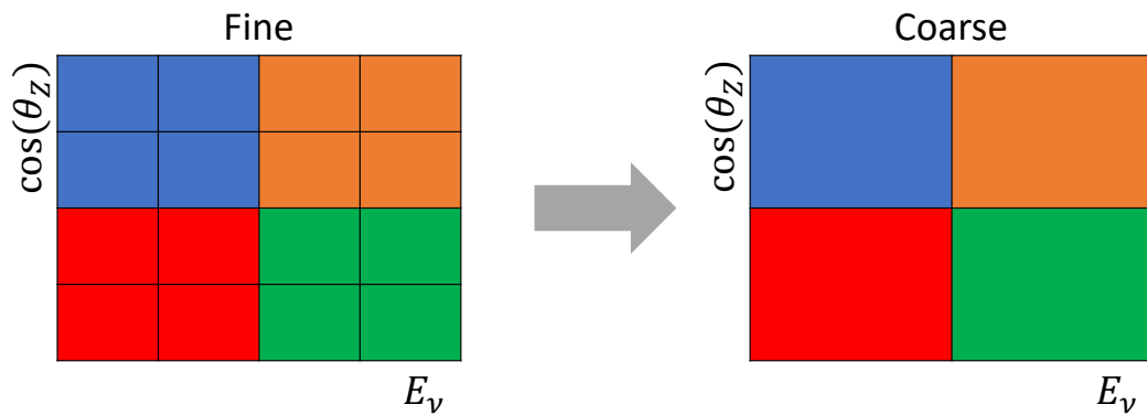
Figure 7.2: Illustration of the averaging procedure for N = 2 . The oscillation probabilities calculated on the finer left binning are averaged to obtain the oscillation probabilities in the coarser right binning. These averaged oscillation probabilities with the coarser binning are then applied to each event during the fit.
