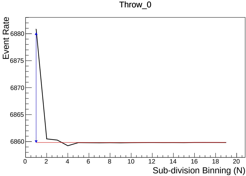
Figure 7.4: Event rate of the SubGeV_elike_0dcy sample, for a particular oscillation parameter throw, as a function of the number of sub-divisions, N , per coarse bin. The difference between the mean event rate (red), \bar{\lambda} , and the event rate at N = 1 , \lambda^{N=1} is defined as \lambda^N - \bar{\lambda} and illustrated by the blue arrow.
