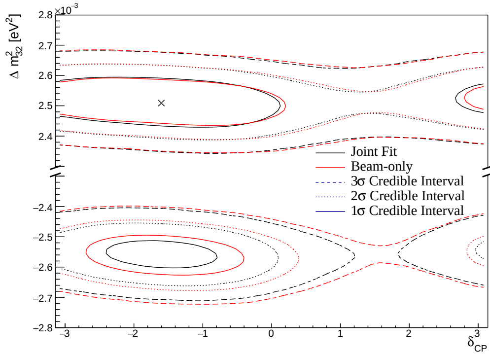
Figure 8.36: The two-dimensional posterior probability density distribution in \Delta m_{32}^2 - \Delta_{CP} compared between the joint beam-atmospheric fit (Black) and the latest T2K sensitivities (Red) [2, 212]. The reactor constraint is not applied in either fit. The marker represents the known value of \Delta m_{32}^2 - \Delta_{CP} .
