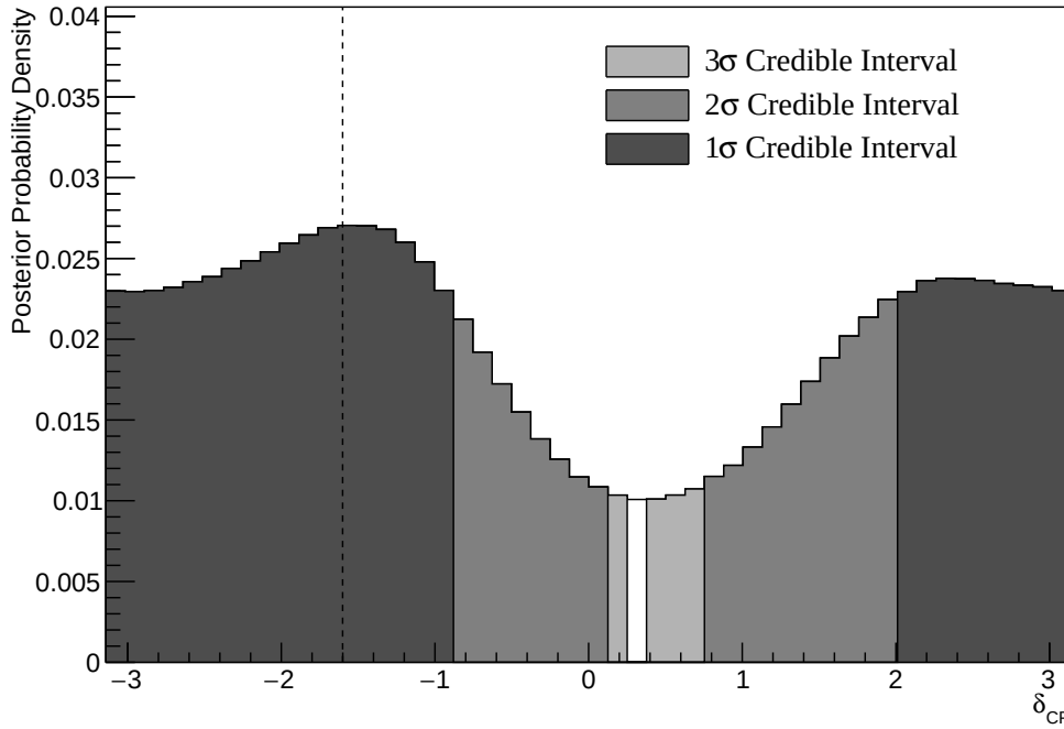
Figure 8.7: The one-dimensional posterior probability density distribution in \delta_{CP} , marginalised over both hierarchies, from the SK atmospheric-only fit. The reactor constraint is not applied. The vertical dashed line represents the known value of \delta_{CP} .
