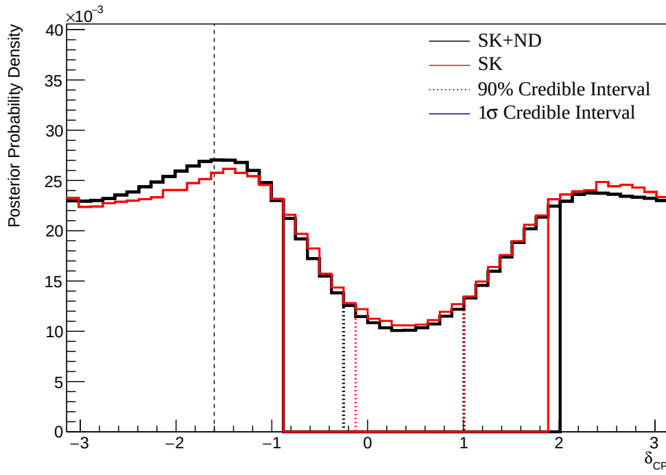
Figure 8.15: The one-dimensional posterior probability density distribution in \delta_{CP} compared between the SK atmospheric-only fit where the near detector constraint is (Black) and is not (Red) applied. The distributions are marginalised over both hierarchies. The reactor constraint is not applied in either fit. The vertical dashed line represents the known value of \delta_{CP} .
