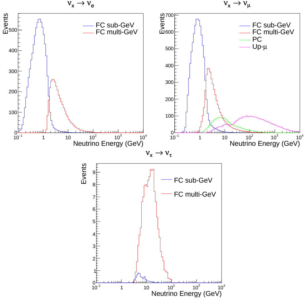
Figure 5.11: The predicted neutrino flux of the fully contained (FC) sub-GeV and multi-GeV, partially contained (PC), and upward-going muon (Up- \mu ) events. The prediction is broken down by the \nu_x \rightarrow \nu_e prediction (top left), \nu_x \rightarrow \nu_\mu prediction (top right) and \nu_x \rightarrow \nu_\tau prediction (bottom). \nu_x represents the flavours of neutrinos produced in the cosmic ray showers (electron and muon). Asimov A oscillation parameters are assumed (given in Table 2.2).
