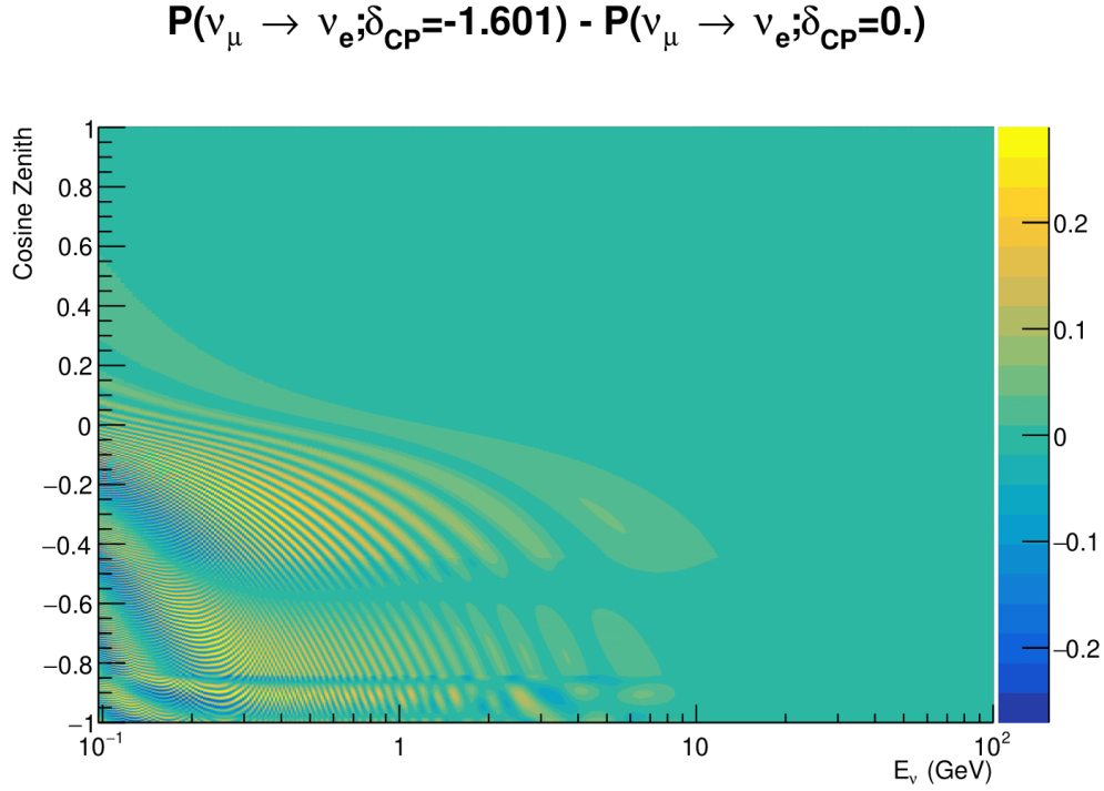
Figure 2.10: The effect of \delta_{CP} for atmospheric neutrinos given in terms of the neutrino energy and zenith angle. This oscillogram compares the P(\nu_\mu \rightarrow \nu_e) oscillation probability for a CP conserving ( \delta_{CP} = 0.0 ) and a CP violating ( \delta_{CP} = -1.601 ) value taken from the Asimov A parameter set. The other oscillation parameters assume the Asimov A oscillation parameter set given in Table 2.2.
