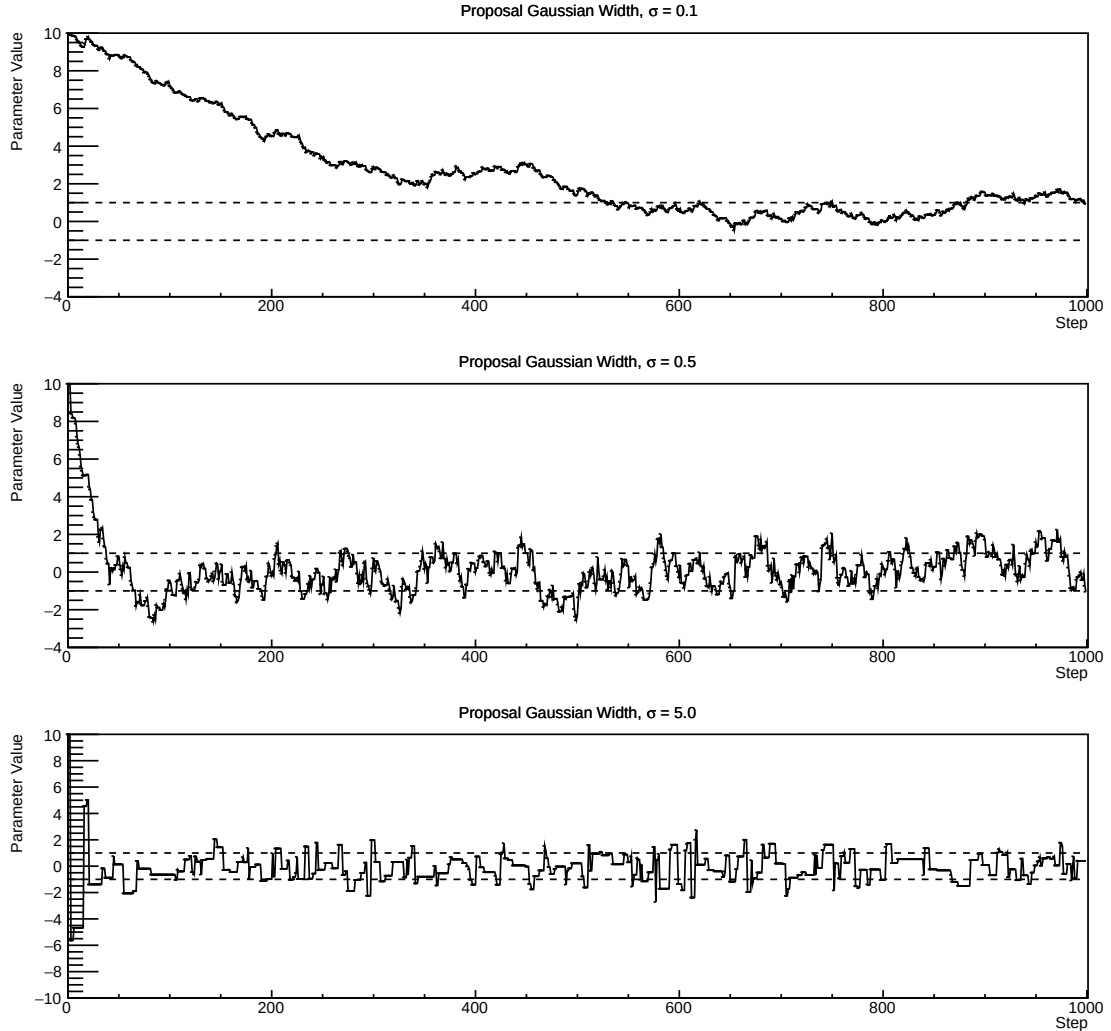
Figure 4.3: Three MCMC chains, each with a stationary distribution equal to a Gaussian centered at 0 and width 1 (As indicated by the black dotted lines). All of the chains use a Gaussian proposal function but have different widths (or ‘step size \sigma ’). The top panel has \sigma = 0.1 , middle panel has \sigma = 0.5 and the bottom panel has \sigma = 5.0 .
