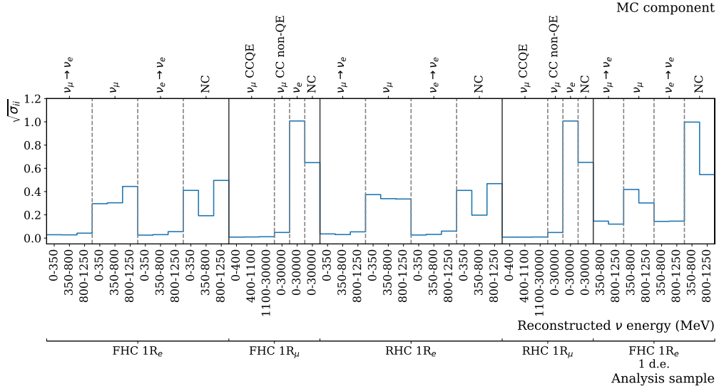
Figure 6.12: The fractional uncertainty on each of the 44 parameters describing the SK detector systematics (The energy scale systematic is neglected). The parameters are split by sample, oscillation channel, interaction mode, and reconstructed neutrino energy.
