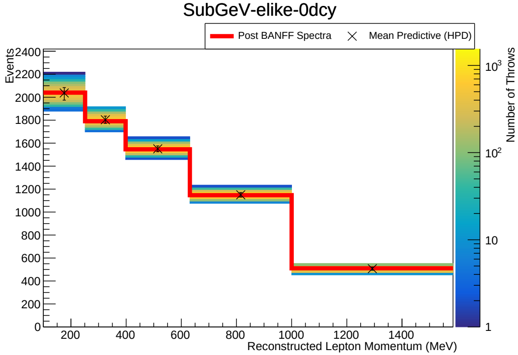
Figure 8.44: Result of the posterior predictive method for the SubGeV_elike_0dcy sample after sampling 2000 steps from the joint beam-atmospheric chain detailed in subsection 8.3.4 (Coloured histogram). The mean and uncertainty is presented for each bin. The Asimov data prediction (denoted ‘Post BANFF Spectra’, Red) assumes the post-BANFF tune and Asimov A oscillation parameters.
