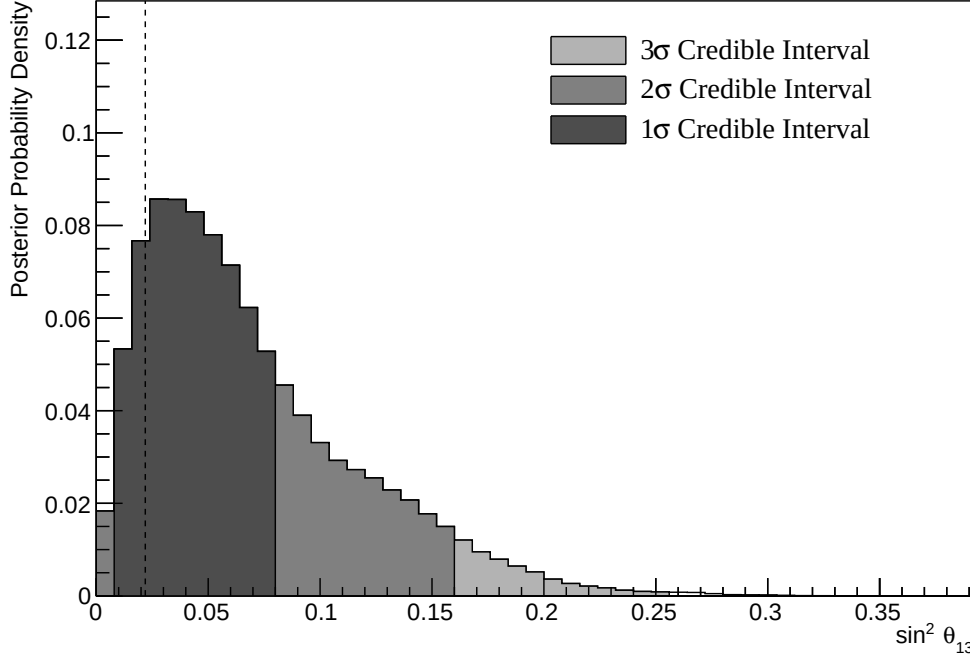
Figure 8.9: The one-dimensional posterior probability density distribution in \sin^2(\theta_{13}) , marginalised over both hierarchies, from the SK atmospheric-only fit. The reactor constraint is not applied. The vertical dashed line represents the known value of \sin^2(\theta_{13}) .
