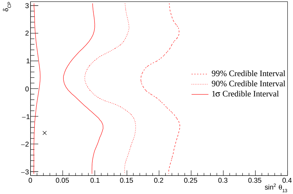
Figure 8.10: The two-dimensional posterior probability density distribution in \delta_{CP}-\sin^2(\theta_{13}) , marginalised over both hierarchies, from the SK atmospheric-only fit. The reactor constraint is not applied. The marker represents the input value.
