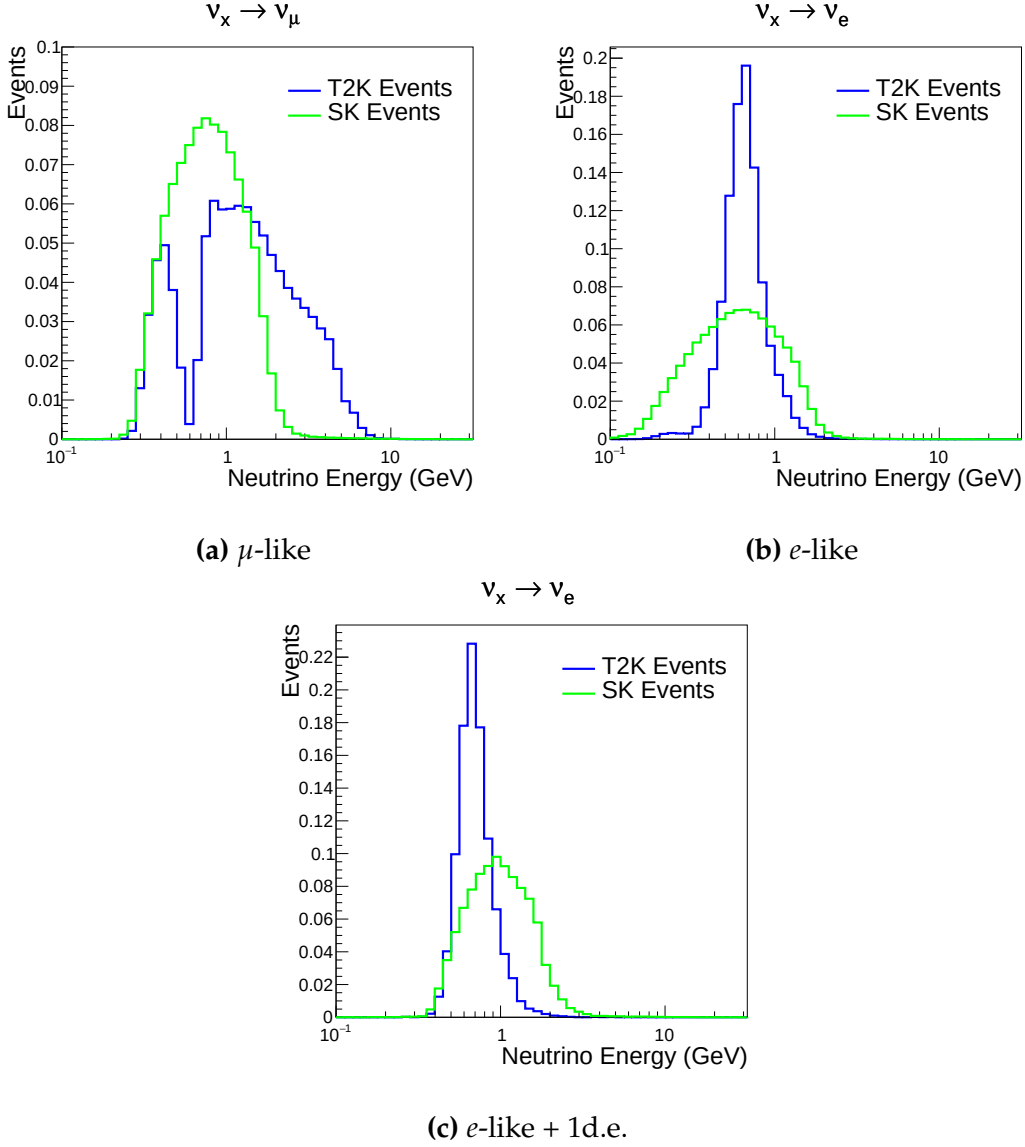
Figure 6.9: The predicted neutrino energy distribution for subGeV atmospheric and beam samples. FHC and RHC beam samples are summed together. Asimov A oscillation parameters are assumed (given in Table 2.2). Beam and atmospheric samples with similar cuts are compared against one another.
