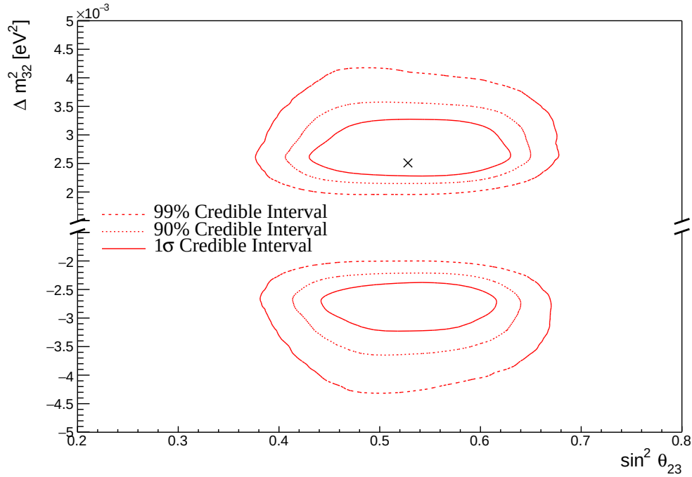
Figure 8.11: The two-dimensional posterior probability density distribution in \Delta m^2_{32}-\sin^2(\theta_{23}) , marginalised over both hierarchies, from the SK atmospheric-only fit. The reactor constraint is not applied. The marker represents the input value.
