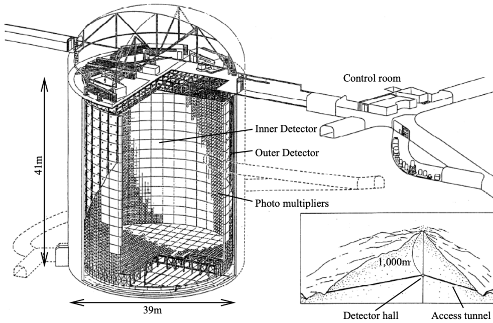
Figure 3.1: A schematic diagram of the Super-Kamiokande Detector. Taken from [84].
