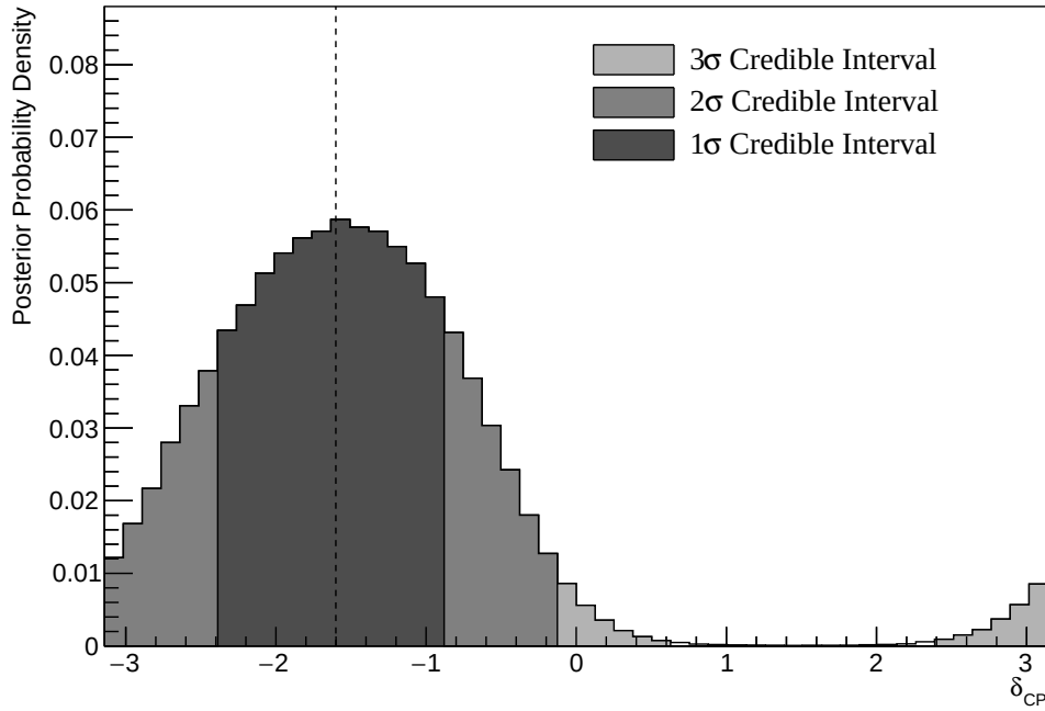
Figure 8.23: The one-dimensional posterior probability density distribution in \delta_{CP} , marginalised over both hierarchies, from the joint beam-atmospheric fit where the reactor constraint is applied. The vertical dashed line represents the known value.
