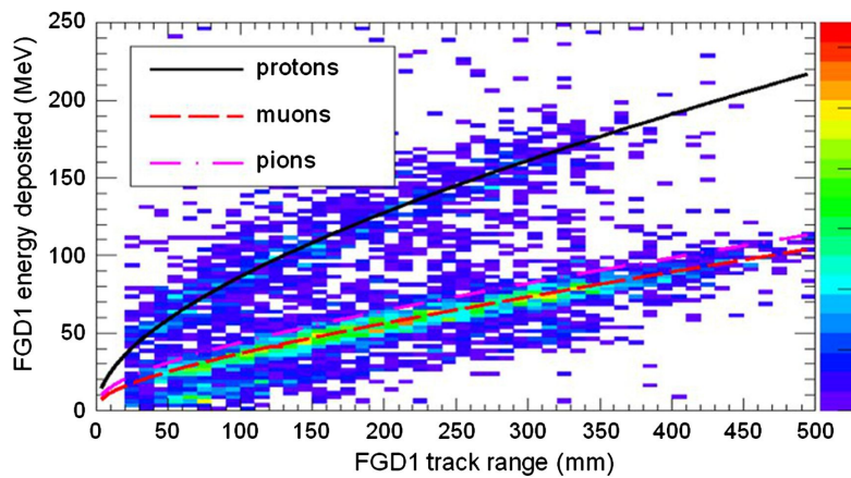
Figure 3.9: Comparison of data to Monte Carlo prediction of integrated deposited energy as a function of track length for particles that stopped in FGD1. Taken from [112].
