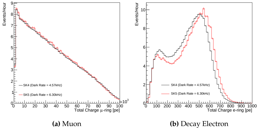
Figure 5.7: Comparison of the measured raw charge deposited per event from the stopping muon data samples between SK-IV (Black) and SK-V (Red), split by the primary muon subevent (left) and the associated decay electron subevent (right).
