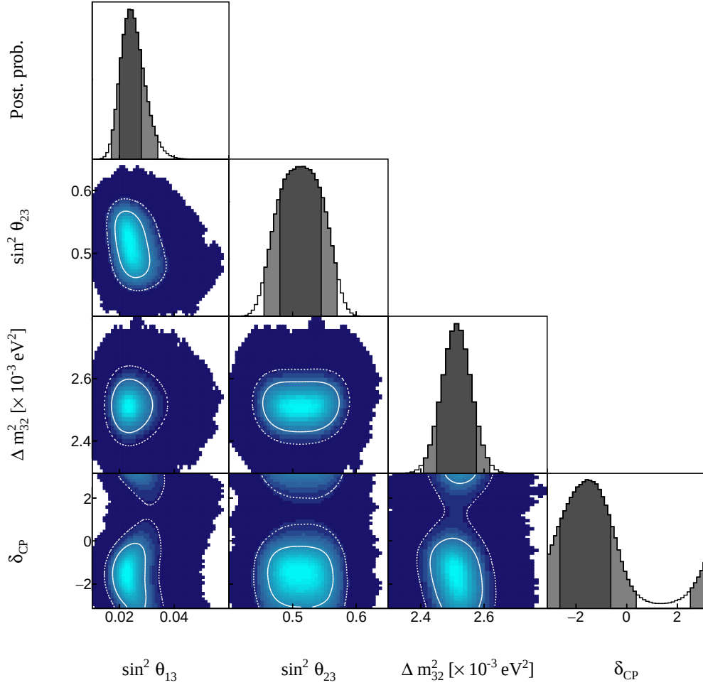
Figure 8.21: The posterior probability density distribution from the joint beam-atmospheric fit. The reactor constraint is not applied. The distribution is given for each two-dimensional permutation of the oscillation parameters of interest where the solid(dashed) white lines represent the 1\sigma(2\sigma) contours. The one-dimensional distribution of each parameter is also given, where the dark(light) grey region represents the 1\sigma(2\sigma) credible intervals.
