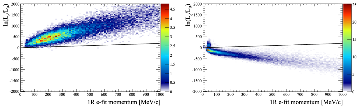
Figure 5.4: The difference of the electron-like and muon-like log-likelihood compared to the reconstructed single-ring fit momentum for atmospheric \nu_e (left) and \nu_\mu (right) samples. The black line represents the cut used to discriminate electron-like and muon-like events, with coefficients obtained from Monte Carlo studies. Figures from [168].
