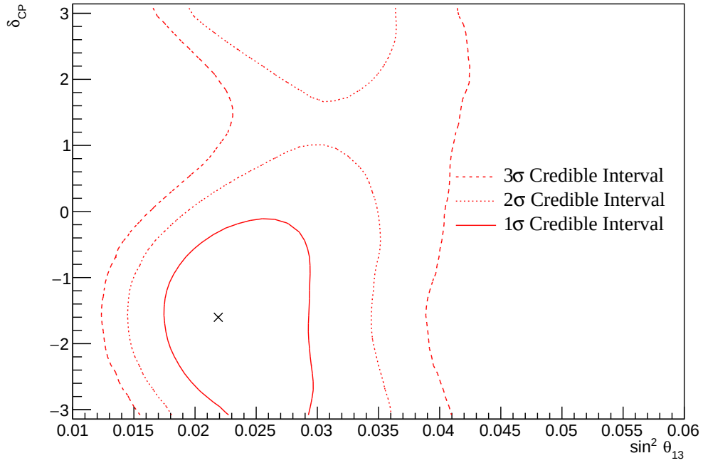
Figure 8.19: The two-dimensional posterior probability density distribution in \delta_{CP}-\sin^2(\theta_{13}) , marginalised over both hierarchies, from the joint beam-atmospheric fit. The reactor constraint is not applied. The marker represents the input value.
