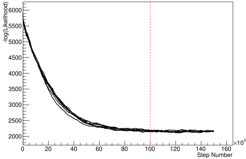
Figure 4.4: The log-likelihood from the fit detailed in subsection 8.3.4 as a function of the number of steps accumulated in each fit. Many independent MCMC chains were run in parallel and overlaid on this plot. The red line indicates the 1 \times 10^5 step burn-in period after which the log-likelihood becomes stable.
