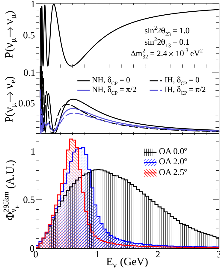
Figure 3.7: Top panel: T2K muon neutrino disappearance probability as a function of neutrino energy. Middle panel: T2K electron neutrino appearance probability as a function of neutrino energy. Bottom panel: The neutrino flux distribution for three different off-axis angles (Arbitrary units) as a function of neutrino energy.
