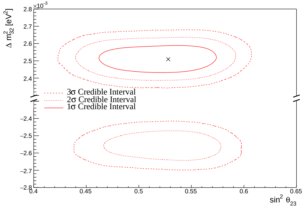
Figure 8.29: The two-dimensional posterior probability density distribution in \Delta m^2_{32} - \sin^2(\theta_{23}) , marginalised over both hierarchies, from the joint beam-atmospheric fit where the reactor constraint is applied. The marker represents the known value.
