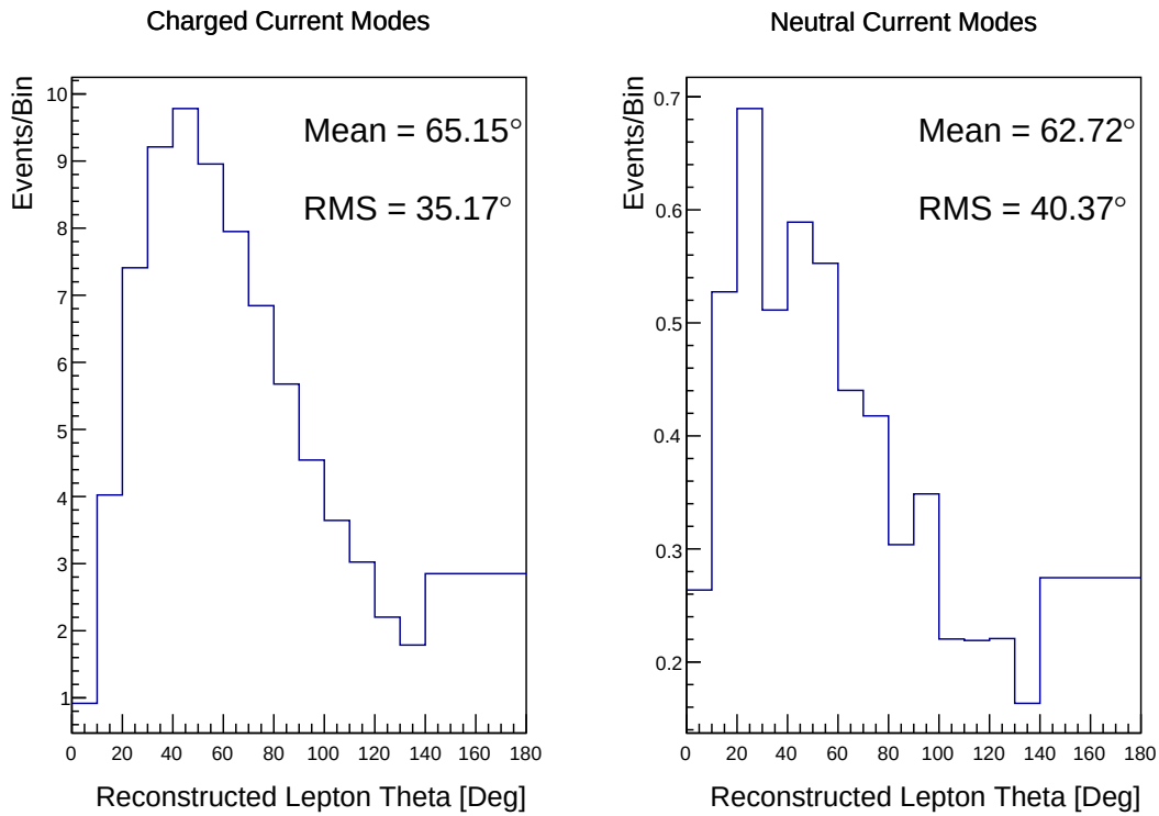
Figure 6.6: The distribution of the angle between the neutrino beam direction and the reconstructed final state lepton, for the FHC 1Re-like sample. The distribution is broken down by neutrino interaction mode into charged current (left) and neutral current (right) components. Asimov A oscillation parameter sets are assumed (given in Table 2.2). The RMS of the charged and neutral current plots are 35.17° and 40.37°, respectively.
