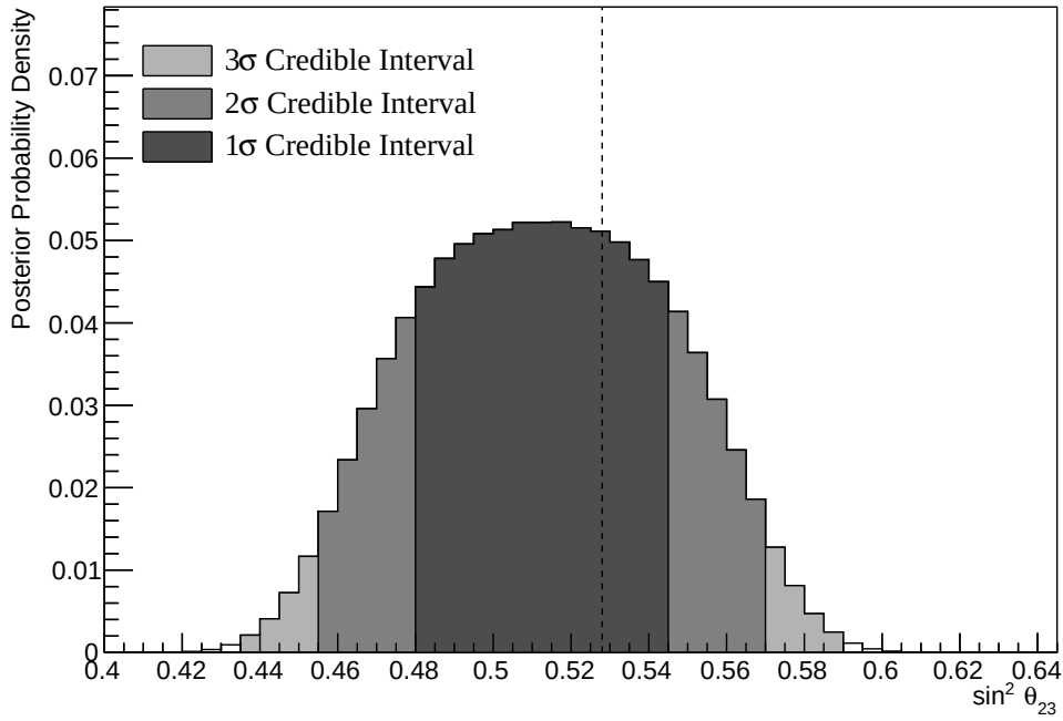
Figure 8.18: The one-dimensional posterior probability density distribution in \sin^2(\theta_{23}) , marginalised over both hierarchies, from the joint beam-atmospheric fit. The reactor constraint is not applied. The vertical dashed line represents the known value of \sin^2(\theta_{23}) .
