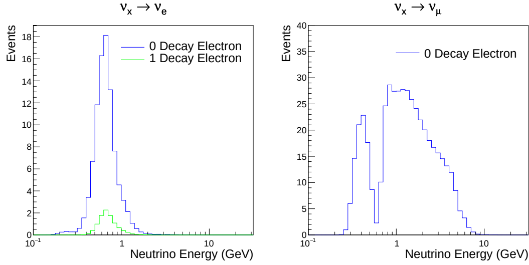
Figure 5.12: The predicted flux of beam neutrinos, as a function of neutrino energy. The predictions are broken down by the number of decay electrons associated with the particular events. Asimov A oscillation parameters are assumed (given in Table 2.2).
