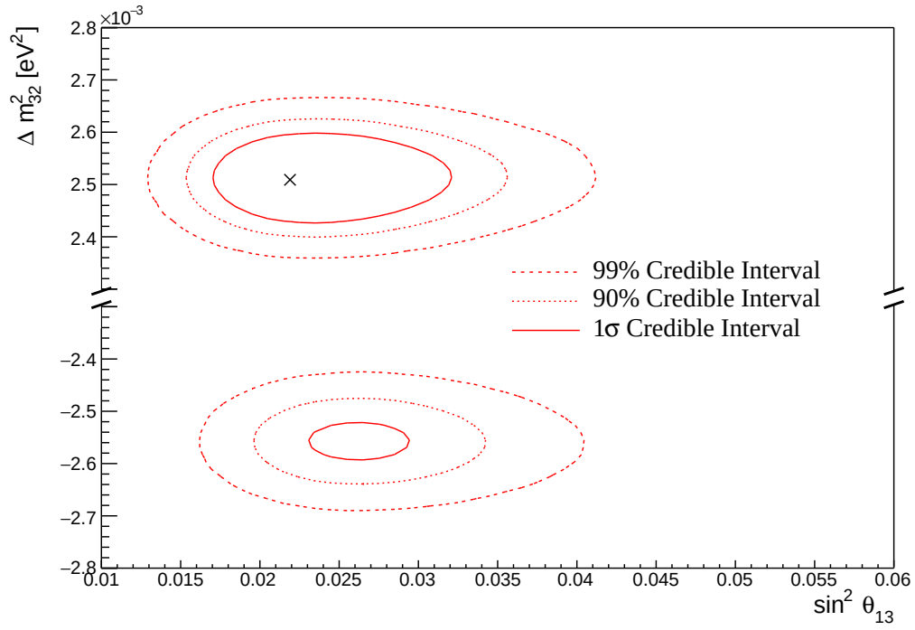
Figure 8.22: The two-dimensional posterior probability density distribution in \Delta m_{32}^2 - \sin^2(\theta_{13}) , marginalised over both hierarchies, from the joint beam-atmospheric fit. The reactor constraint is not applied. The marker represents the known value of \Delta m_{32}^2 - \sin^2(\theta_{13}) .
