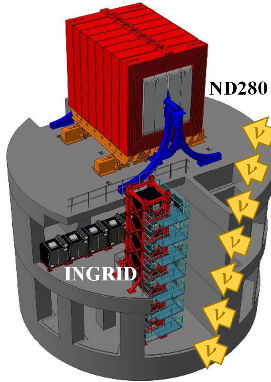
Figure 3.4: The near detector suite for the T2K experiment showing the ND280 and INGRID detectors. The distance between the detectors and the beam target is 280m.
