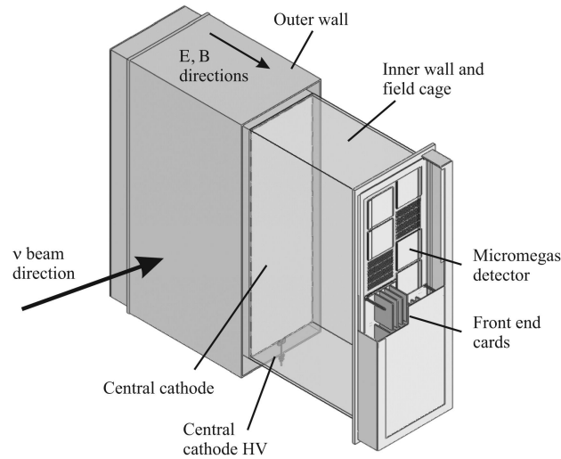
Figure 3.10: Schematic design of a Time Projection Chamber detector. Taken from [113].
