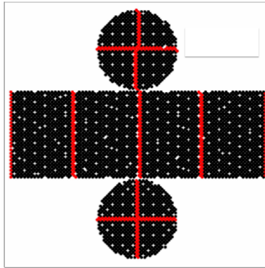
Figure 3.2: The location of “standard PMTs” (red) inside the SK detector. Taken from [80].
