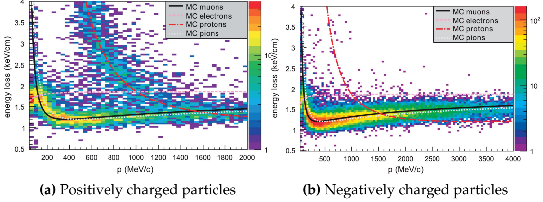
Figure 3.11: The distribution of energy loss as a function of reconstructed momentum for charged particles passing through the TPC, comparing data to Monte Carlo prediction. Taken from [113].
