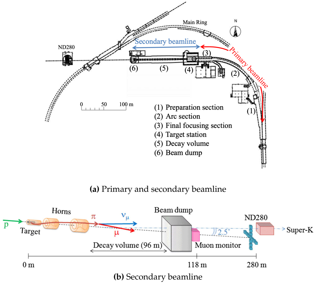
Figure 3.5: Top panel: Bird's eye view of the most relevant part of primary and secondary beamline used within the T2K experiment. The primary beamline is the main-ring proton synchrotron, kicker magnet, and graphite target. The secondary beamline consists of the three focusing horns, decay volume, and beam dump. Figure taken from [42]. Bottom panel: The side-view of the secondary beamline including the focusing horns, beam dump and neutrino detectors. Figure taken from [109].
