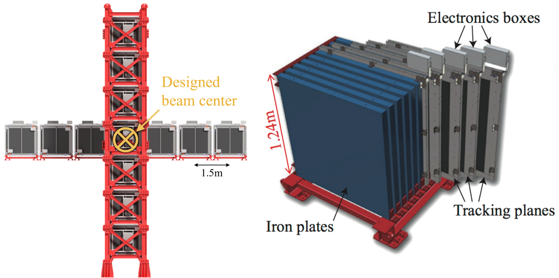
Figure 3.13: Left panel: The Interactive Neutrino GRID on-axis Detector. 14 modules are arranged in a cross-shape configuration, with the center modules being directly aligned with the on-axis beam. Right panel: The layout of a single module of the INGRID detector. Both figures are recreated from [42].
