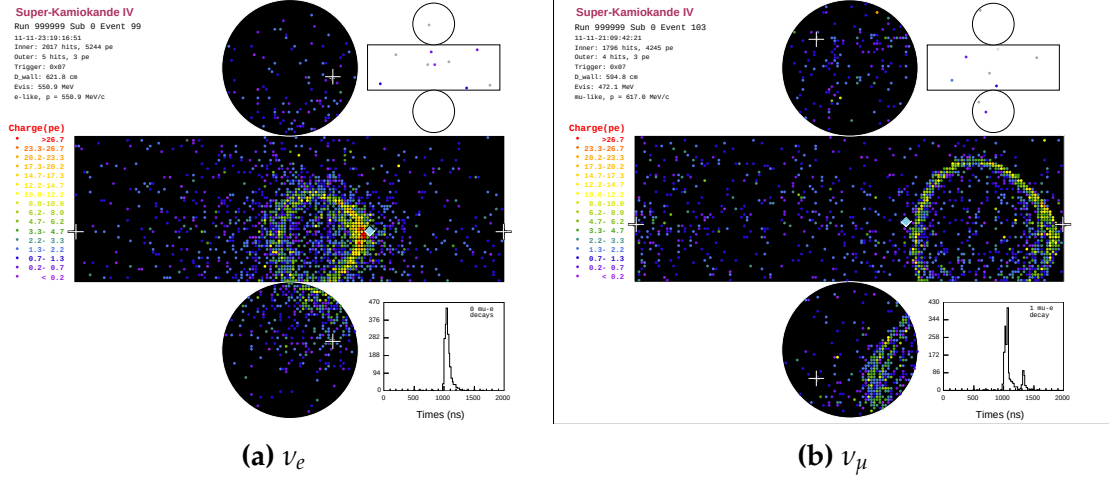
Figure 5.3: Event displays from Monte Carlo simulation at Super Kamiokande illustrating the “crisp” ring from a muon and the typically “fuzzier” electron ring. Each pixel represents a PMT and the color scheme denotes the accumulated charge deposited on that PMT. Figures taken from [167].
