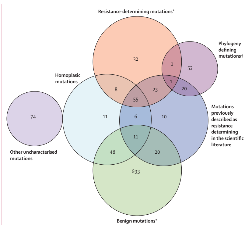
Figure 4: Training-set-characterised mutations
