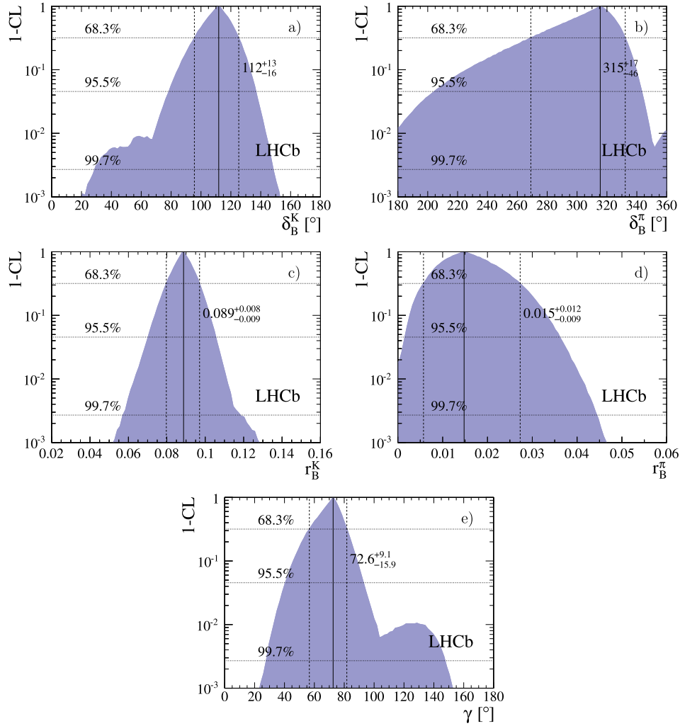
Fig. 3. Graphs showing 1 - \text{CL} for (a) \delta_B^K , (b) \delta_B^{\pi^\pm} , (c) r_B^K , (d) r_B^{\pi^\pm} , and (e) \gamma , for the full DK^\pm and D\pi^\pm combination. The reported numbers correspond to the best-fit values and the uncertainties are computed using appropriate 68.3% CL confidence intervals shown in Table 7.
