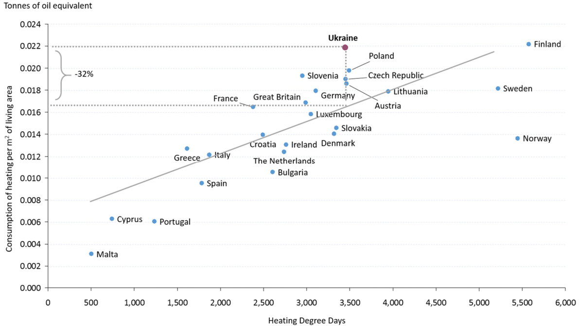
Figure 14: Heating usage per square metre of living area in Ukraine, comparison with European countries, 2013
