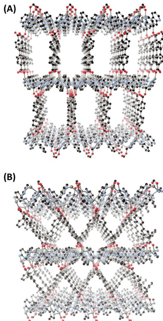
Fig. 4 Comparison of the pore structures in MOFs 1 (A) and 2 (B).
