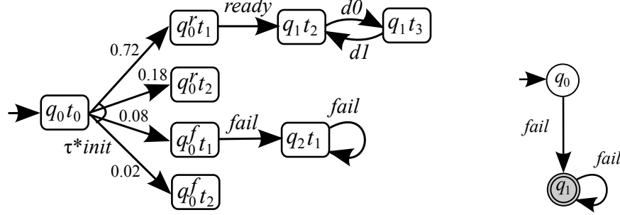
Figure 5.3: p_{ios}(\mathcal{A}) \parallel \mathcal{M}_2 and a DFA G^{err} for Example 5.16
