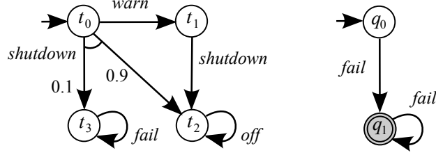
Figure 4.18: PA \mathcal{M}_3 and a DFA G^{err} for Example 4.16
