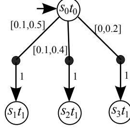
Figure 6.6: The behaviour of state s_0 t_0 in an example IDTMC \mathcal{I} \parallel \mathcal{D}
