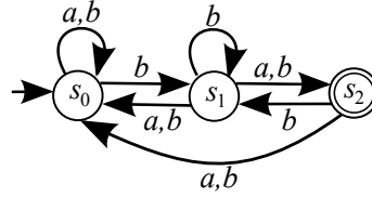
Figure 3.10: Minimal RFSA accepting language \mathcal{L} = \alpha^*b\alpha with 3 states
