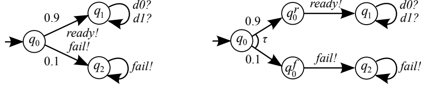
Figure 5.2: RPA \mathcal{A} and its PIOS conversion \text{pios}(\mathcal{A}) (taken from [FHKP11a])
