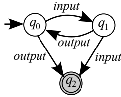
Figure 4.12: DFA G^{err} for Example 4.15
