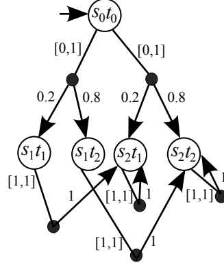
Figure 6.5: The synchronous parallel composition \mathcal{I} \parallel \mathcal{D}_2 (for \mathcal{I} and \mathcal{D}_2 in Figure 6.4)
