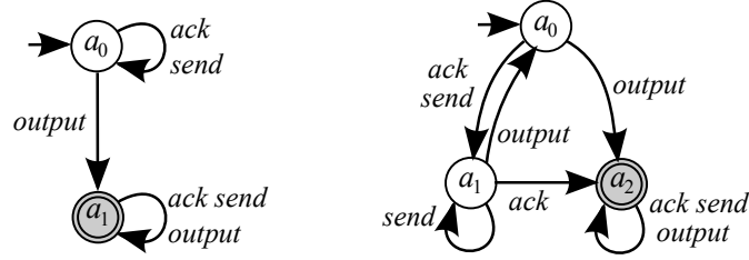
Figure 4.13: Learnt DFAs A_1^{err} , A_2^{err} for Example 4.15
