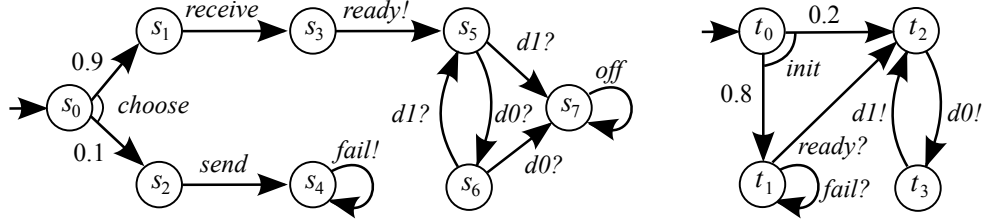
Figure 5.1: A pair of PIOSs \mathcal{M}_1 and \mathcal{M}_2 (taken from [FHKP11a])
