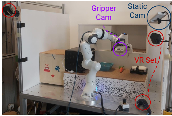
Fig. 5: Visualization of the complete real-world robot setup. This figure highlights the static and gripper cameras, as well as the VR controller and tracking system.
