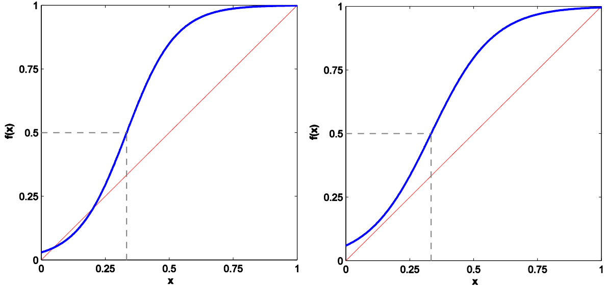
Figure 2 – The response functions for payoff gain \alpha = 100\% and initial error rate \varepsilon = 3\% (left panel) and \varepsilon = 6\% (right panel). The two systems have three equilibria and a unique equilibrium, respectively. In each case, the vertical dashed line corresponds to the indifference point of the pure best response.
