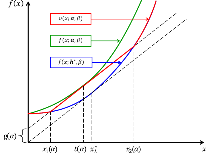
Figure 8 – The function v(x, \alpha) (red) is a lower bound for f(x; \alpha) (green)
