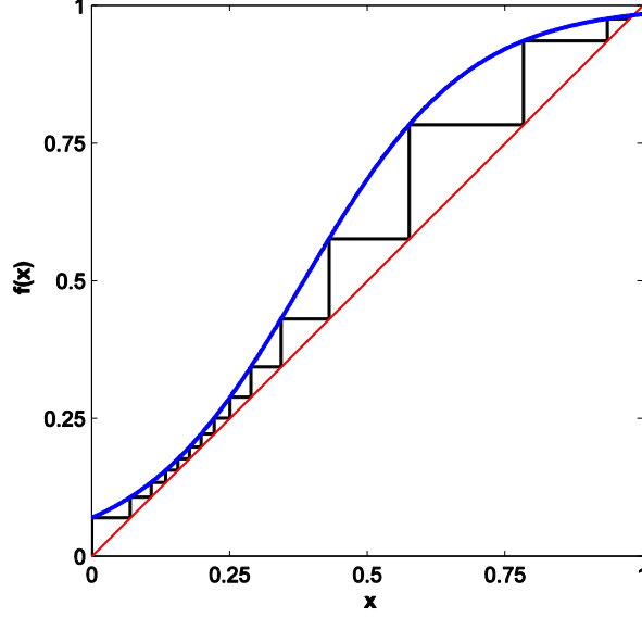
Figure 6 – An informal illustration of the evolution of the process
