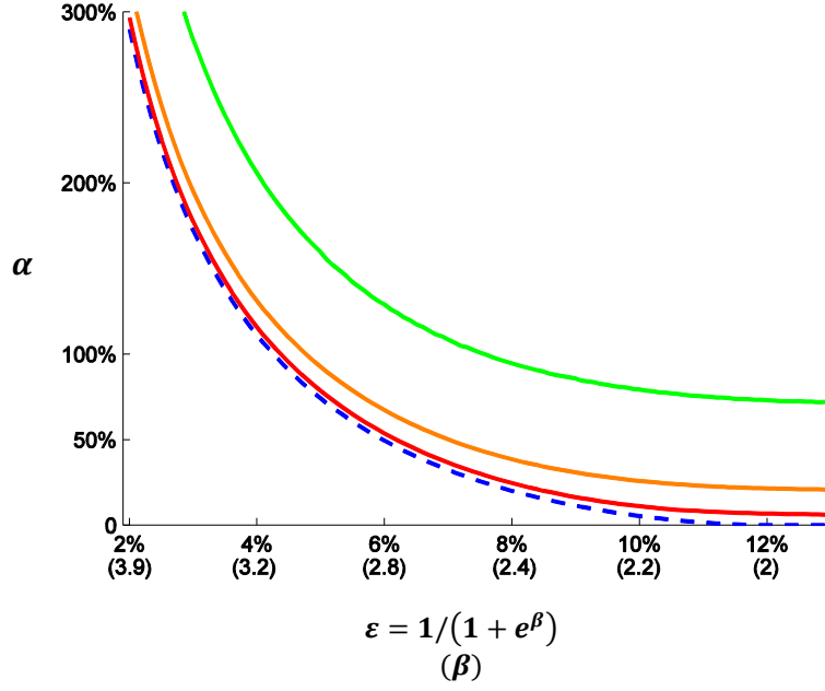
Figure 5 – Waiting times to within \delta = 1\% of the high equilibrium; 40 (red), 20 (orange) and 10 (green) revisions per capita. The x-axis is labeled with the initial error rate \varepsilon ; the corresponding noise level \beta appears in parentheses.
