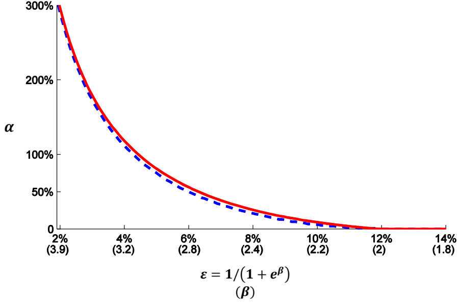
Figure 1 - The critical threshold for fast selection. Simulation (blue, dashed) and upper bound (red, solid). The x-axis is labeled with the initial error rate \epsilon ; the corresponding noise level \beta appears in parentheses.
