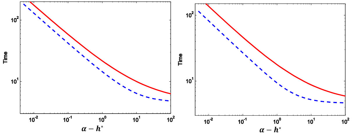
Figure 7 – Waiting time until the process is within \delta = 1\% of the high equilibrium, as a function of the payoff gain differential \alpha - h^* . Both axes have logarithmic scales. Simulation (blue, dashed) and upper bound (red, solid). Initial error rates \varepsilon = 1\% (left panel) and \varepsilon = 5\% (right panel).
