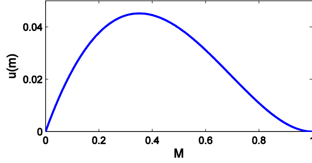
Figure 12 – The function u(M)
