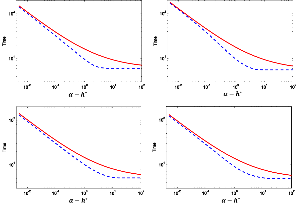
Figure 10 – Waiting time until the process is within \delta = 1\% of the high equilibrium, as a function of the payoff gain difference \alpha - h^* . Both axes have logarithmic scales. Simulation (blue, dashed) and upper bound (red, solid). Information parameters and initial error rates, and values for constant S :
