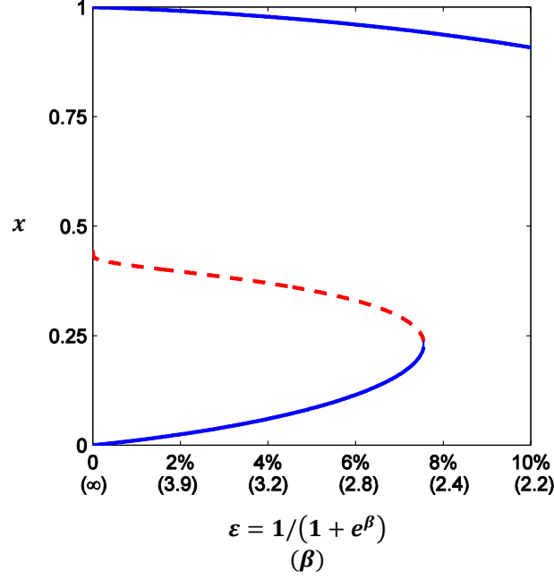
Figure 4 – Rest points of the deterministic process ( \alpha = 25\% ): stable rest points (blue, solid line) and unstable rest points (red, dashed line). The x -axis is labeled with the initial error rate \varepsilon ; the corresponding noise level \beta appears in parentheses.
