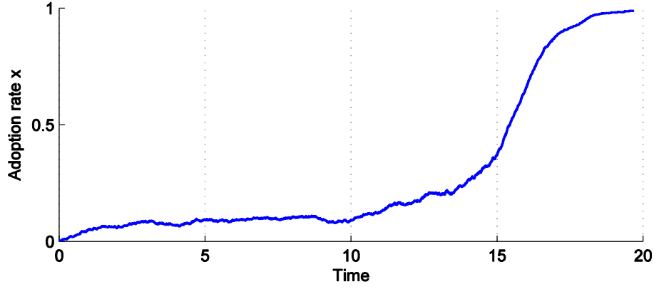
Figure 3 – Adoption path to 99%, \alpha = 100\% , \varepsilon = 5\% ( \beta \approx 3 ), N = 1000 .
