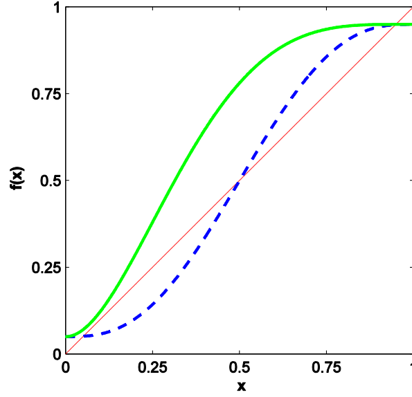
Figure 11 – Response functions for the uniform error model with \varepsilon = 5\% , sample size d = 5 , and \alpha = 40\% (blue, dashed line) , \alpha = 50\% (green, solid line).
