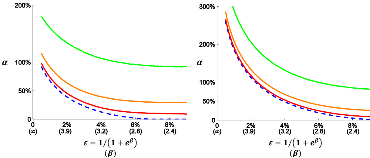
Figure 9 – Waiting times to within \delta = 1\% of the high equilibrium, for d = 4 (left panel) and d = 10 (right panel). Waiting times on solid lines are 40 (red), 20 (orange) and 10 (green) revisions per capita. The x-axis is labeled with the initial error rate \varepsilon ; the corresponding noise level \beta appears in parentheses.
