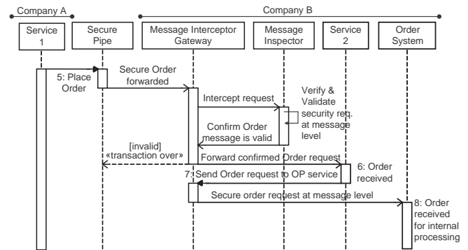
Figure 15. UML process model with patterns applied
