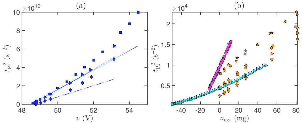
Figure 2.8: Re-scaling the pull-in times according to the scaling law t_{PI} = O(\epsilon^{-1/2}) as \epsilon \rightarrow 0 for (a) the data of Grétilat et al. (1997) and (b) all accelerometer data. (Reprinted from Gomez et al. (2018a), DOI: https://doi.org/10.1088/1361-6439/aa9a70 . Copyright © IOP Publishing. Reproduced with permission. All rights reserved.)
