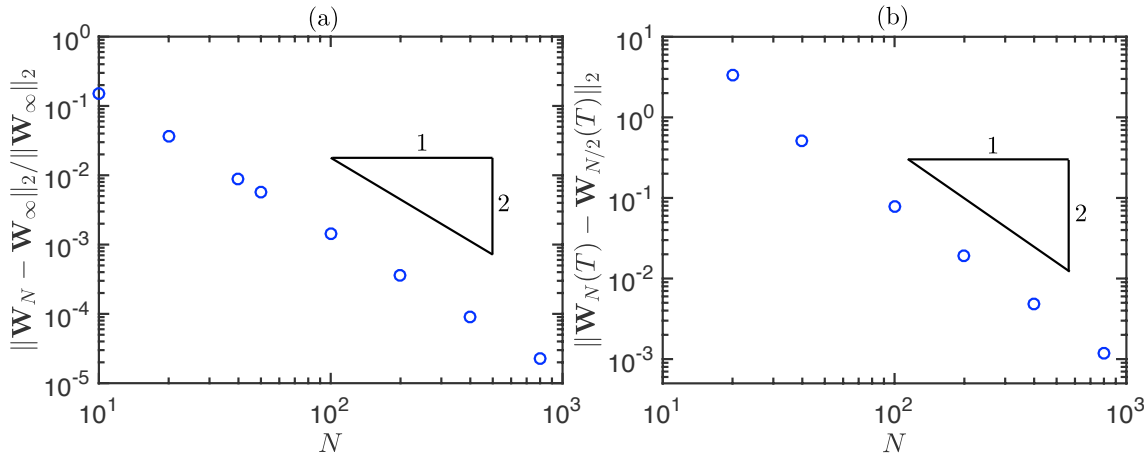
Figure 3.8: (a) Relative error between the steady solution of the discretised system for N grid points, \mathbf{W}_N , and the solution \mathbf{W}_\infty of the steady beam equation ( \lambda = 100 , \mathcal{S} = 10^{-2} , \tau_0 = 0 ). (b) Difference between successive solutions of the unsteady equations as N increases ( \lambda = 200 , T = 3 \times 10^{-3} , Q = 10^{-2} , \mathcal{S} = 10^{-2} , \tau_0 = 0 ).
