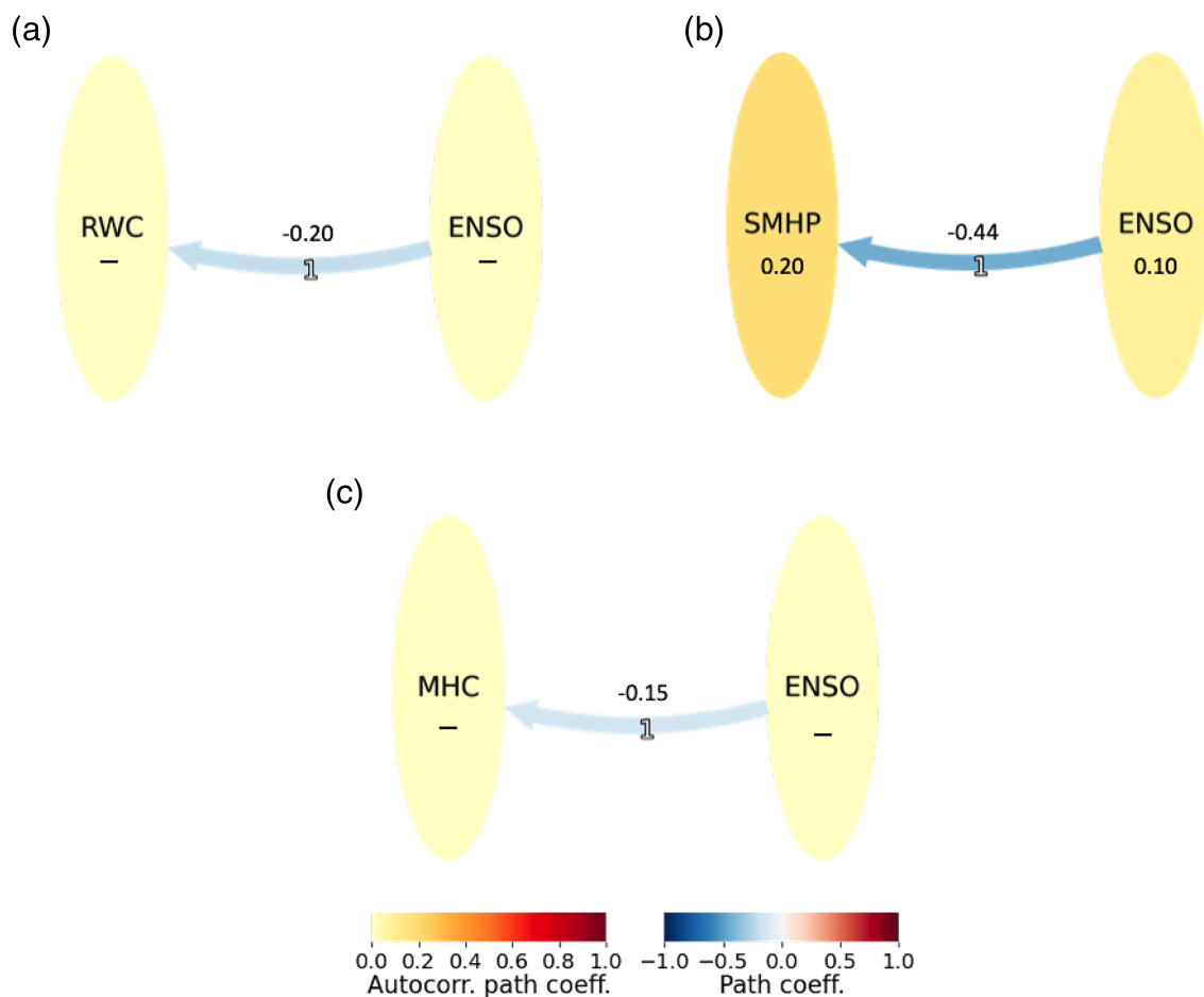
FIGURE 3 CENs showing the causal links that involve a one-way interaction with ENSO: (a) ENSO \rightarrow RWC, (b) ENSO \rightarrow SMHP, and (c) ENSO \rightarrow MHC. For example, ENSO \rightarrow RWC refers to direct links from ENSO to RWC. The nodes represent the indices, with an arrow between the nodes indicating that a statistically significant causal link has been found, with the direction of the arrow showing the direction of the link and the colour showing the path coefficient \beta (also shown as the value above the arrow). The colour of the nodes shows the value of the autocorrelation path coefficient, in case the index influences itself (also shown as the value shown in the node). All causal links have a time lag of one month, as our analysis is limited to this, which is shown as the value on the path coefficient \beta arrow. [Colour figure can be viewed at wileyonlinelibrary.com ]
