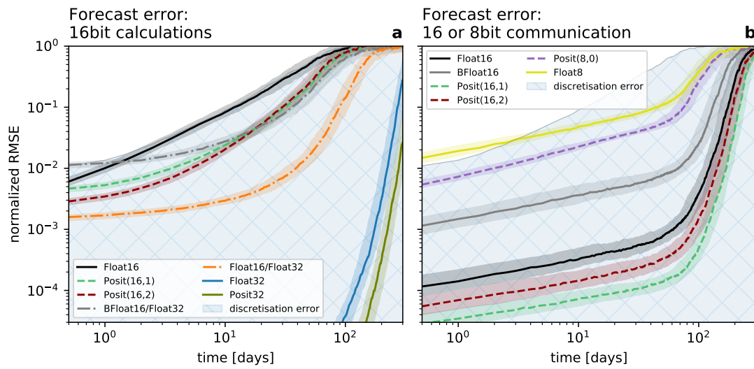
Figure 5.3 | Forecast error of sea surface height \eta measured as root mean square error (RMSE) taking Float64 as reference. a Forecast error for various 16-bit number formats and mixed 16/32-bit simulations for which the prognostic variables are kept in Float32. b Forecast error for reduced-precision communication in 8 or 16 bit with various number formats used for encoding, with Float64 used for all calculations. The communication of boundary values occurs at every time step for the prognostic variables. The RMSE is normalised by a mean forecast error at very long lead times. Solid or dashed lines represent the median of 200 forecasts per number format. The shaded areas of each model configuration denote the interquartile range of the forecast experiments. Only the finite numerical precision contributes to the forecast error here by construction.
