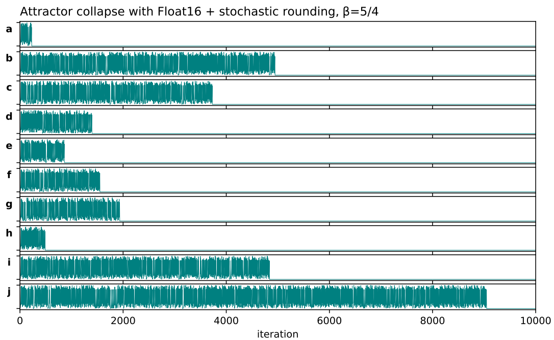
Figure 4.7 | Attractor collapse of the generalised Bernoulli map with Float16 and stochastic rounding. a-j Simulation of the Bernoulli starting from identical initial conditions and \beta = 5/4 . Only the the state of the random number generator for stochastic rounding differs between a-j . After 10,000 iterations all simulations a-j stalled at the fixed-point 0 of the analytical attractor. The y-axes denote the value of x_i in [0,1] .
