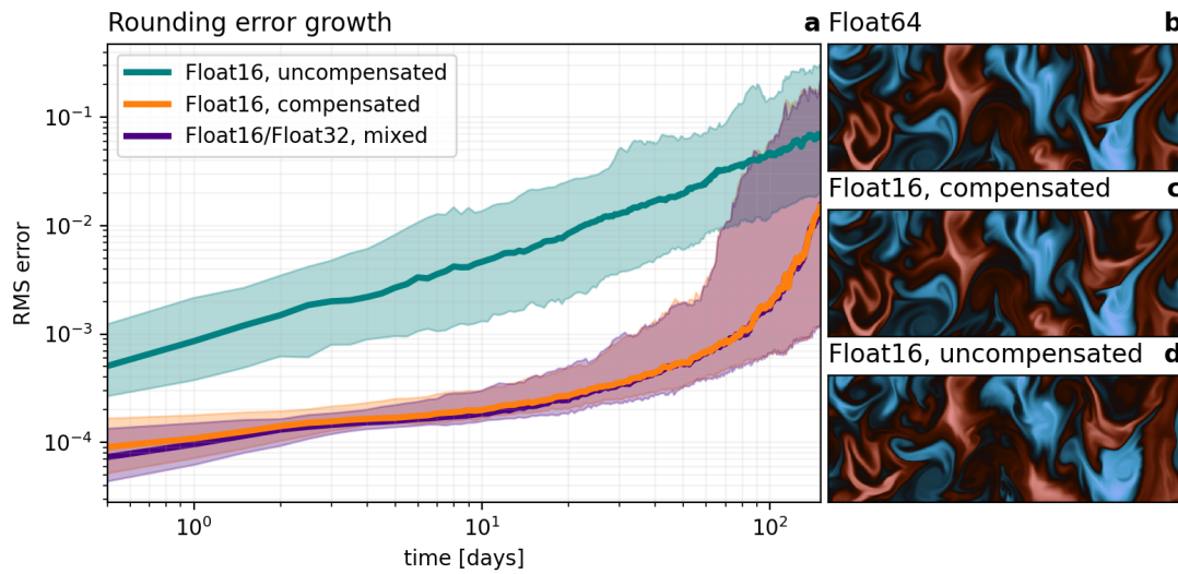
Figure 6.3 | Rounding error growth with Float16 in ShallowWaters.jl using compensated time integration or mixed precision. a Errors are root-mean square (RMS) errors of zonal velocity u relative to Float64. Solid lines denote the median and shadings the interdecile confidence interval. b,c Snapshots of tracer q from a zoom into Fig. 6.4 after 100 days of simulation and d as c but without compensated time integration.
