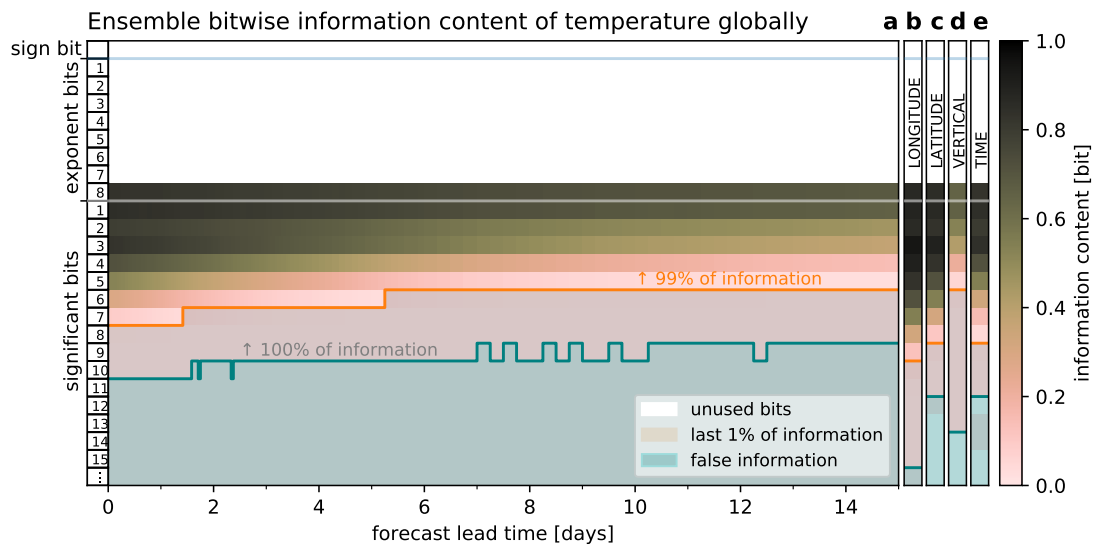
Figure 3.18 | Bitwise real information content for temperature in various dimensions. a ensemble, b longitude, c latitude, d vertical and e forecast lead time. The ensemble information effectively encodes the ensemble mean, which is less information than in most other dimensions. Longitude, latitude and forecast lead time have the highest total information which should be preserved in compression. The ensemble information decreases over time as the ensemble spread increases (Fig. 3.17).
