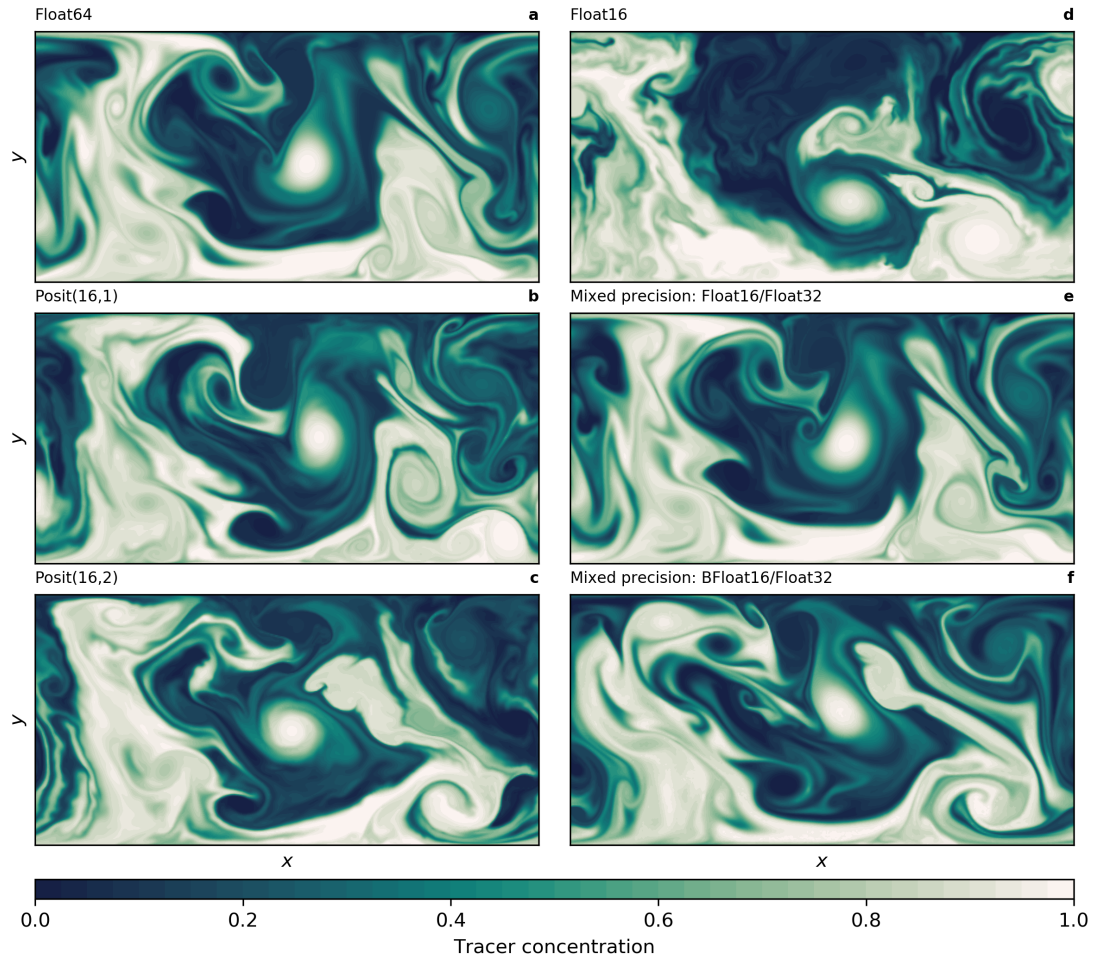
Figure 5.2 | Snapshot of tracer concentration simulated by the shallow water model using different 16-bit number formats. The high-resolution configuration ( \Delta = 5\text{km} ) is used with 400x200 grid points. The mixed-precision simulations presented in e and f use Float32 for the prognostic variables only. The tracer was injected uniformly in the lower half of the domain 50 days before the time step shown.
