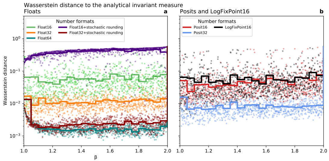
Figure 4.6 | Agreement between the simulated and analytical invariant measures in the generalised Bernoulli map. For all values except \beta = 2 a high precision number format yields a better agreement with the analytical Bernoulli map. Simulations using a Floats with and without stochastic rounding, b Posits and LogFixPoint16. The Wasserstein distances are calculated for the invariant measures obtained from 1000 simulations for every value of \beta . Scatter points denote individual Wasserstein distances, solid lines indicate averages across a range of as indicated by steps.
