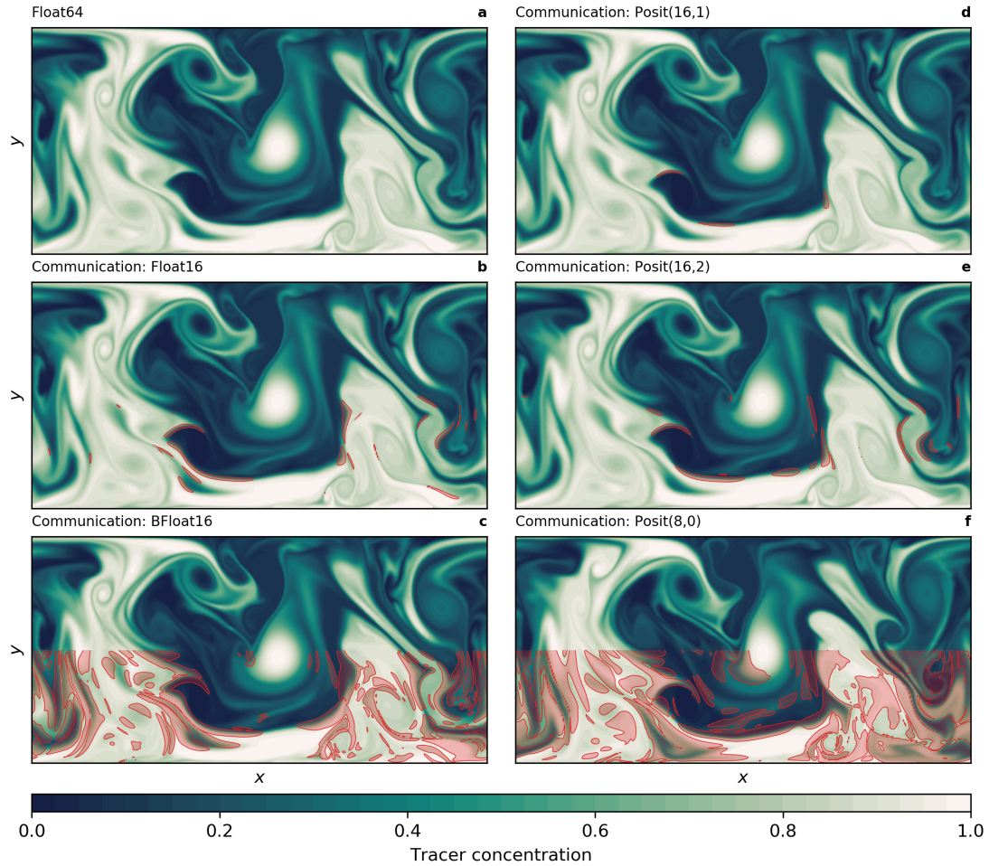
Figure 5.7 | Snapshot of tracer concentration simulated by the shallow water model using reduced-precision communication. The communication of boundary values occurs at every time step for the prognostic variables. Float64 was used for all calculations. Areas where the absolute error exceeds 0.05 are shaded in red only in the lower half of the domain. The tracer was injected uniformly in the lower half of the domain 50 days before. This simulation was run in the high-resolution configuration ( \Delta = 5\text{km} ).
