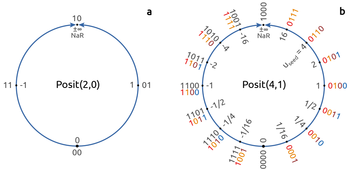
Figure 2.1 | Two posit number formats obtained by projecting the real axis onto a circle. a The 2-bit Posit(2,0) format and b the 4-bit Posit(4,1) format. The bitpatterns are marked on the outside and the respective values on the inside of each circle. Bit patterns of negative numbers (black) have to be converted to their two's complement (colours) first. At the top (12 o'clock) of every posit circle is Not-A-Real (NaR), also called complex infinity ( \pm\infty ), at the bottom (6 o'clock) is always 0, at 3 o'clock always 1 and at 9 o'clock always -1. After Gustafson & Yonemoto [2017] .
