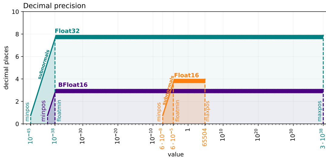
Figure 2.4 | Decimal precision of Float16, BFloat16 and Float32 over the range of representable numbers. The decimal precision is worst-case, i.e. given in terms of decimal places that are at least correct after rounding (see section 2.3.3). The smallest representable number ( minpos ), the smallest normal number ( floatmin ) and the largest representable number ( maxpos ) are denoted with vertical dashed lines (see section 2.1.3). The subnormal range is between minpos and floatmin .
