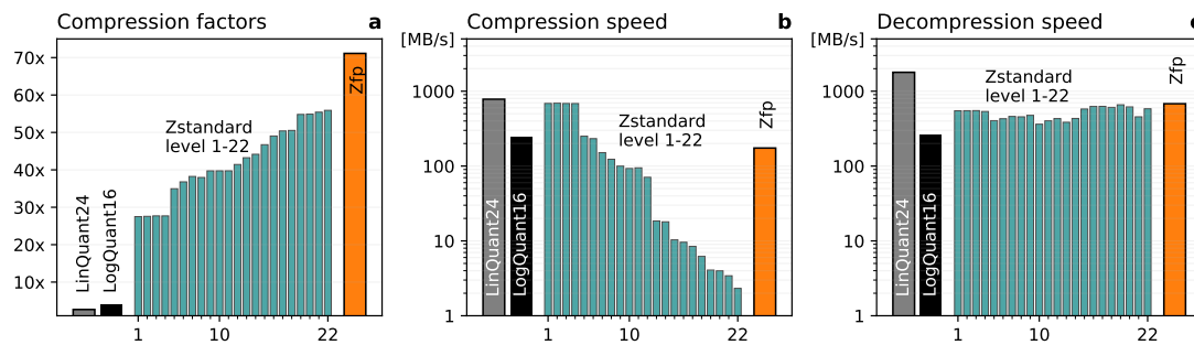
Figure 3.6 | Compressor performances. Compressing water vapour (specific humidity, variable code q) (3 mantissa bits retained, as in Fig. 3.11) with 24-bit linear quantization (LinQuant24), 16-bit logarithmic quantization (LogQuant16), round+lossless (Zstandard, compression level 1-22) and Zfp (precision-mode, including log-preprocessing): a Compression factors, b compression speed, c decompression speed. Timings are single-threaded on an Intel Core™ i7 (Kaby Lake) and do not include the writing to disk.
