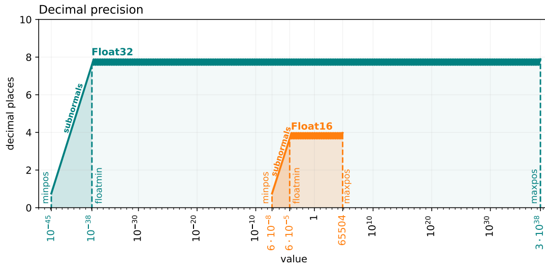
Figure 6.1 | Decimal precision of Float16 and Float32 over the range of representable numbers. The decimal precision is worst-case, i.e. given in terms of decimal places that are at least correct after rounding (see section 2.3.3). The smallest representable number ( minpos , see section 2.1.3), the smallest normal number ( floatmin ) and the largest representable number ( maxpos ) are denoted with vertical dashed lines. The subnormal range is between minpos and floatmin .
