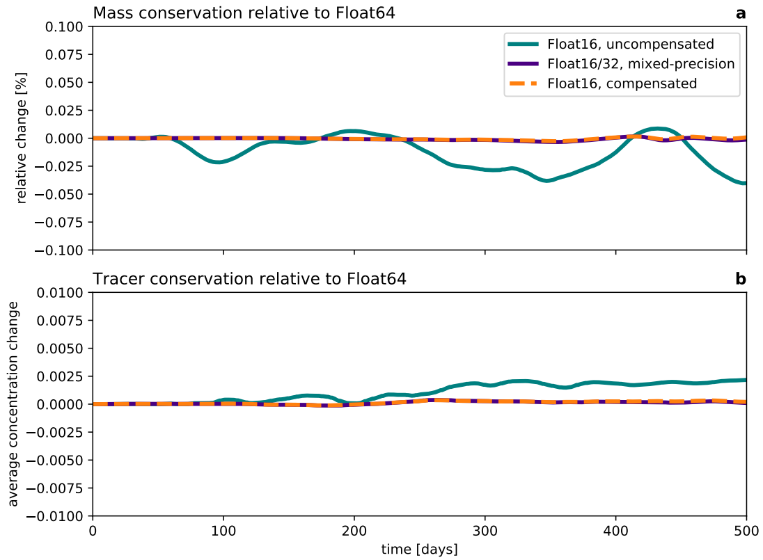
Figure 6.5 | Mass and tracer conservation with Float16 arithmetic. a Mass conservation relative to Float64. b Tracer conservation relative to Float64 in units of tracer concentration with initial conditions in (-1,1) , see Fig. 6.4. Both mass and tracer are well conserved with Float16 arithmetic. Best conservations are obtained with compensated time integration or mixed precision.
