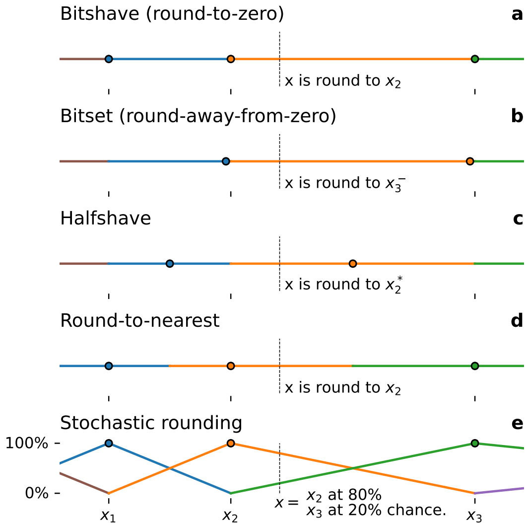
Figure 2.2 | Schematic to illustrate some rounding modes. a Bitshave rounds the exact value x , indicated by a dashed line, down to the next smaller or equal representable number x_2 (all assumed positive). b Bitset rounds x up to x_3^- = x_3 - \epsilon , i.e. just smaller than x_3 by machine precision \epsilon of the exact representation (see Eq. 2.20). c Halfshave rounds x to x_2^* = \frac{x_2 + x_3}{2} which is half-way between the representable numbers x_2, x_3 . d Round-to-nearest rounds x to the nearest representable number, x_2 here. Nearest is hereby defined as the smallest linear distance |x - x_i| for all representable numbers x_i . e Stochastic rounding rounds x up or down at a chance that is proportional to the distance of x from its adjacent representable numbers. Here, x is located one fifth the way between x_2 and x_3 , hence it is rounded down to x_2 in 1 - \frac{1}{5} = 80\% of the cases, but rounded up to x_3 at \frac{1}{5} = 20\% chance. The rounding modes a-d are deterministic. Line segments and representable numbers (circles) are colour-coded, such that all numbers on a line segment of a given colour are rounded to the representable number with the same colour.
