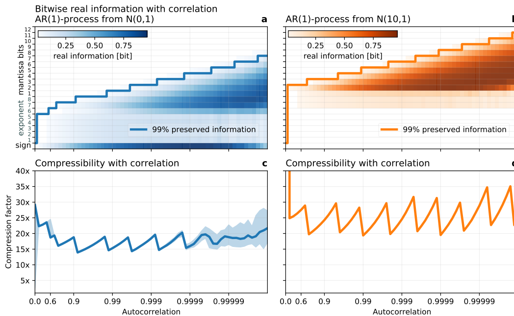
Figure 3.2 | Dependency of the bitwise real information and compressibility on correlation. a The bitwise real information content of a first-order autoregressive process (AR(1) with Gaussian distribution N(0,1) , i.e. with zero mean and unit variance) with varying lag-1 autocorrelation. The bits that have to be retained to preserve 99% of information are enclosed with a solid line. b as a but the AR(1) process follows a Gaussian distribution with a mean of 10. c,d Compression factors for a,b when preserving 99% of information. Shading denotes the interdecile range.
