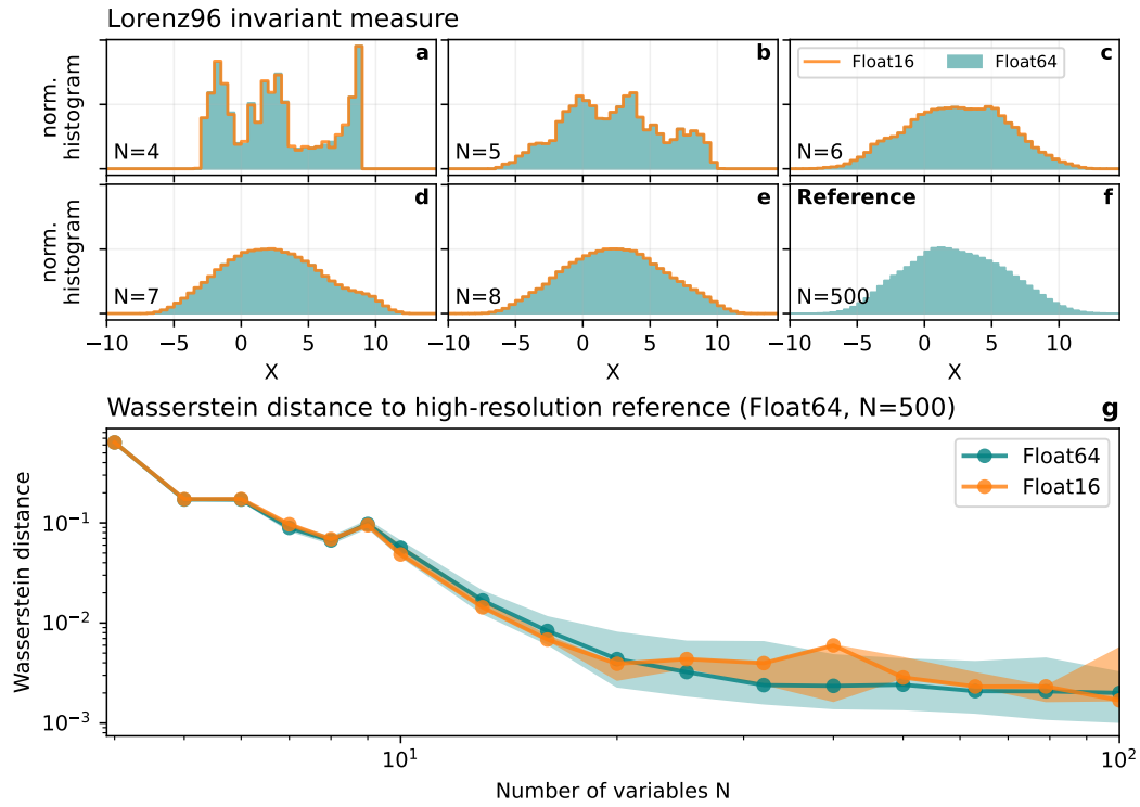
Figure 4.10 | Improvement of the simulated Lorenz 1996 invariant measure with increasing number of variables. a The invariant measure of Lorenz 1996 simulated with 4 variables. Using Float16 or Float64 arithmetic yields a virtually identical invariant measure. b-e as a but with an increasing number of variables. f The reference invariant measure obtained from 500 variables using Float64 arithmetic. g The Wasserstein distance of the simulated Lorenz 1996 system with respect to the reference. Invariant measures are taken from all available variables, which are invariant due to periodic boundary conditions and spatially-independent forcing (see Eq. 4.4). Shadings in g represent the 5-95% confidence interval and solid lines the median obtained from an ensemble simulation with 51 members starting from slightly perturbed random initial conditions.
