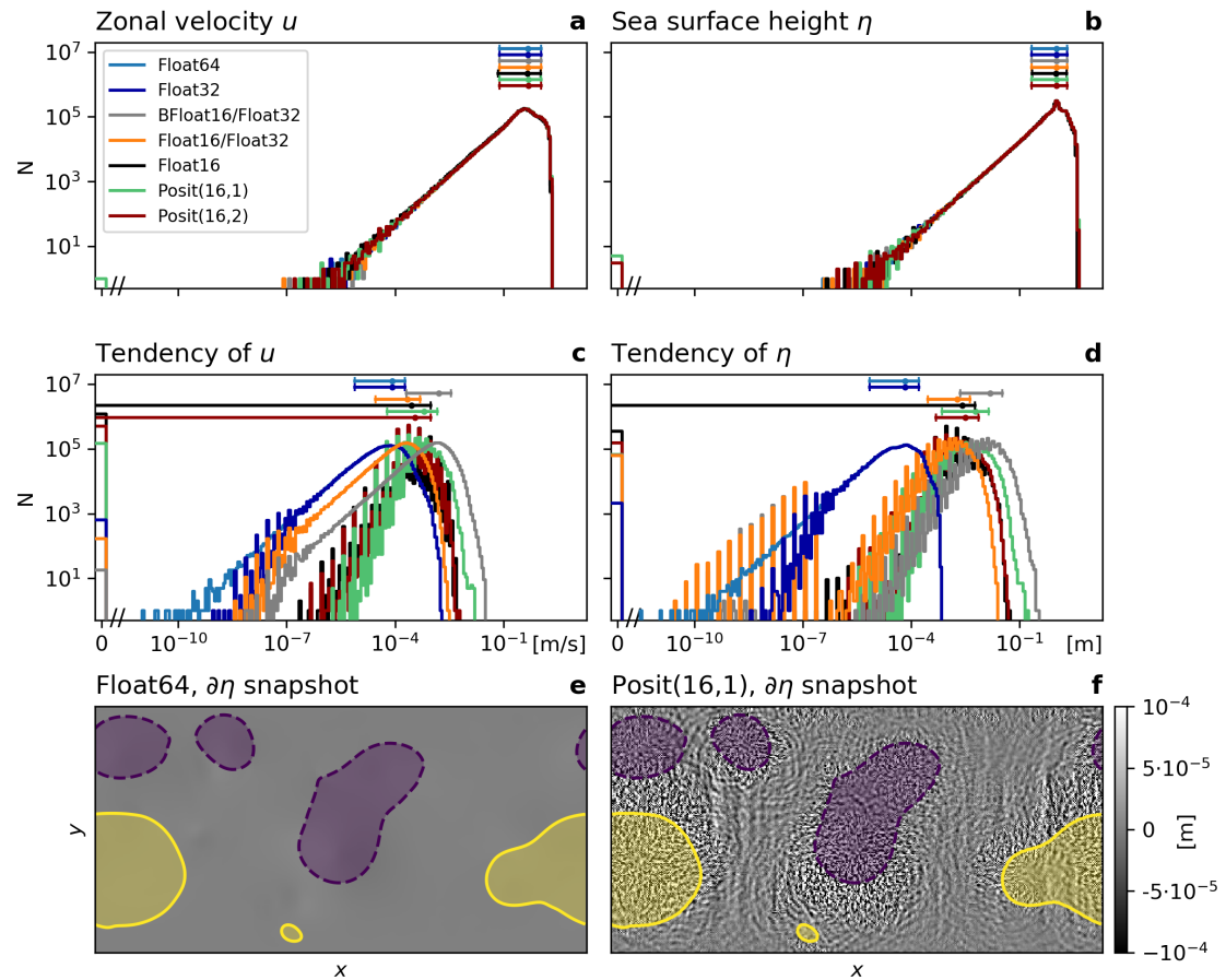
Figure 5.6 | Detecting gravity waves due to rounding errors from low precision. Histograms of the numeric values of the prognostic variables a zonal velocity u , b sea surface height \eta , and the respective tendencies of c u and d \eta , simulated with different 16, 32 and 64-bit number formats. Mean, 10th and 90th percentile are shown above the histograms in respective colours. Snapshots of the tendencies of \eta simulated with e Float64 and f Posit(16,1). Snapshots are similar for other 16-bit formats (not shown here). Areas of sea surface height anomalies exceeding \pm 1.4 m are shown in purple (negative) and yellow (positive). Note the break on the x-axis close to zero in a-d .
