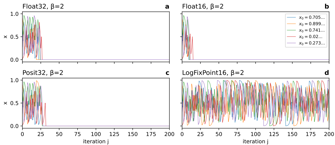
Figure 4.2 | The Bernoulli map simulated with different number formats. a Float32, b Float16, c Posit32, and d LogFixPoint16. The arithmetic operations in the Bernoulli map do not introduce rounding errors in a-c , only the initial conditions are subject to rounding, causing the attractor to collapse after a few iterations. However, the subtraction in the Bernoulli map causes rounding errors with logfix arithmetic in d that prevent the stalling at 0 from a-c .
