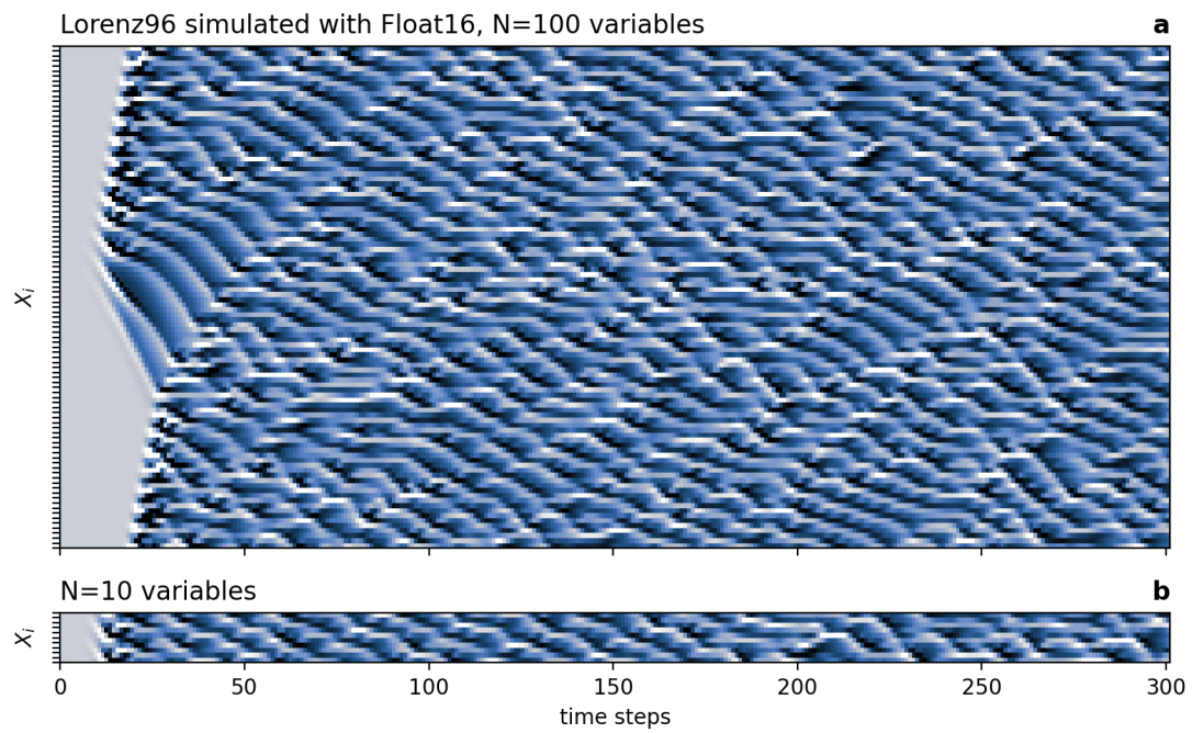
Figure 4.8 | The Lorenz 1996 system simulated with Float16 arithmetic. a 100 variables are used, starting from equilibrium with a small perturbation in X_{50} , and b 10 variables starting with a small perturbation in X_5 . Rectangles visible in shading represent individual variables and time step.
