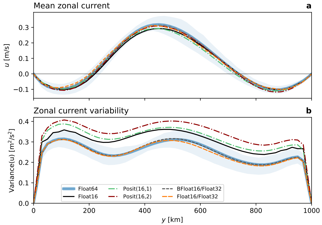
Figure 5.4 | Climatology and variability of the zonal current in the medium-resolution simulations. a Zonally-averaged zonal current u as a function of the meridional coordinate y . b Zonal variance of the zonal current as a function of y . The dashed lines for BFloat16/Float32 and Float16/Float32 are almost identical. The shaded area denotes the interquartile temporal variability around the a mean and b variance of reference simulations with Float64.
