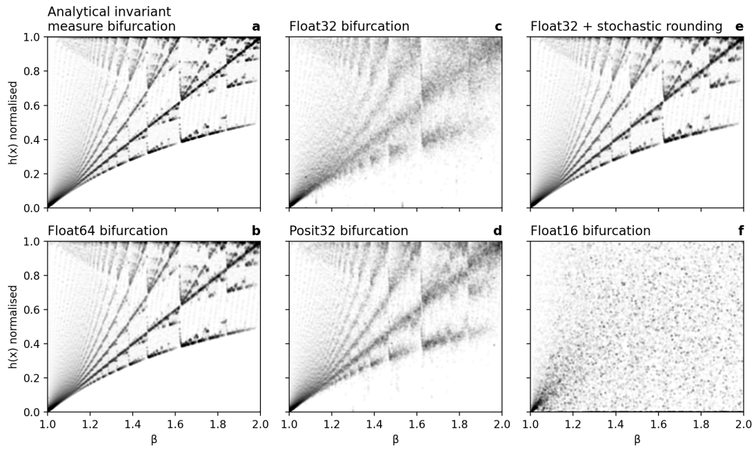
Figure 4.4 | Bifurcation of the quantization levels corresponding to the invariant measures in the generalised Bernoulli map as simulated with various number formats. a Analytical bifurcation h_\beta(x) from the exact invariant measure, normalised by \max(h_\beta(x)) , compared to the invariant measure by simulating the Bernoulli map with b Float64, c Float32, d Posit32, e Float32 and stochastic rounding, and f Float16.
