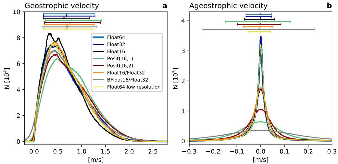
Figure 5.5 | Geostrophic balance as simulated with different number formats. a Histograms of flow-parallel components of geostrophic velocity. b as (a) but for the ageostrophic velocities, as defined by Eq. 5.6. Horizontal bars denote the mean, 10th and 90th-percentile in respective colours.
