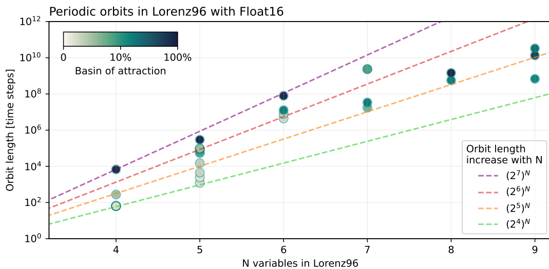
Figure 4.9 | Periodic orbits in Lorenz96 simulated with Float16 and an increasing number of variables. Initial conditions are randomly taken from a spin-up simulation. Size of the basins of attraction (shading) correspond to the share of initial conditions that converge to the respective periodic orbit. Dashed lines provide an orientation for the exponential increase in orbit lengths with the number of variables.
