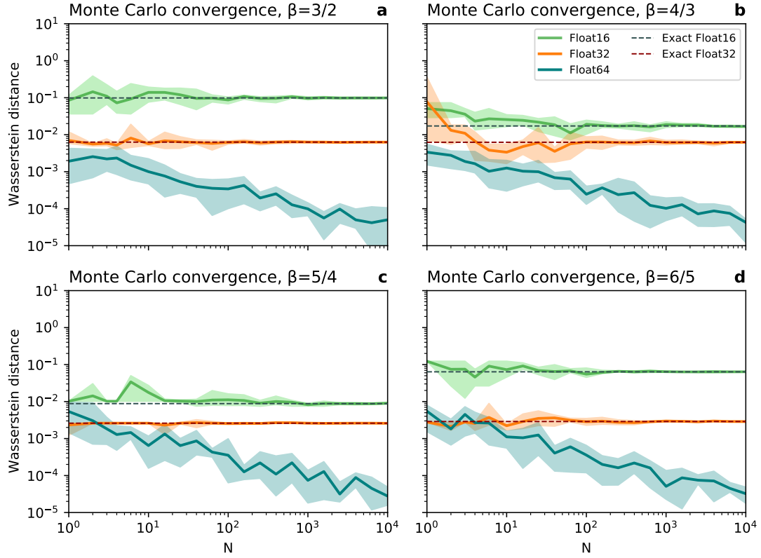
Figure 4.1 | Convergence of the Monte Carlo sampling to estimate invariant measures. The agreement between the analytical and simulated invariant measures (Figure 4.3) from N random initial conditions uniformly distributed in [0, 1) are assessed with the Wasserstein distance (section 4.2.4). About N = 1000 random initial conditions allow for a robust estimate of the invariant measure with Float16 and Float32, virtually identical with exact invariant measure obtained from computing all 15,360 Float16 and 1,065,353,216 Float32 numbers in [0, 1) , respectively. The \beta parameter of the generalised Bernoulli map is a \beta = \frac{3}{2} , b \beta = \frac{4}{3} , c \beta = \frac{5}{4} , and d \beta = \frac{6}{5} . Solid lines represent the mean and shading the min-max range.
