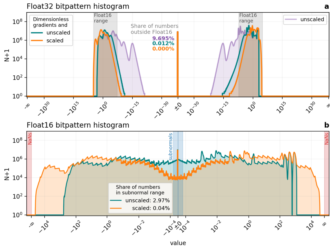
Figure 6.2 | Bitpattern histogram of all arithmetic results in ShallowWaters.jl. a 200-day simulation at \Delta x = 20 km based on Float32 arithmetic. The share of numbers outside the Float16 range (grey shading) are colour-coded to the respective histograms. b as a but based on Float16. Bitpattern histograms are created with Sherlogs.jl. The logarithmic y-axis denotes the number of occurrences N of the respective bitpattern during the simulation. The histograms span all available bitpatterns (0x0000 to 0xffff in hexadecimal) in the respective formats evenly but are sorted and relabelled with the corresponding values for readability. The range of bitpatterns that are subnormals or interpreted as Not-A-Number (NaN) are marked. Bitpatterns histograms are without compensated time integration.
