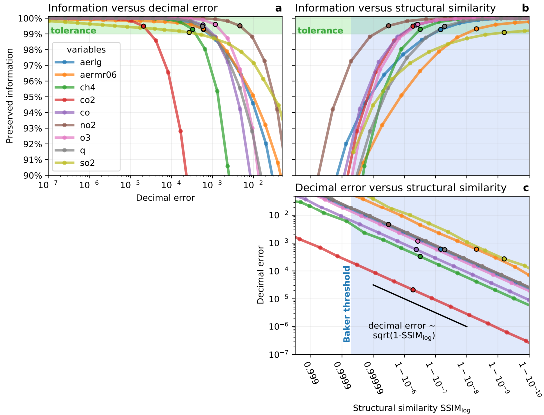
Figure 3.4 | The relationships between preserved information, decimal error and structural similarity for rounding within the information-preserving compression. a The last 1% of information tends to be distributed across many mantissa bits such that a trade-off arises where a large increase in compressibility is achieved for a small tolerance in information loss. The preserved information is presented as a function of the decimal error, which itself increases exponentially for every additional bit (small circles) that is discarded due to rounding. Denoted circles present the number of mantissa bits that have to be retained during compression to preserve at least 99% of information. b The preserved information increases as a function of the structural similarity (SSIM, Wang et al. [2004]). The proposed threshold for climate data of SSIM=0.99995 by Baker et al. [2019] is shaded. All variables are very close or above the Baker threshold when preserving 99% of information. c The decimal error is proportional to the square root of the structural dissimilarity 1-SSIM for binary rounding within the information-preserving compression
