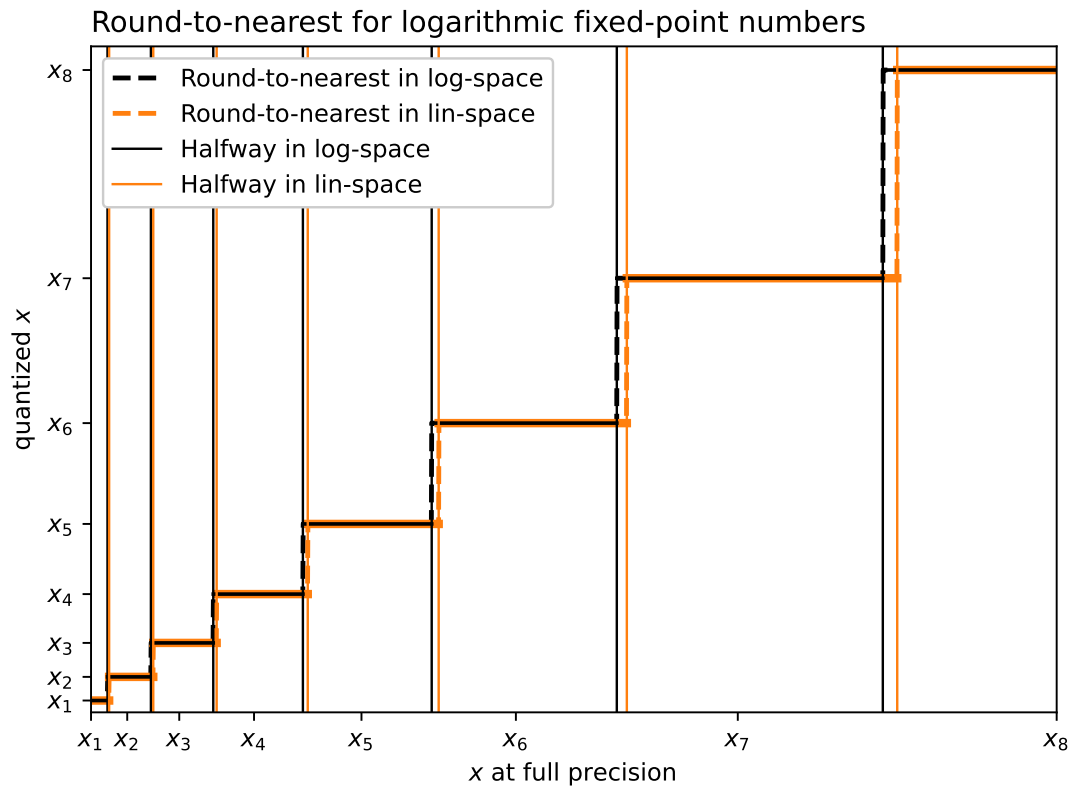
Figure 2.3 | Schematic to illustrate round-to-nearest in linear and logarithmic space for logarithmic fixed-point numbers. Exact values x at full precision are presented on the x-axis and their rounding to the logarithmically spaced representable numbers x_1, \dots, x_8 on the y-axis. Round-to-nearest in linear space will use the midpoints \frac{x_i + x_{i+1}}{2} (arithmetic mean) as ties, round-to-nearest in logarithmic space uses the geometric mean \sqrt{x_i x_{i+1}} .
