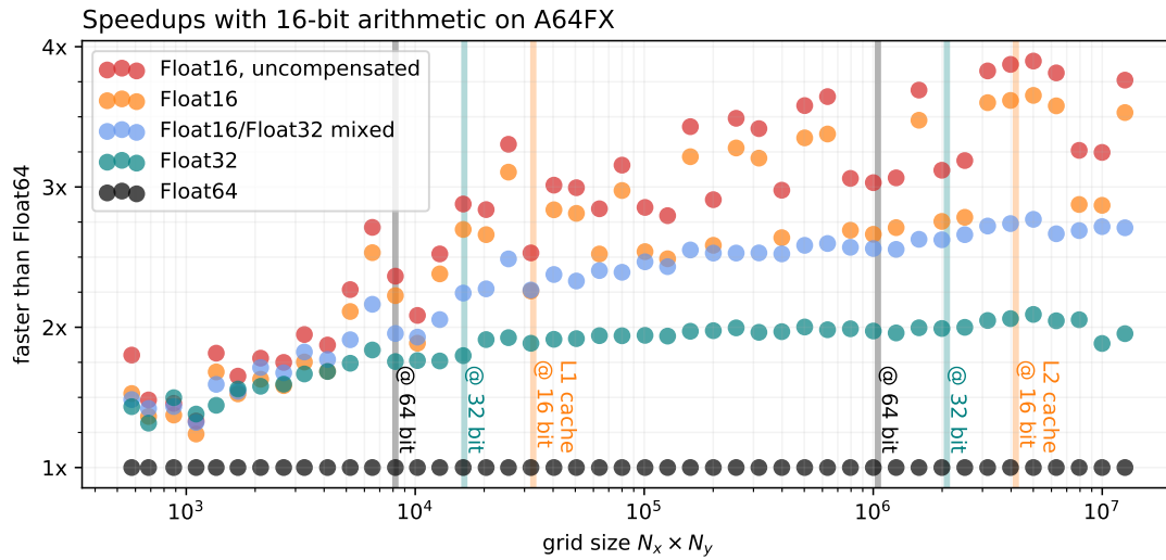
Figure 6.6 | Performance increase from Float16 when running ShallowWaters.jl at varying grid sizes on A64FX. The grid size is the total number of grid points N_x \times N_y . All timings are single-threaded median wall clock times relative to Float64, excluding compilation, model initialisation and memory pre-allocation. The corresponding size of the L1 and L2 cache (64KiB, 8 MiB) of A64FX is given as vertical lines for arrays of 16, 32 and 64-bit floats.
