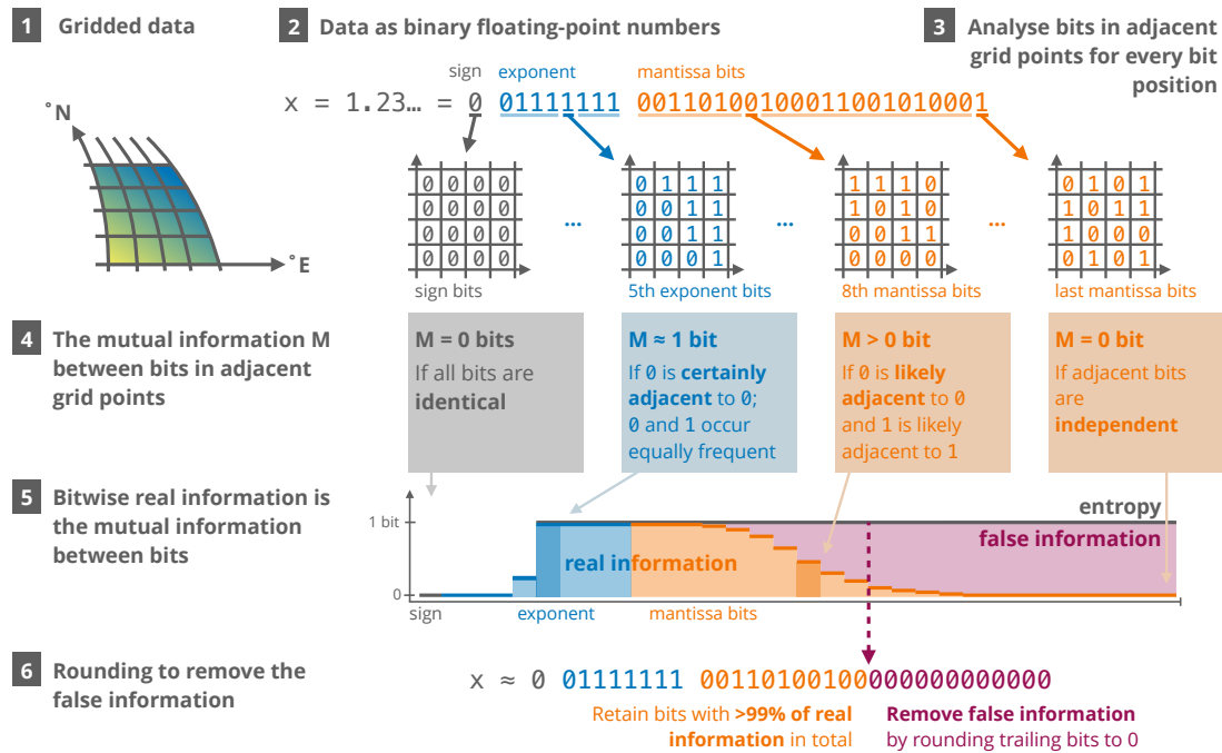
Figure 3.9 | The bitwise real information content is defined as the mutual information of bits in adjacent grid points. A bit contains more real information the stronger the statistical dependence to the adjacent bits is. Independent bits contain only false information and are rounded to 0 to facilitate lossless compression.
