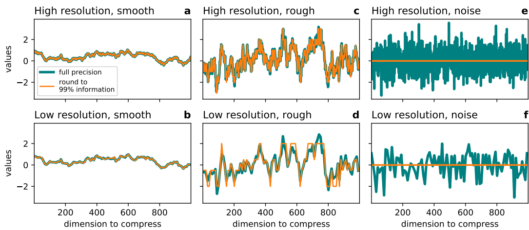
Figure 3.1 | Resolution and smoothness dependence of the information-preserving compression. a,b Highly autocorrelated data (1st order auto-regressive process with correlation r = 0.999 ) will have many mantissa bits preserved, at high and low resolution. c,d Many mantissa bits in data with less auto-correlation ( r = 0.95 ) will be independent at low resolution and therefore rounded to zero. e,f All bits in random data ( r = 0 ) drawn from a standard normal distribution are fully independent so that removing the false information rounds this data to zero. Low resolution data ( b,d,f ) is obtained from high resolution ( a,c,e ) by subsampling every 10th data point.
