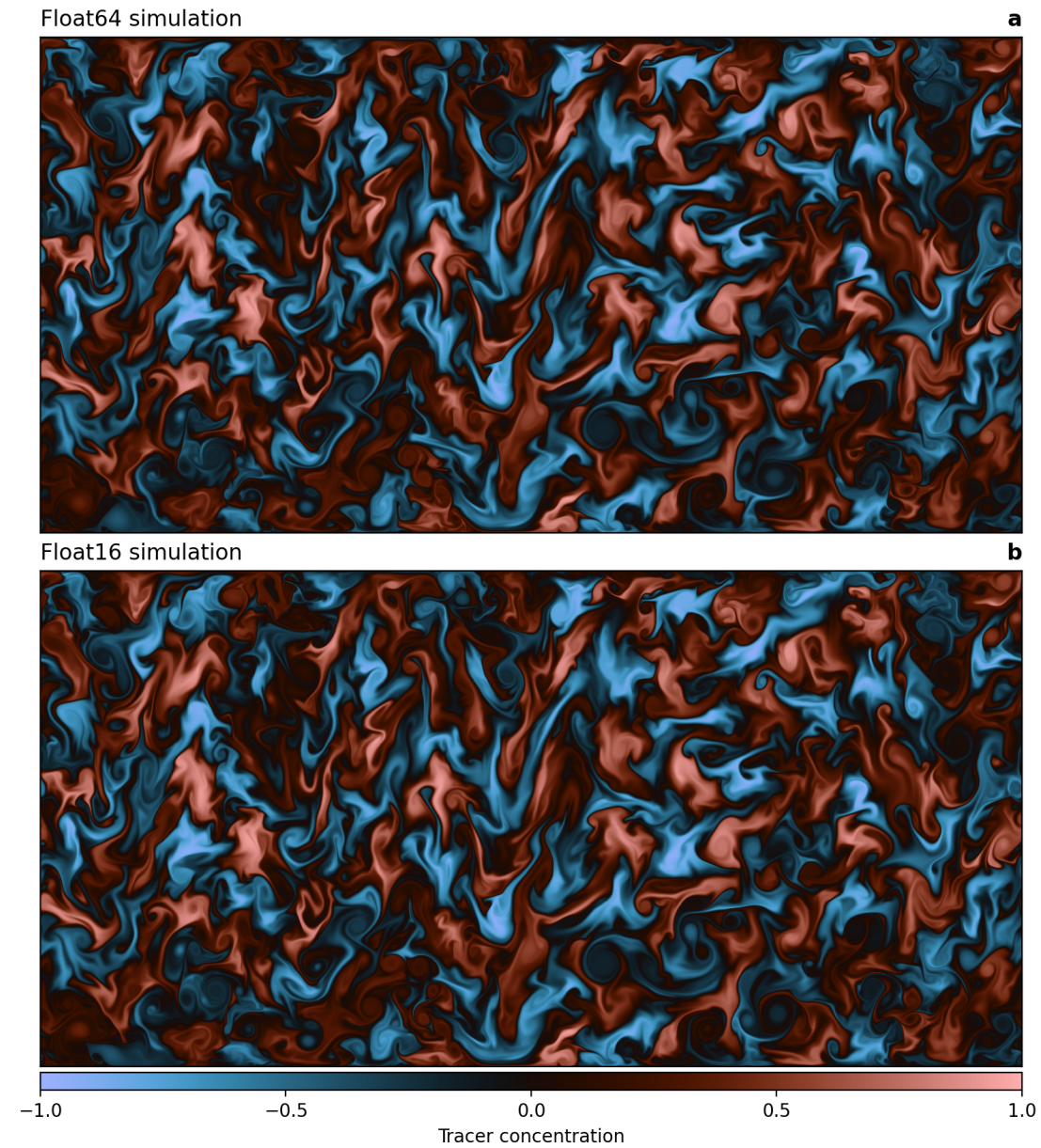
Figure 6.4 | Turbulent tracer mixing as simulated by ShallowWaters.jl. a Simulation based on Float64 arithmetic and b Float16 with compensated time integration. Snapshot is taken after 100 days of simulation (about 25,000 time steps) with 3000x1500 grid points starting from identical initial conditions. Remaining errors between a and b from low-precision Float16 are tolerable and will be masked by other sources of error in a less idealised model setup.
