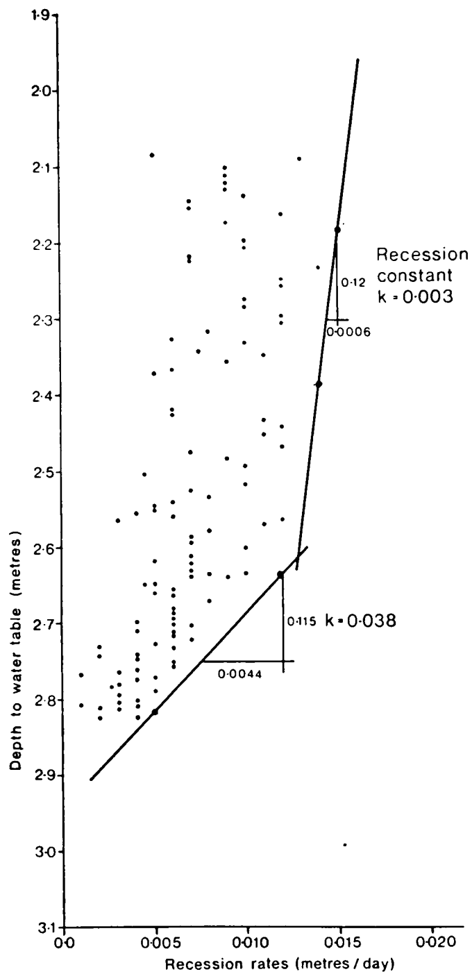
Fig. 9.12 Rates of groundwater level recession, (summer 1980) for borehole R/8.
