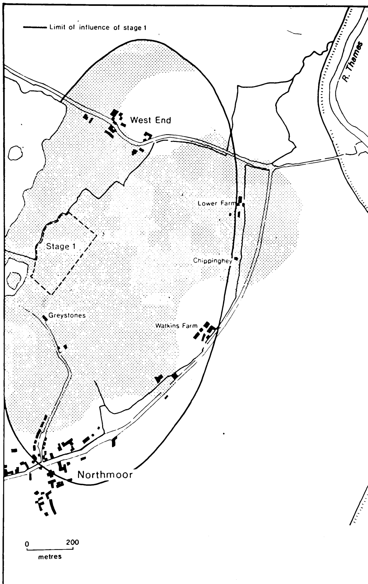
Fig 10.50 Area around Watkins Farm that will not benefit from the water-table during dewatering of stage 1 (based on min. water-table conditions).
