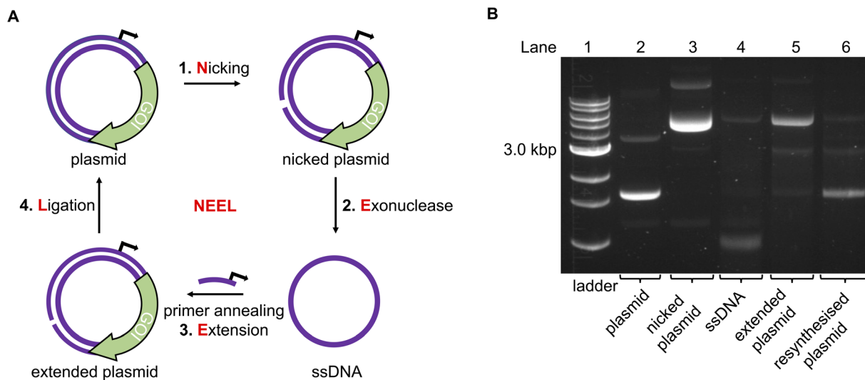
Fig. 2 The NEEL method to resynthesise a plasmid. (A) Overview of the enzymatic reactions in NEEL. (B) Using NEEL, our plasmid encoding mVenus was successfully resynthesised.
