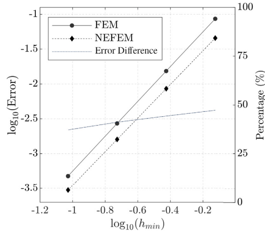
Fig. 7. Linear elastic problem: L^2(\Omega) error for FEM and NEFEM as a function of the minimum element size.
