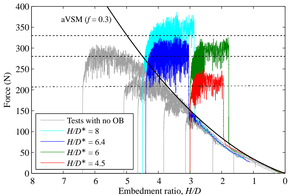
Figure 3-34 Force-disp. curves for OB tests shown at actual embedment vs. normal dry tests in RH110
