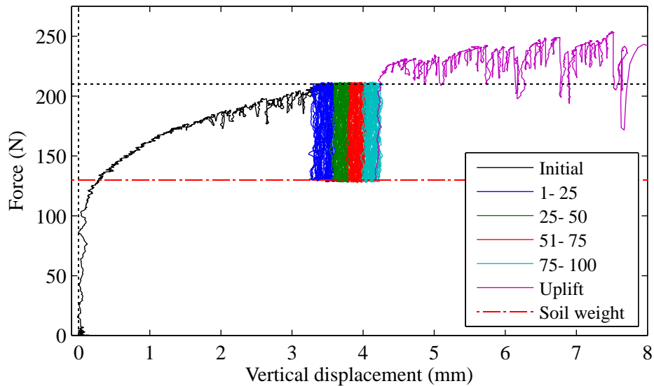
Figure 5-20 Force-displacement response cycling from 130-210 N at H/D = 4.5 (test: D-4)
