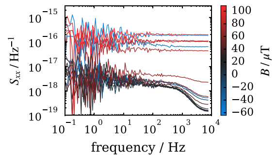
FIG. 4. The spectral density of the fractional frequency time series data from the 161 MHz resonator. The color scale corresponds to the magnetic field ( B_a + B_m ). To more clearly show the trend at low frequencies, the lowest 15 harmonics of the 1.412 Hz pulse tube cooler frequency have been masked in all of the spectra. The color bar is the same as Figure 2.
