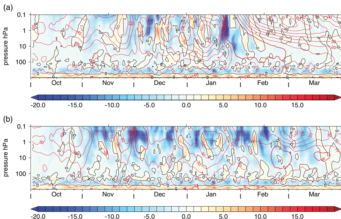
FIGURE 1 Time-series (2008–2009)/pressure (hPa) of zonally averaged zonal winds at 60°N (red contours; \text{m}\cdot\text{s}^{-1} ; thick contour indicates the zero-wind contour) and E-P flux divergence (shaded; \text{m}\cdot\text{s}^{-1}\cdot\text{day}^{-1} ) averaged over 45–75°N from (a) the successful (AllTrop-UpStrat-Eq) simulation in which the zonal winds were relaxed in the upper equatorial stratosphere as well as in the troposphere, and (b) the unsuccessful (AllTrop) simulation in which the zonal winds were relaxed only in the troposphere [Colour figure can be viewed at wileyonlinelibrary.com ]
