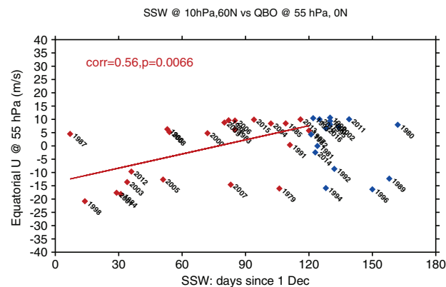
FIGURE 9 As Figure 8 but showing the relationship between SSW date (since 1 December) and amplitude of the QBO ( \text{m s}^{-1} ) at 0^\circ\text{N} , 55 hPa [Colour figure can be viewed at wileyonlinelibrary.com ]
