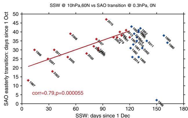
FIGURE 8 Scatter plot showing relationship between the date at which the ERA-I zonally averaged zonal winds at 60°N, 10 hPa reverses to easterly, indicating an SSW (x-axis; days since 1 December) and the date at which the equatorial zonally averaged zonal winds reverse to easterly at 0.29 hPa after 1 October, indicating the transition from westerly-to-easterly SAO phase (y-axis; days since 1 October). Red squares show SSWs in DJFM, blue squares show final warmings in April/May. The year associated with each square is the year at the start of winter for example, 1987 denotes the winter of 1987/1988. Red line shows the line of best fit to the red (mid-winter) SSW years, and the associated rank correlation and statistical significance is also shown. Three winters (1984/1985, 1986/1987 and 1988/1989) have been excluded due to unrealistic early SAO transitions [Colour figure can be viewed at wileyonlinelibrary.com ]
