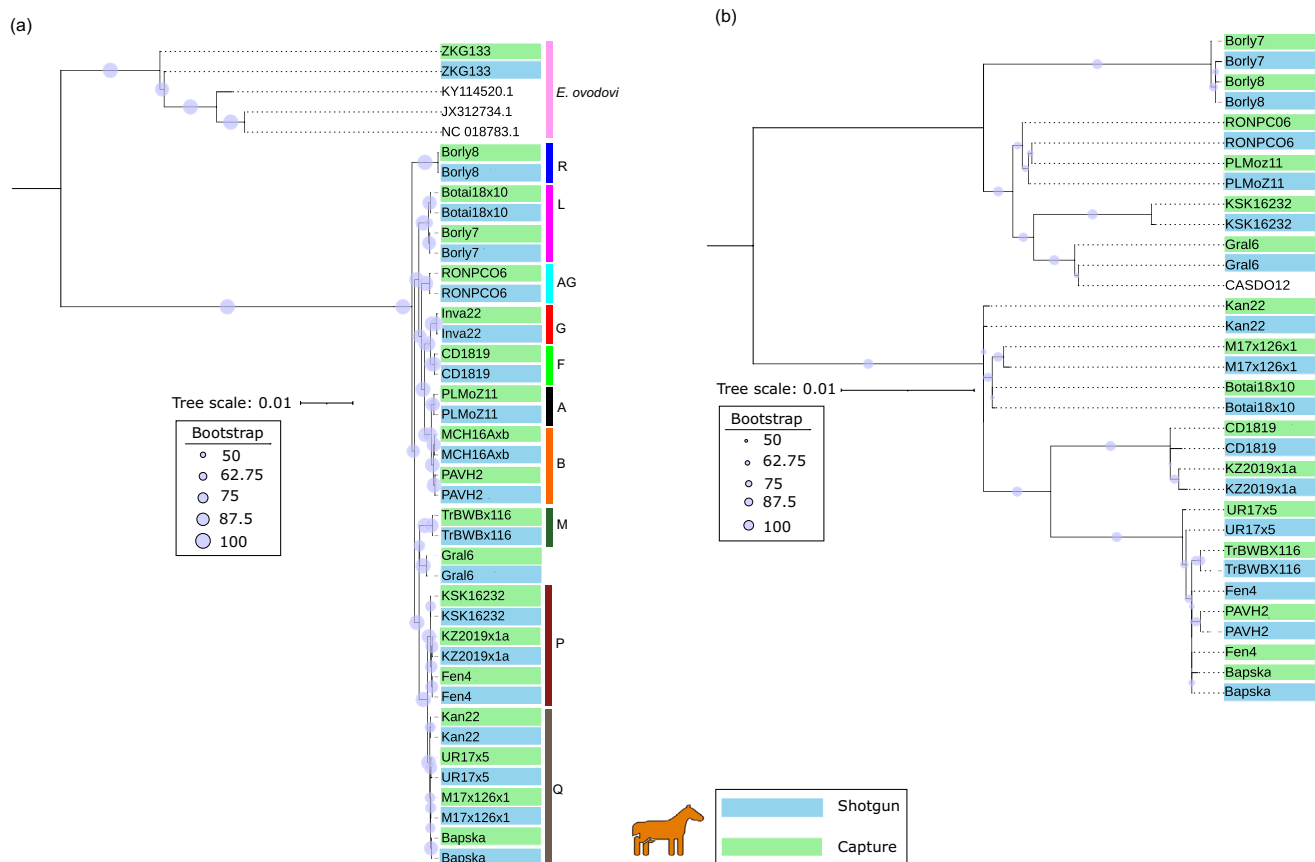
FIGURE 2 | IQ-TREE maximum likelihood (ML) phylogenetic reconstructions. (a) Mitochondrial and (b) Y chromosomal sequences recovered from shotgun and captured samples occupied identical phylogenetic placements on the Equus caballus phylogenetic tree (each coloured bar indicates an individual haplogroup).
