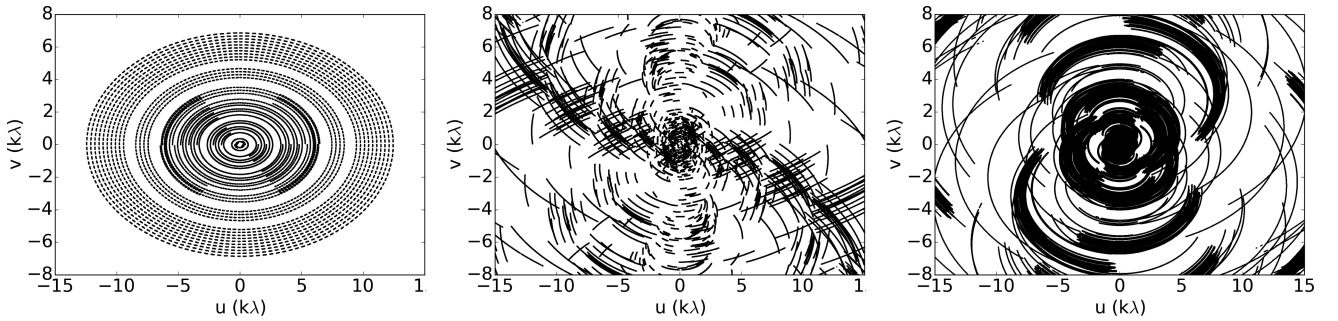
Figure 2. The monochromatic uv -coverage of the 1.4 GHz WSRT (left), 610 MHz GMRT (centre) and 150 MHz LOFAR (right) observations of Abell 2034. This figure shows the entire WSRT uv -coverage but the GMRT and LOFAR coverage extends to 53k\lambda and 60k\lambda , respectively. Here the monochromatic coverage has been presented for display purposes but the full bandwidth used in each observation (160 MHz for WSRT, 32 MHz for GMRT and 48 MHz for LOFAR) provides considerable additional filling of the uv -plane.
