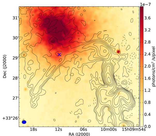
Figure 9. Contours from a medium-resolution (12 arcsec \times 10 arcsec) LOFAR image of Abell 2034 overlaid on a high-resolution Chandra image (pixels of 1.968 arcsec) which has been smoothed with a Gaussian kernel of FWHM = 6 arcsec. The Chandra image is the same as that in Fig. 3 and the radio image is the same as that in Fig. 1. The cross shows the position of BCG1.
