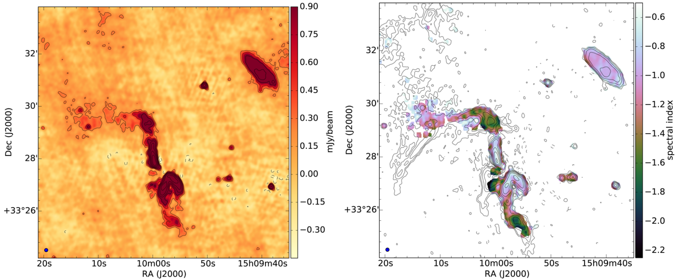
Figure 5. The 150 MHz to 610 MHz high-resolution ( 7.8 \text{ arcsec} \times 7.8 \text{ arcsec} ) spectral properties of the emission from Abell 2034. Left: the 610 MHz GMRT image with contours at (1, 2, 4, \dots) \times 3 \times \sigma_{\text{GMRT}, 8 \text{ arcsec}} where \sigma_{\text{GMRT}, 8 \text{ arcsec}} = 90 \mu\text{Jy beam}^{-1} . Right: the 150–610 MHz high-resolution spectral index image where pixels with errors greater than 0.3 have been blanked. The contours show a high-resolution ( 7.8 \text{ arcsec} \times 7.8 \text{ arcsec} ) 150 MHz LOFAR image with levels at (1, 2, 4, \dots) \times 3 \times \sigma_{\text{LOFAR}, 8 \text{ arcsec}} where \sigma_{\text{LOFAR}, 8 \text{ arcsec}} = 185 \mu\text{Jy beam}^{-1} . In both the 610 and 150 MHz images, the uv -range ( 102\lambda to 52.8k\lambda ) is the same and the maximum recoverable scale is \approx 20 \text{ arcmin} which is sufficient to not resolve out any of the cluster emission but the resolution is high and the flux per pixel of the very low surface brightness structures is too low to be detected at high significance. The procedure for creating the GMRT and LOFAR images is outlined in Section 2.2.
