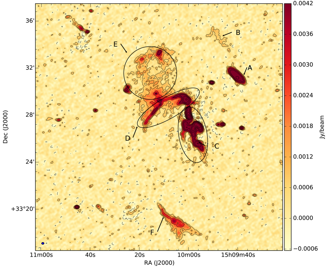
Figure 1. A medium-resolution ( 12 \text{ arcsec} \times 10 \text{ arcsec} ) 118–166 MHz Stokes I image towards Abell 2034 with six regions of interest highlighted. The LOFAR contours show the (1, 2, 4, \dots) \times 3 \times \sigma_{\text{LOFAR}, 10 \text{ arcsec}} levels where \sigma_{\text{LOFAR}, 10 \text{ arcsec}} = 210 \mu\text{Jy beam}^{-1} .
