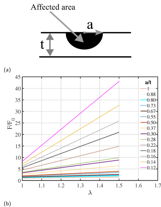
Fig. 6 (a) Kinematics for the cases where a \ll t in the small strain regime (b) evolution of F/F_0 at small stretch for a \ll t and various a/t values as predicted from eqn (5) and (7).
