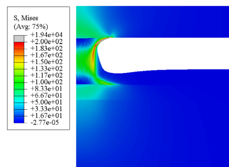
(a) von Mises stress distribution
