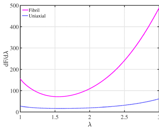
Fig. 8 Slope of force against stretch: Arruda–Boyce, a/t = 2.2 , \lambda_L = 2 , b = 10 mm: It gives an explanation of the positive slope in F/F_0 curve for aspect ratio: a/t = 2.2 starting from \lambda = 2 .
