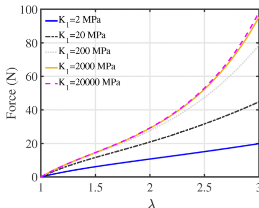
Fig. 11 Effect of change in bulk modulus on the force required to pull the fibril: Arruda–Boyce, a/t = 1 , b = 10 mm, \mu = 1 MPa, \lambda_L = 2 .
