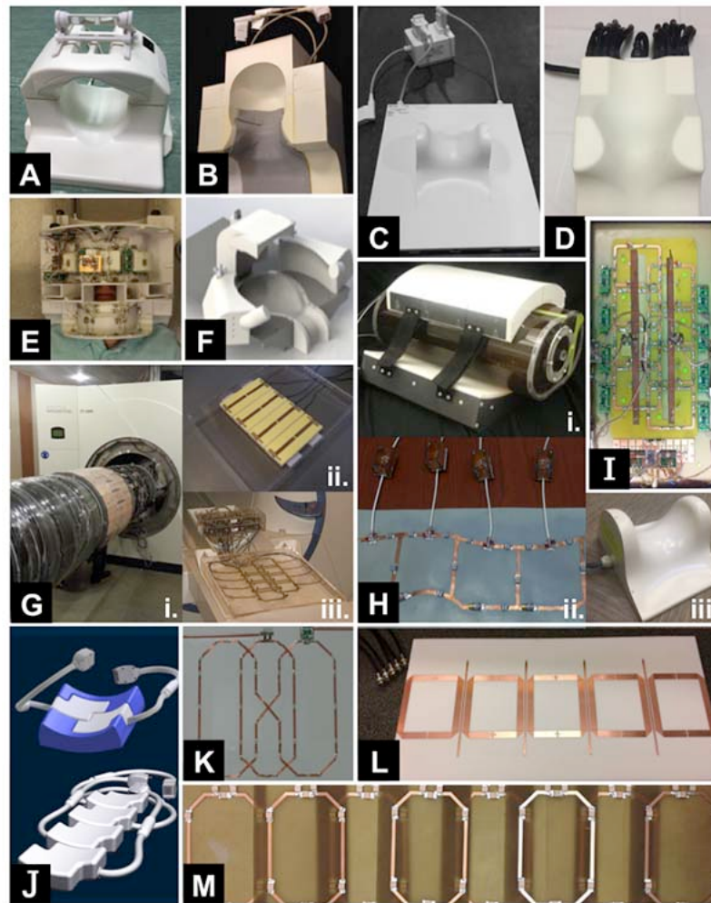
Figure 2: Montage of coils for human spinal cord MRI at 7T.
