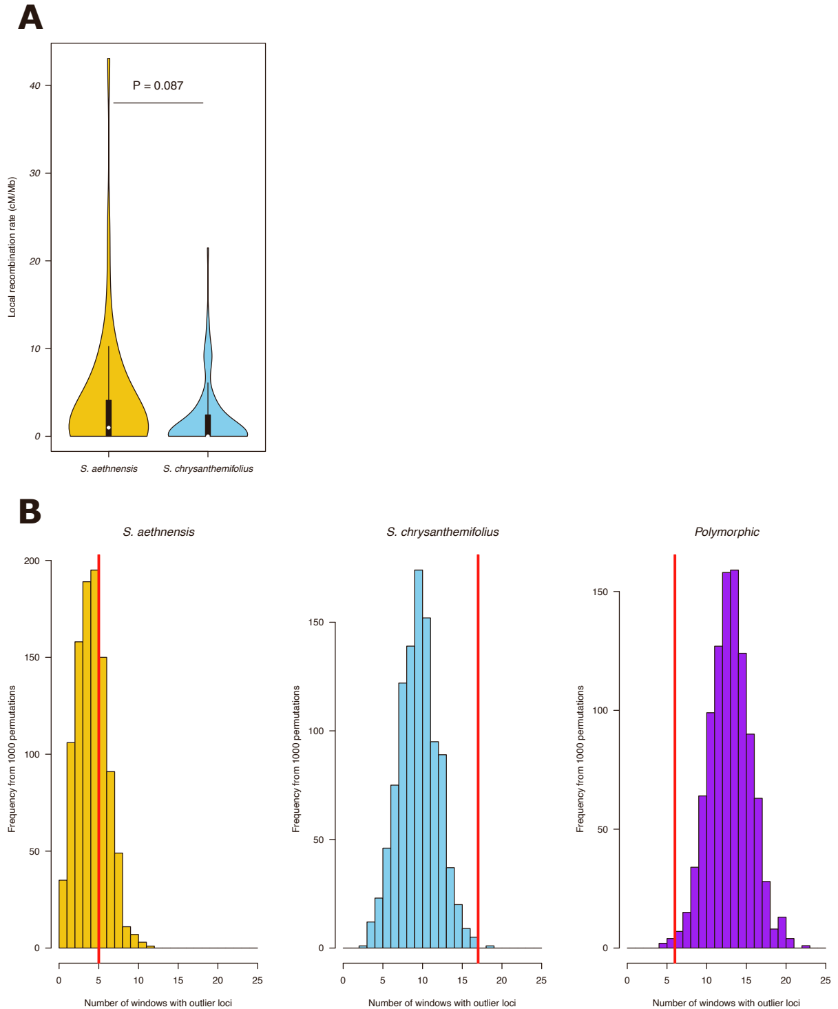
Figure S7: Parental ancestry, recombination rates and natural selection in S. squalidus . Related to Figure 4. (A) Local recombination rate in genomic regions with different parental ancestry. Regions with minor parent ancestry (i.e. S. aethnensis ) exhibit higher recombination rates, but the difference is not significant ( P values from Welch two sample t-test). (B) The number of genomic windows that have at least 1 outlier locus found to be under divergent selection in parental species on Mount Etna, according to the parental ancestry. Shown are the results for 1000 permutations of outlier loci over all genomic windows with known parental ancestry (i.e., excluding genomic windows without diagnostic SNPs or with mixed ancestry from both parental species). For each graph, red vertical line denotes the number of genomic windows with at least 1 outlier locus observed in the real data.
