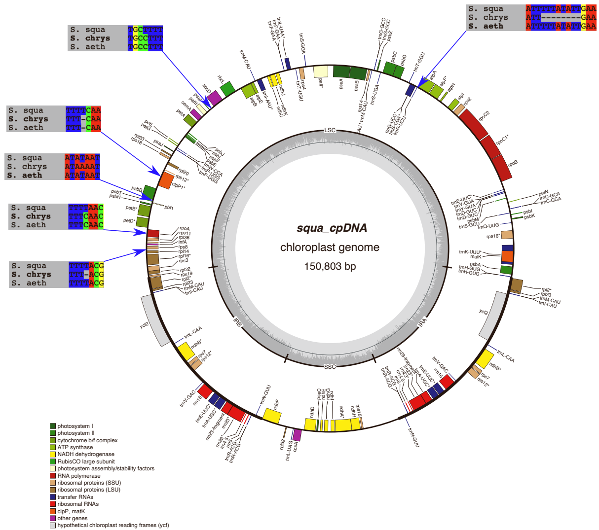
Figure S1: Complete chloroplast genome of S. squalidus . Related to Figure 2. Genes annotated in the genome are labelled and color-coded according to function. Genes inside circle are transcribed clockwise, outside circle transcribed counterclockwise. Dark and light grey bars in inner circle denote percentage GC (dark) and AT (light) content. Insets depict the six differences detected across the three species, with the corresponding alleles found in S. squalidus ( S. squa ), S. chrysanthemifolius ( S. chrys ) and S. aethnensis ( S. aeth ).
