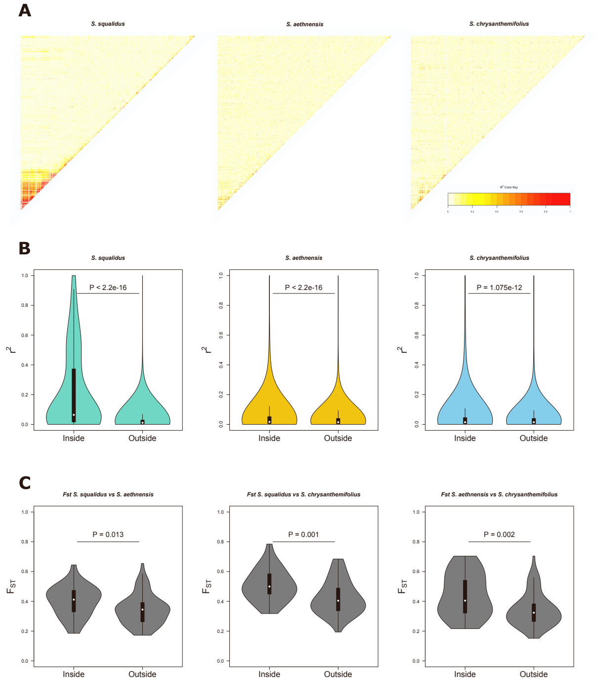
Figure S3: Linkage disequilibrium and pairwise F_{ST} values inside vs outside the first 15 Mb of chromosome 4. Related to Figure 4. (A) Pairwise linkage disequilibrium between pairs of SNPs estimated along chromosome 4 for S. squalidus (left), S. aethnensis (middle) and S. chrysanthemifolius (right). (B) Linkage Disequilibrium values inside and outside the first 15 Mb region of chromosome 4 for S. squalidus (left), S. aethnensis (centre) and S. chrysanthemifolius (right). P-values refer to Welch two sample t-test results, for LD between pairs of SNPs in chromosome 4, inside vs outside the first 15 MB region. (C) F_{ST} values between pairs of species (left to right: S. squalidus vs S. aethnensis , S. squalidus vs S. chrysanthemifolius , and S. aethnensis vs S. chrysanthemifolius ) inside and outside this 15 Mb region of chromosome 4. P-values refer to Welch two sample t-test results, for pairwise F_{ST} values estimated in sliding windows of 500 kb, along chromosome 4. For panels B and C, black boxplots indicate the median (white dot), the quartiles (black rectangle), 1.5 times the interquartile range (whiskers), and the kernel probability density (shaded area).
