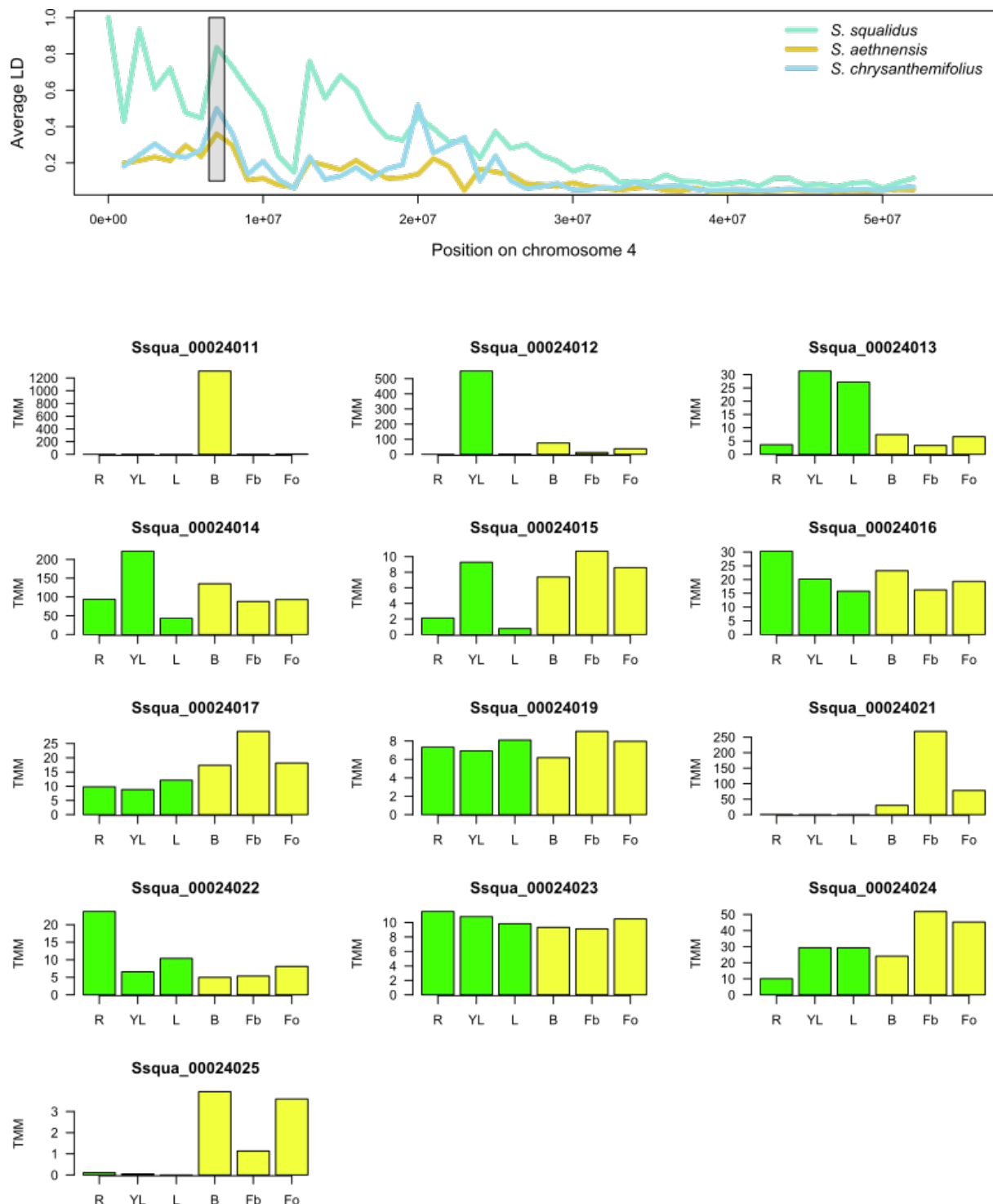
Figure S4: Putative location of the self-incompatibility ( S )-locus on chromosome 4 of S. squalidus . Related to Figure 4. Top panel shows average linkage disequilibrium (LD) between SNPs within 1 Mb windows along chromosome 4, for S. squalidus and the two parental species S. aethnensis and S. chrysanthemifolius . Rectangle highlights the single window (7-8 Mb) with elevated LD in all three species. Bottom inset shows the gene expression estimates of genes annotated in this window, across floral (yellow) and non-floral (green) plant tissues in S. squalidus (R: root, YL: young leaf; L: leaf; B: capitulum bud; Fb: flower buds; Fo: whole open flower).
