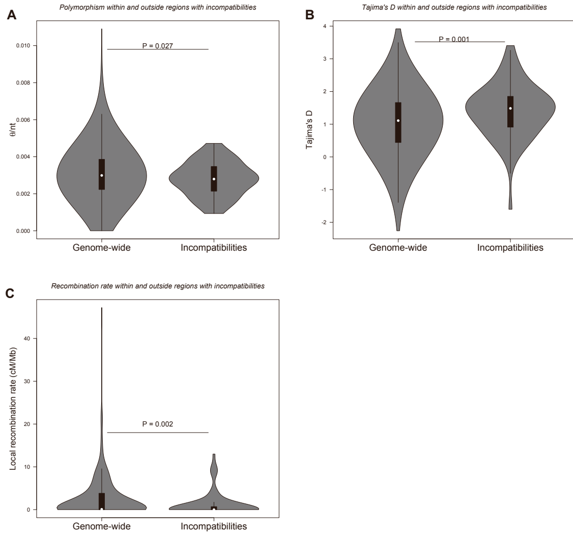
Figure S6: Comparison of summary statistics estimated from windows harbouring genetic incompatibilities vs genome-wide background. Related to Figure 4. Estimates of (A) Watterson's theta, (B) Tajima's D and (C) local recombination rates using non-overlapping windows (500 kb) along the newly assembled genome of S. squalidus and based on the population-level RNAseq data. For each panel, left-side distribution refers to values estimated genome-wide (excluding windows harbouring genetic incompatibilities), and right-side distribution values observed in windows harbouring genetic incompatibilities described in S1 between the two parental species of S. squalidus . Significance P values refer to Welch two sample t-tests in each panel.
