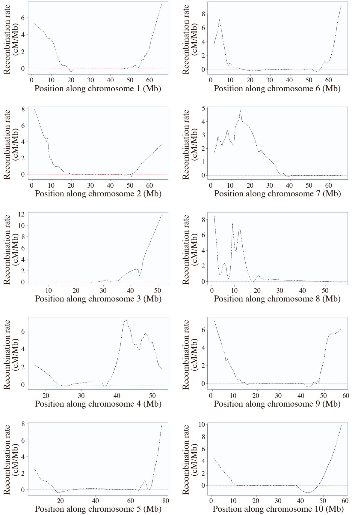
Figure S2. Local recombination rates estimated along each chromosome. Related to Figure 2. Results obtained using the genetic map of reference S1 . Note that axes vary between panels.
