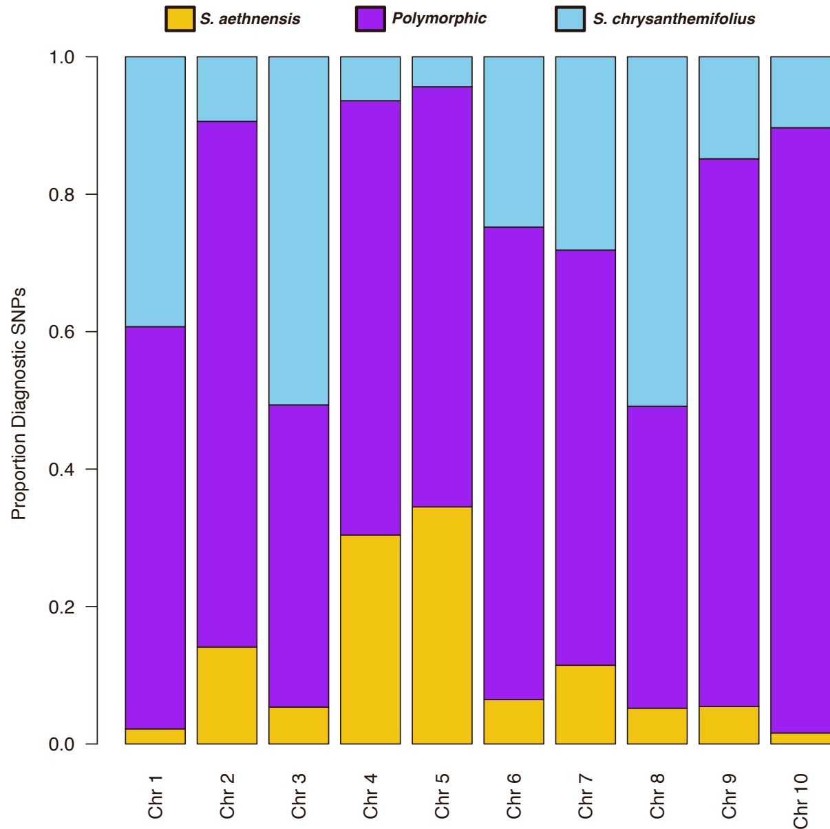
Figure S5. Proportion of diagnostic SNPs. Related to Figure 4. (i.e., SNPs that are fixed or nearly fixed for different alleles in the two parental species) sequenced in S. squalidus that are fixed or nearly fixed for either parental allele, or polymorphic for the two parental alleles (legend on top).
