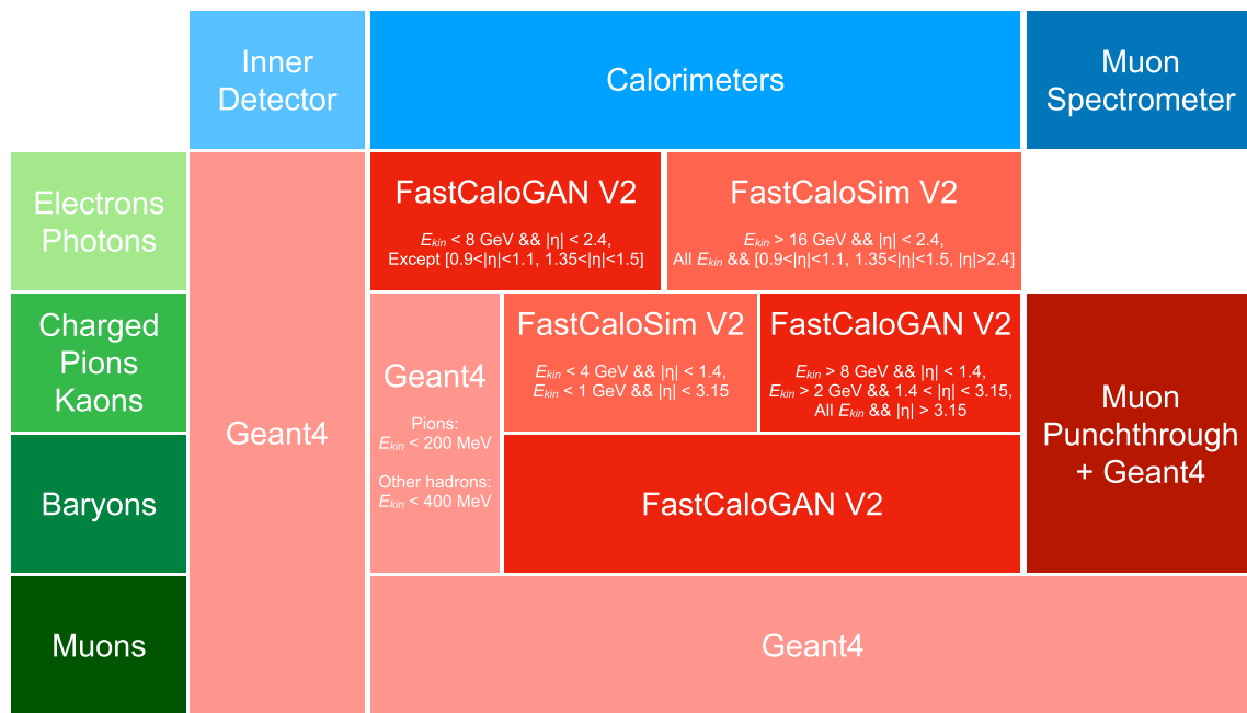
Fig. 9 The configuration of tools that together form ATLF3. The tools (GEANT4, FastCaloSimV2 and FastCaloGANV2) are combined in a way that the physics performance of ATLF3 is closest to
