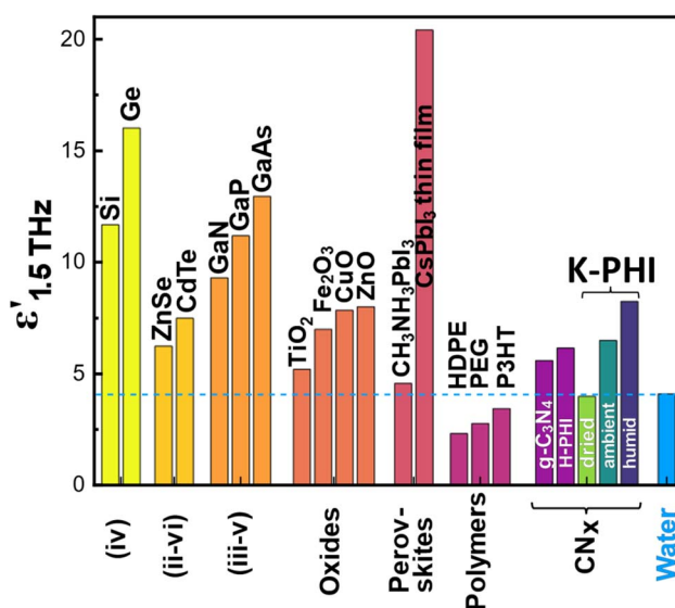
Fig. 4 Real permittivity at 1.5 THz ( \epsilon'_{1.5\text{THz}} ) for common semiconductor materials used for solar energy conversion applications, relative to measured CN x and water. 48–58
