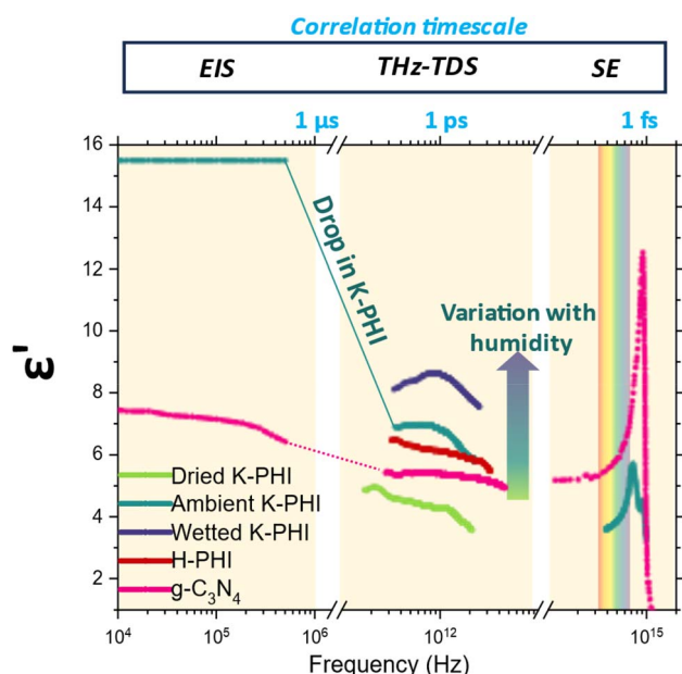
Fig. 5 Real permittivity comparison over the frequency spectrum for melon and K-PHI, with data extracted from Electrochemical Impedance Spectroscopy (EIS), THz (data from Fig. 2) and Spectroscopic Ellipsometry (SE) (literature values reproduced under CC by 4.0 license), 47,62,63 confirming the predicted dispersive trends in real permittivity (Fig. 1a).
