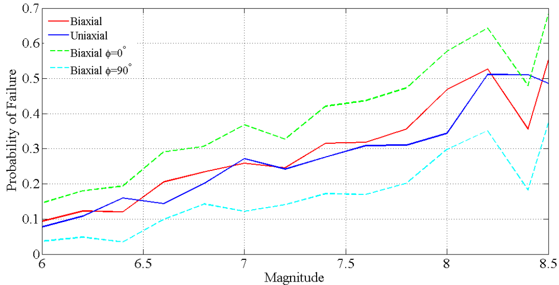
Fig. 9, where it can be seen that the probability of failure from the uniaxial method and the biaxial methods are both enveloped from the estimates of the biaxial method for angles \phi = 0^\circ and 90^\circ . An exception occurs near the maximum M_w of 8.5, which is to a point expected as the list of earthquakes used to calibrate both models of section 3 contains very few earthquakes with M_w > 8 and hence the results obtained in that region should be addressed with some skepticism.
