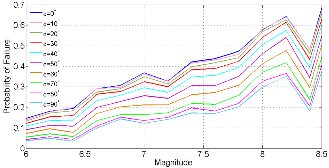
Fig. 7 – Probability of failure curves generated using the biaxial method for different values of \phi
