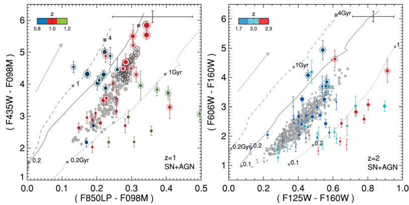
Figure 1. Colour comparisons of massive galaxies at z = 1 (left-hand panel; m_{\text{star}} \geq 10^{11} M_{\odot} ) and z = 2 (right-hand panel; m_{\text{star}} \gtrsim 10^{10.5} M_{\odot} ) with simulations that include AGN+SN feedback. The observed colours on the x -axis and y -axis trace rest frame (B - V) and (\text{NUV} - V) , respectively (see text for more details). Filled circles with error bars indicate the WFC3 ERS data, while simulated galaxies are shown using filled grey circles. The size of the symbol scales with stellar mass. The three lines represent the expected colours of SSPs with different ages at different redshift: in the left-hand panel, z = 0.8 (dashed), z = 1.0 (solid) and z = 1.2 (dotted), while in the right-hand panel, z = 1.7 (dashed), z = 2.0 (solid) and z = 2.3 (dotted). For clarity, the colours of SSPs with different ages (0.1, 0.2, 1 and 4 Gyr) are indicated by filled square symbols. Points with a concentric circle denote galaxies with low specific star formation rate ( \text{SSFR} < 0.01 \text{ Gyr}^{-1} ). We indicate the median uncertainty of the observed colours in the top right and the typical extinction vectors of the simulated galaxies in the left of each panel.
