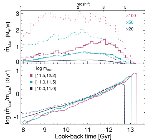
Figure 4. The median SFH of simulated galaxies at z = 1 in the run with (solid) and without (dotted) AGN feedback. Top: the median SFRs of galaxies in three different mass bins. For clarity, the SFRs are scaled down by 100 for galaxies with 10^{11.5} \leq m_{\text{star}} < 10^{12.2} (red), 50 for galaxies with 10^{11.0} \leq m_{\text{star}} < 10^{11.5} (cyan) and 20 for galaxies with 10^{10} \leq m_{\text{star}} < 10^{11} (blue). Bottom: the SSFRs as a function of look-back time.
