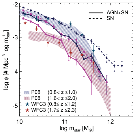
Figure 3. The stellar mass functions of galaxies at z = 2 (reddish colours) and z = 1 (bluish colours). Our estimations at each redshift intervals for simulated galaxies with and without AGN feedback are plotted as solid and dashed lines, respectively. Error bars indicate Poisson errors in the counts. For comparison, we display the mass functions at 0.8 < z \leq 1.0 (blue shading) and 1.6 < z \leq 2.0 (red shading) from Pérez-González et al. (2008). Also included as stars are the simple number counts from the WFC3 sample.
