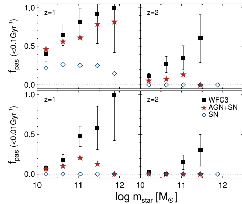
Figure 2. The fraction of passive galaxies for the observations (black squares), the model with SN and AGN (red stars) and the model with SN (blue diamonds). Top panels show the fraction of galaxies showing \text{SSFR} < 0.1 \text{ Gyr}^{-1} , while bottom panels display the fraction of galaxies which are an order of magnitude less active \text{SSFR} < 0.01 \text{ Gyr}^{-1} . Poisson errors are indicated by error bars.
