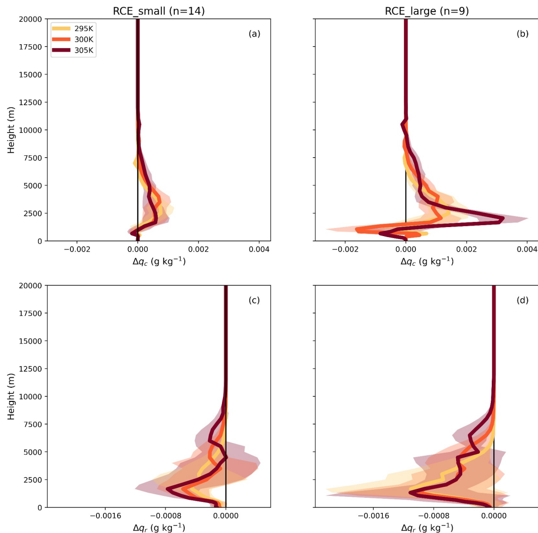
Figure 2. Domain and time mean N_a -driven multi-model mean response of the vertical profile of: (a, b) cloud liquid water content ( q_c ), and (c, d) rain water content ( q_r ), for the different model configurations and sea surface temperatures (the different colors). Shaded areas represent the interquartile range of the different models. This figure is based on the difference between the most polluted ( 2000 \text{ cm}^{-3} ) and cleanest ( 20 \text{ cm}^{-3} ) simulations in each model, divided by two to represent the response to an order-of-magnitude change in aerosol concentration. The responses based on the two other available aerosol contrasts ( 200\text{--}20 and 2,000\text{--}200 \text{ cm}^{-3} ) are presented in Figures S1 and S2 in Supporting Information S1, while the baseline vertical profiles of q_c and q_r are shown in Figure S3 in Supporting Information S1.
