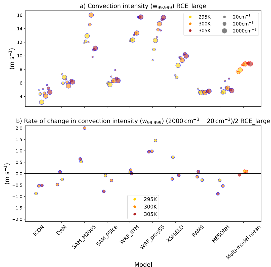
Figure 6. Convection intensity, defined as the 99.999th percentile of the vertical velocity ( w_{99,999} ) at the 500 hPa level (a), and the rate of change in w_{99,999} with aerosol concentration (b) in RCE_large simulations in all models. Markers circled in red on the right side of each panel indicate the multi-model mean. This figure is based on the difference between the most polluted ( 2000 \text{ cm}^{-3} ) and cleanest ( 20 \text{ cm}^{-3} ) simulations in each model, divided by two to represent the response to an order-of-magnitude change in aerosol concentration. The responses based on the two other available aerosol contrasts ( 200 – 20 and 2,000 – 200 \text{ cm}^{-3} ) are presented in Figure S17 in Supporting Information S1.
