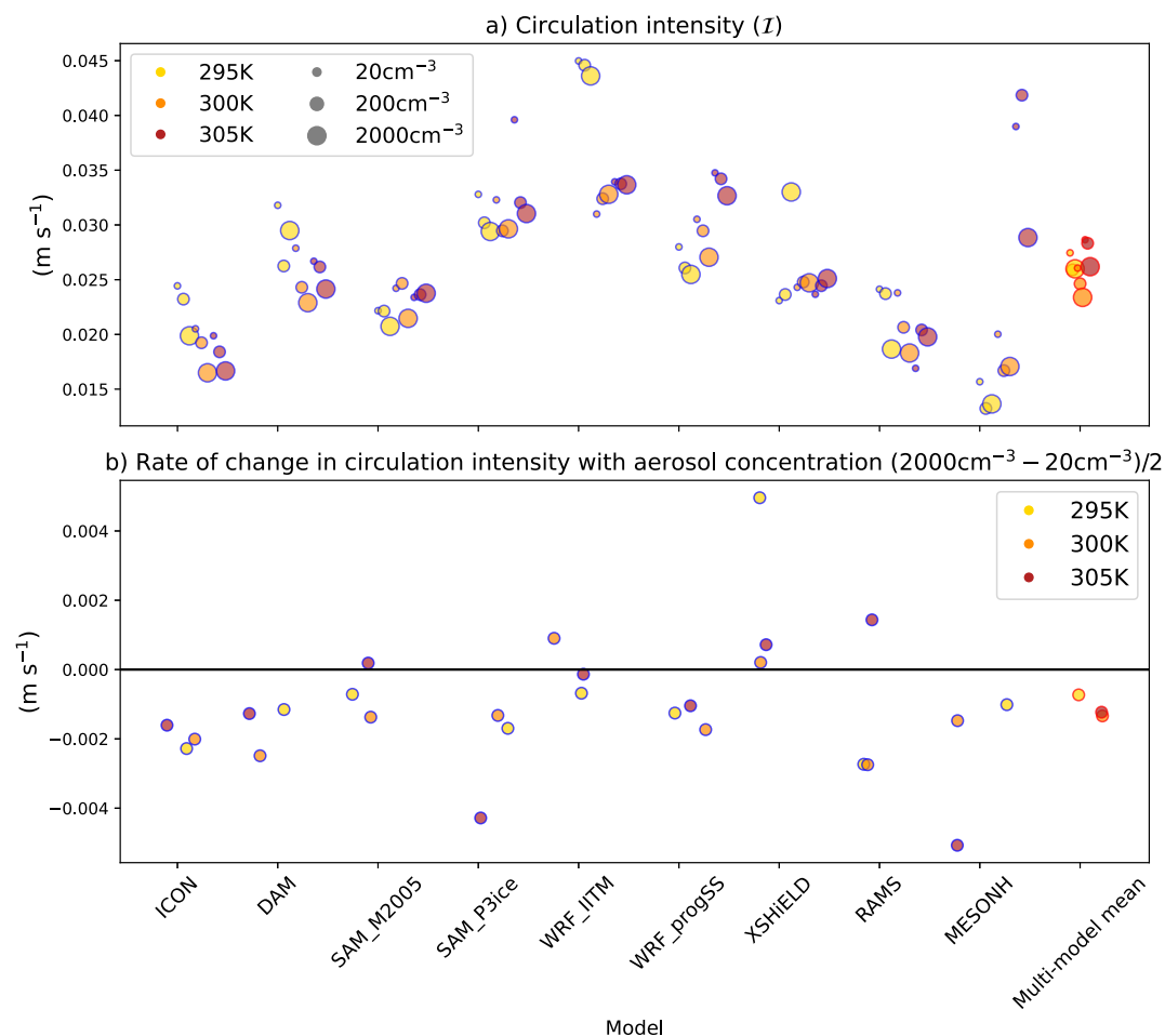
Figure 8. Circulations intensity (a; I ), and the rate of change in I with aerosol concentration (b) for RCE_large simulations in all models. Markers circled in red on the right side of each panel indicate the multi-model mean. This figure is based on the difference between the most polluted ( 2000\text{ cm}^{-3} ) and cleanest ( 20\text{ cm}^{-3} ) simulations in each model, divided by two to represent the response to an order-of-magnitude change in aerosol concentration. The responses based on the two other available aerosol contrasts ( 200\text{--}20 and 2,000\text{--}200\text{ cm}^{-3} ) are presented in Figure S18 in Supporting Information S1.
