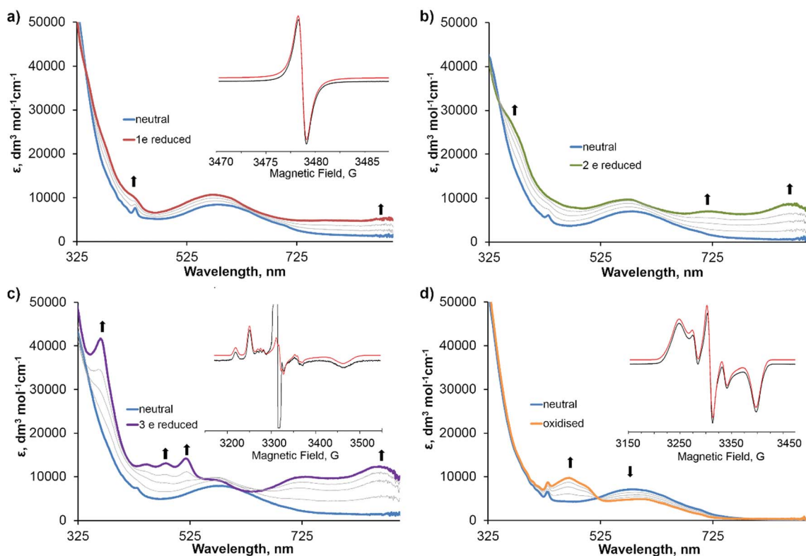
Fig. 2 UV/vis spectra of 3 (blue line in all cases) and the different electrochemically generated radical ion species for the formation of (a) \text{3}^{1-} (red line), (b) \text{3}^{2-} (green line), (c) \text{3}^{3-} (purple line) and (d) \text{3}^{1+} (orange line) with transitional spectra included for all processes (grey lines). All spectra were recorded in DMF solution containing 0.2 M [\text{tBu}_4\text{N}][\text{BF}_4] as supporting electrolyte. The X-band EPR spectra (black line, inset) and corresponding simulated EPR spectra (red line, inset) of each electrochemically generated species were recorded as (a) a fluid solution spectra for \text{3}^{1-} at 298 K, (c) a frozen solution spectra of \text{3}^{3-} at 77 K, and (d) a frozen solution spectra for \text{3}^{1+} at 77 K.
