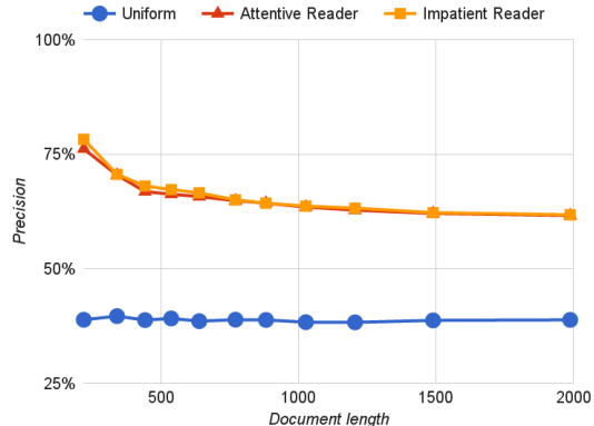
Figure 5: Aggregated precision for documents up to a certain lengths. The points mark the i^{th} decile in document lengths across the corpus.
