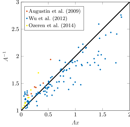
FIGURE 12. Experimentally determined dimensionless decay for waves propagating through a rigid canopy. The black solid line indicates the theoretical prediction A = (1 + \Lambda x)^{-1} (C 1) using the drag coefficient C_D \equiv 1.2 and dots indicate the measurements for individual experiments.
