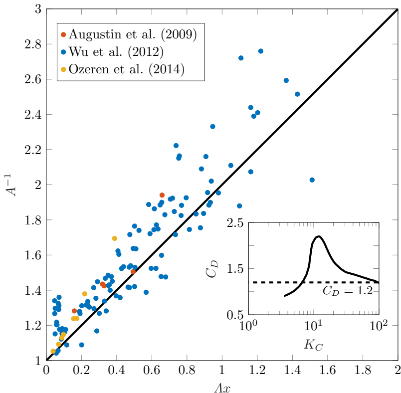
FIGURE 8. Experimentally determined dimensionless decay for waves propagating through a rigid canopy. The black solid line indicates the theoretical prediction A = (1 + \Delta x)^{-1} (4.5) and dots indicate the measurements for individual experiments. We compared 28 of the 29 sets of experiments available – further details are given in Appendix C. The inset plots the experimentally determined relation between the drag coefficient C_D and the Keulegan-Carpenter number K_C for a single cylinder under uniform oscillatory flows (Keulegan & Carpenter 1958). Since wave velocities are depth-dependent, following the definition by Chen et al. (2018), the velocity scale in K_C is chosen to be the maximum velocity at the half water depth.
