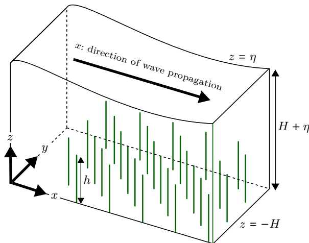
FIGURE 2. Schematic diagram of waves with fluid velocity \hat{\mathbf{u}} propagating through a rigid canopy over a varying substrate with \hat{z} = -\hat{H} . The free-surface elevation is parametrised with \hat{z} = \hat{\eta} and the submerged green obstacles represent individual plants with height \hat{h} .
