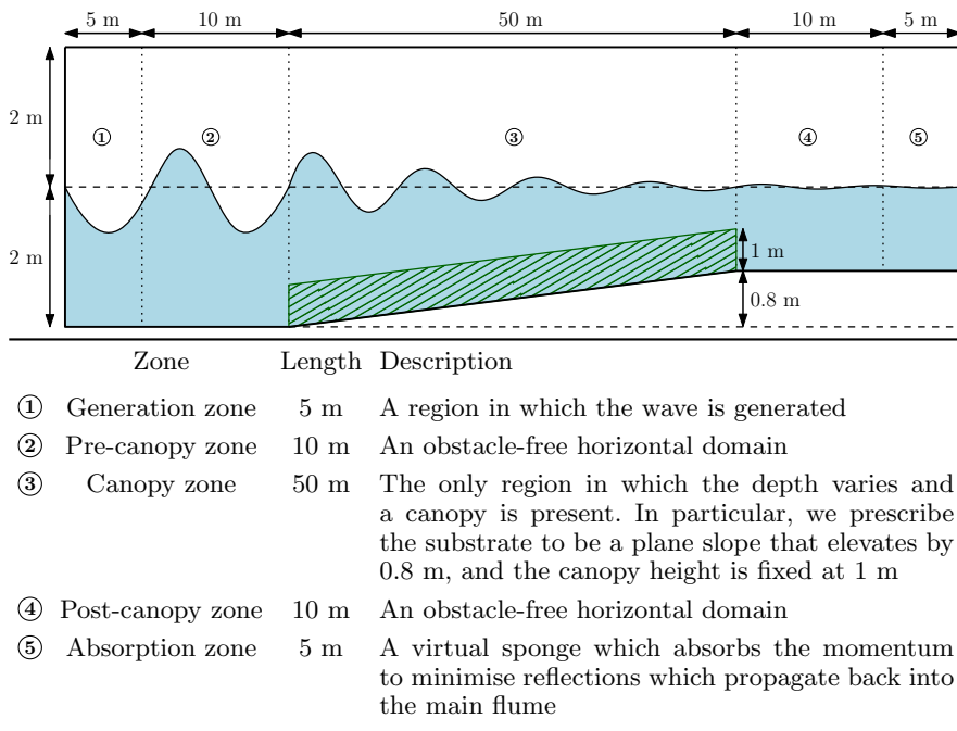
FIGURE 6. Schematic diagram on the dimensions of the numerical wave flume, with the canopy denoted in green. The flume consists of five zones: generation zone, pre-canopy zone, canopy zone, post-canopy zone, and absorption zone. The table below describes each individual zone.
