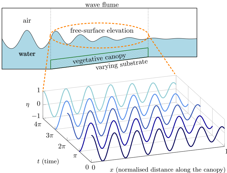
FIGURE 1. Schematic diagram of a wave flume with waves propagating from left to right. Sample solutions of the free-surface elevation, \eta , is plotted as a function of distance of propagation at various times—this is to highlight the slow modulation of the wave due both the vegetative canopy and the varying substrate.
