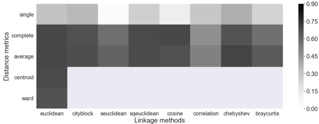
Figure 6. Heatmap of CCC values across combinations of distance and linkage methods used in hierarchical clustering.
