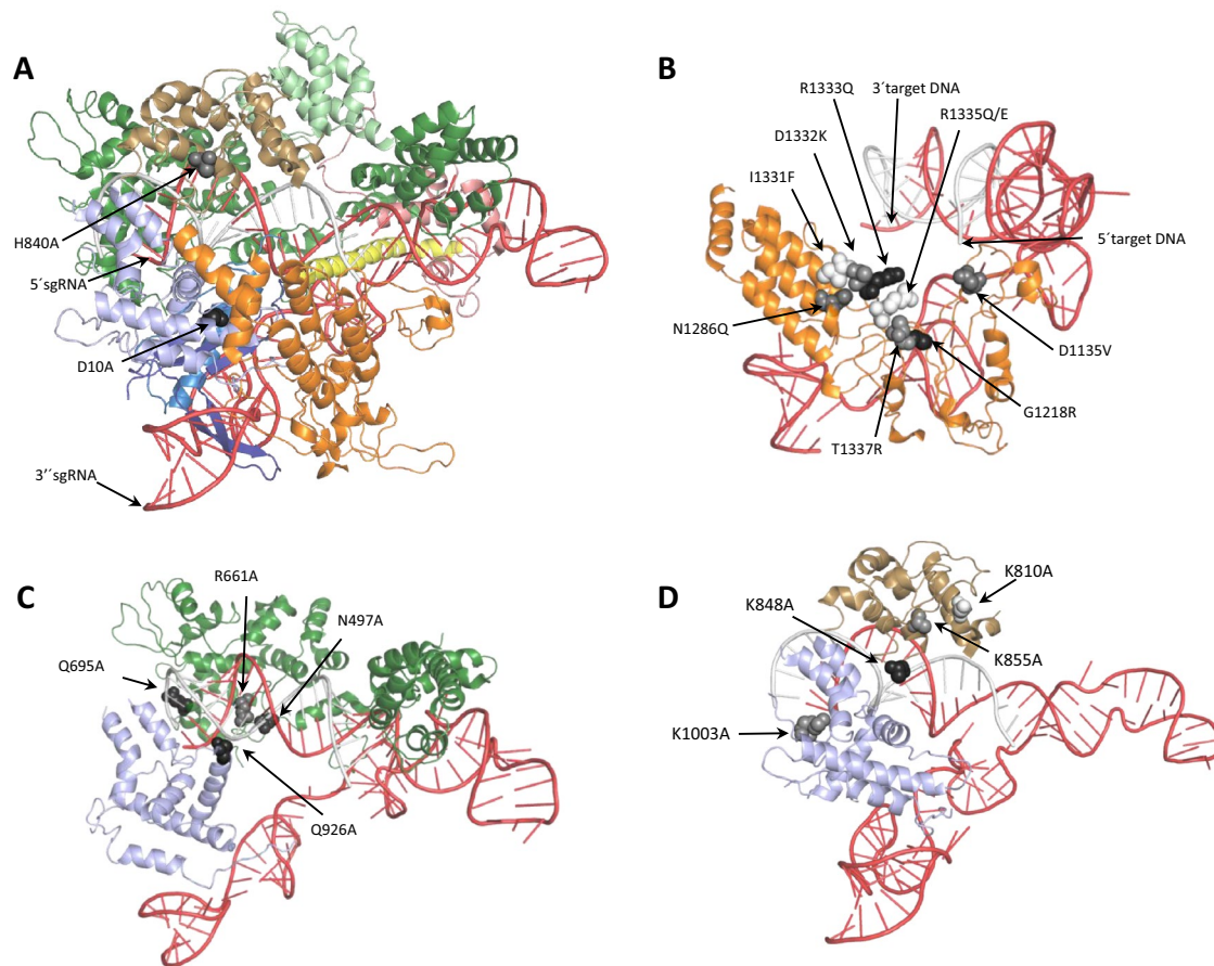
Fig. 1 Position of mutagenized residues in SpCas9. a Crystal structure of SpCas9 in complex with sgRNA and target DNA (PDB ID 4OO8). The position of the catalytic residues responsible for the HNH (Asp-10) and the RuvC (His-840) nuclease activity, which are mutated in the D10A and H840A nickases, are shown in black and grey respectively. b Detail of the PAM interaction domain in complex with guide RNA and target DNA showing the position of the key residues mutated in variant Cas9 with altered PAM specificities and how
