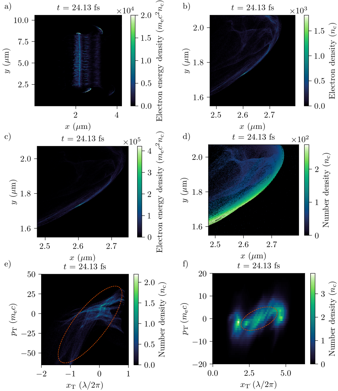
Figure 2.8: 2D PIC simulation results qualitatively describing typical transversally-limited ZVP electron bunch structure. Here, a_0 = 100 , \bar{n}_e = 100 and other simulation parameters are given in Table B.1. a) Electron energy density for the full simulation window, corresponds to Figure 2.4f). The box highlights the bunch presented in the following plots. b) Electron number density of the electron bunch. c) Electron energy density of the electron bunch, the colour bar scale has been increased compared to Figure a) to observe the internal structure. d) The mean electron energy across the electron bunch, suggesting a position-dependent energy or quasi-monoenergetic nature to the electron bunch [130]. Cells with no macroparticles are black. e) The transverse phase space in the 2D simulation plane. The ellipse describes the calculated emittance. The skew of the ellipse is a consequence of a low-density tail on the phase space beyond the bottom left corner. f) This plot was extracted from the equivalent 3D simulation and describes the transverse emittance in the z -direction. Again the ellipse marks the emittance. The relatively well-defined border to the phase space and the mild tilt (indicating only mild divergence) are direct consequences of the 2D nature of the interaction.
