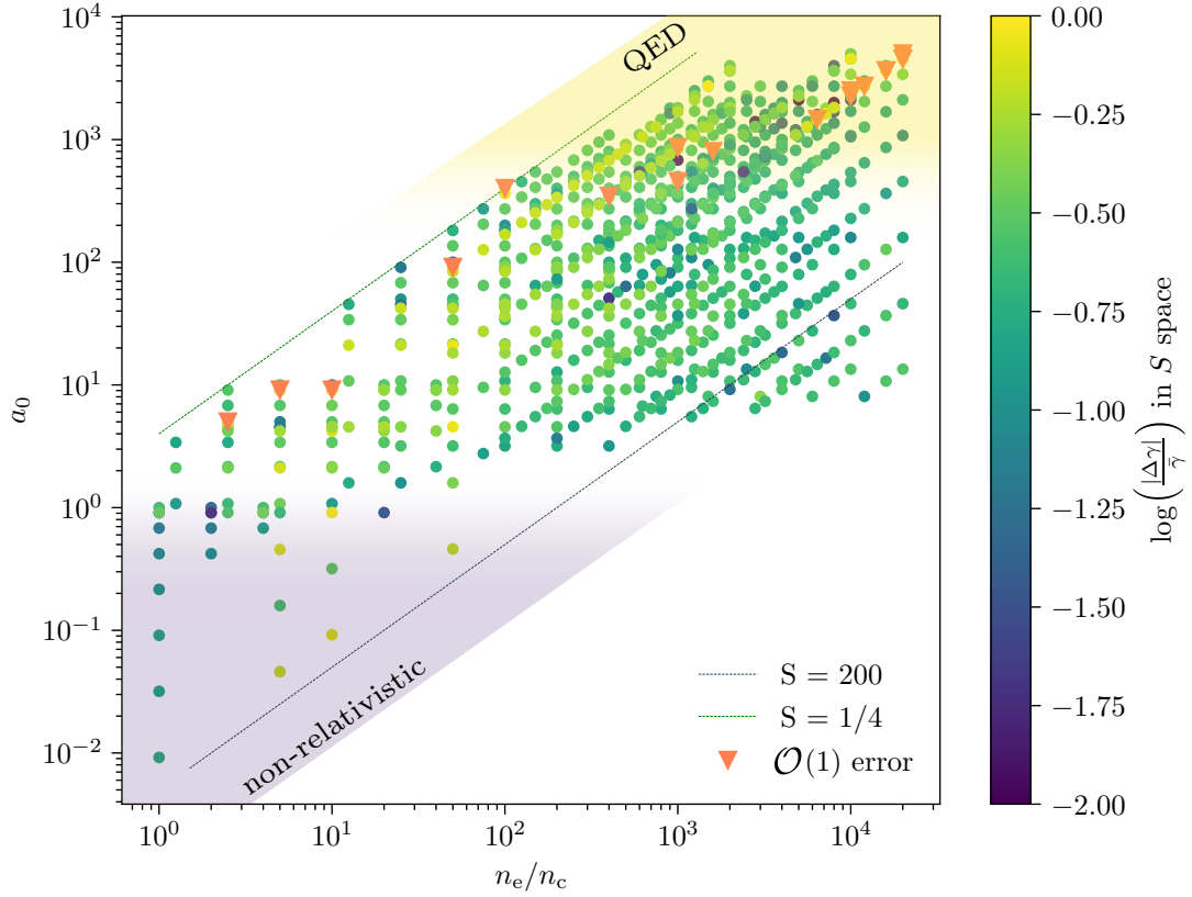
Figure 2.12: The relative errors for each mean energy data point compared to Figure 2.10. Additional simulation parameters are given in Table B.1. The orange triangles indicate data points for which the model fails to predict the mean energy.
