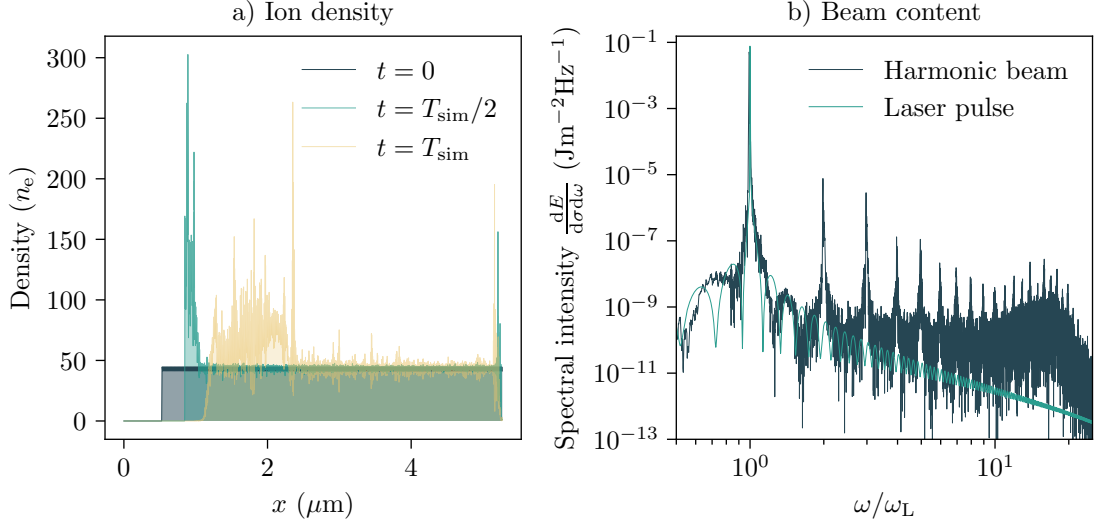
Figure 3.2: 1D PIC simulation of the SP1 ORION beamline geometry at a_0 = 7 interacting with a pre-ionised CVD target. Additional simulation parameters are given in Table 3.1, real laser parameters are listed in Table 1.3. a) Ion density at initialisation ( t = 0 ), halfway ( t = T_{\text{sim}}/2 ) and at the simulation end ( t = T_{\text{sim}} ) demonstrating hole-boring. b) Absolute spectral intensity of the laser pulse and reflected harmonic beam obtained via Fourier transform. The harmonic beam retains the laser pulse spectral width. Even harmonics are significantly suppressed at this polarisation. The large bump in the distribution around the 18 th harmonic is spuriously generated via numerical heating.
