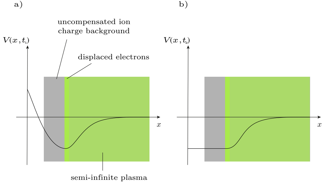
Figure 2.2: Diagram of the ZVP potential well, V(x, t) . a) At t_1 , electrons in the skin layer are confined within a potential well maintained by the uncompensated ion population and ponderomotive pressure of the laser pulse. b) At t_2 when the vector potential passes through zero then the outer wall of the potential well disappears and electrons can escape the plasma, breaking adiabaticity.
