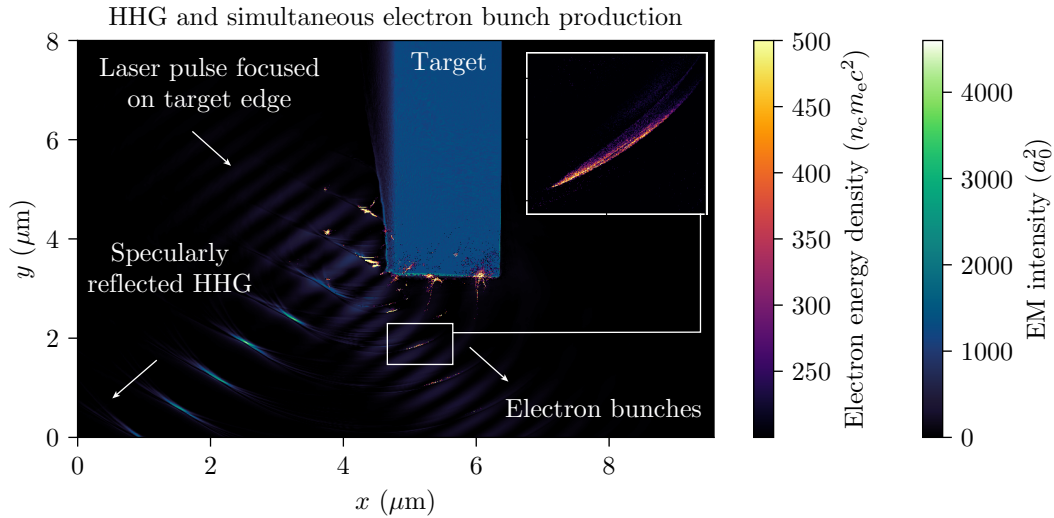
Figure 4.5: A simulation of the planned GEMINI-PW experimental setup for the measurement of ZVP electron bunches. Here, a_0 = 21.6 , \bar{n}_e = 181 . Additional simulation parameters and corresponding laser parameters are listed in Tables B.3 and 1.3 respectively. This novel setup enables the simultaneous measurement of attosecond ZVP electron bunches and their coherent emission of X-ray light. The GEMINI-PW laser pulse is incident at 45^\circ on the low-density polyethylene target with a preplasma scale length of 0.2\lambda_L . For this angle of incidence, transmitted bunches and specularly reflected X-ray harmonics are produced at a frequency of \omega_L .
