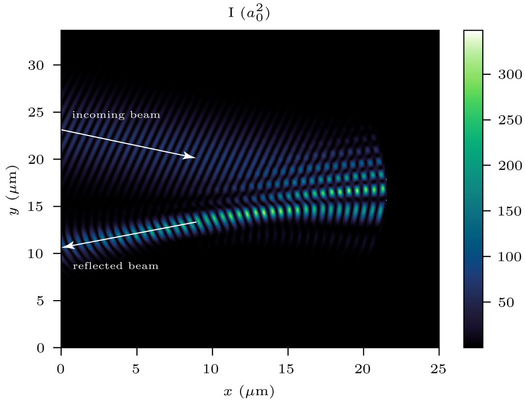
Figure 3.1: Electromagnetic field intensity in a 2D PIC simulation of a relativistic ( a_0 = 30 ) laser pulse incident on a solid density plasma, \bar{n}_e = 100 . These parameters are chosen to clearly highlight the effect of hole boring, typical targets fielded on the ORION experiment were of higher density. The incoming beam is specularly reflected off the target which is curved by the radiation pressure leading to beaming in the reflected harmonic beam.
