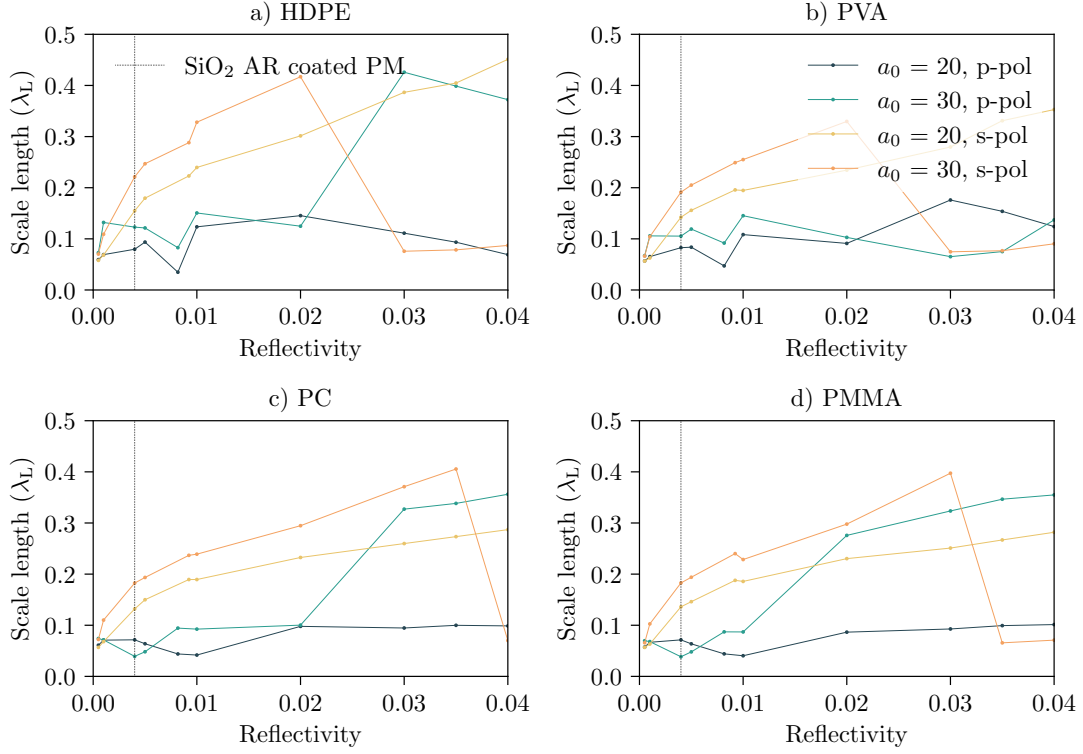
Figure 3.10: Preplasma scale length parameter scan for a variety of plastic targets. The main laser pulse intensity profile is taken from Equation 1.9.1 while the PM reflectivity and peak normalised vector potential are varied. Additional simulation parameters are referred to in the text and laser parameters in Table 1.3. Target materials are a) HDPE, b) PVA, c) PC and d) PMMA. The dashed line highlights the reflectivity of the SiO 2 AR-coated PM for the SP2 wavelength. The preplasma scale length remains small for the range of parameters explored.
