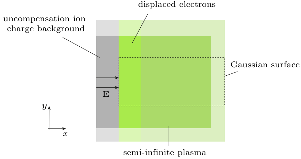
Figure 1.2: A diagram to illustrate the derivation of plasma frequency. The electrons of a semi-infinite plasma are displaced inwards by some external force leaving in their wake an uncompensated space charge of ‘immobile’ positive ions. By constructing a Gaussian surface along the dashed line, the electric field associated with the positive space charge can be calculated from Gauss’ Law.
