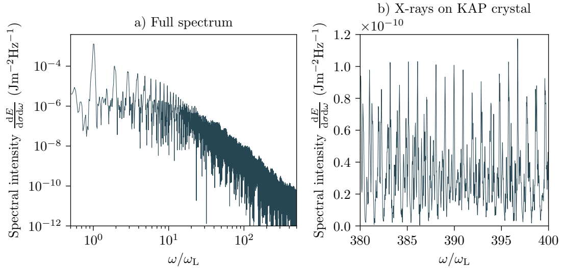
Figure 4.3: 1D PIC simulation of XHHG on the GEMINI PW laser system. Here, a_0 = 24 , \bar{n}_e = 379 in the laboratory frame. Additional simulation parameters and corresponding laser parameters are listed in Tables B.2 and 1.3 respectively. The beamline is incident on a \text{SiO}_2 target under optimised conditions. a) The full harmonic spectrum. b) Window of the spectrum recorded by the KAP OHREX crystal. The harmonics are clearly visible.
