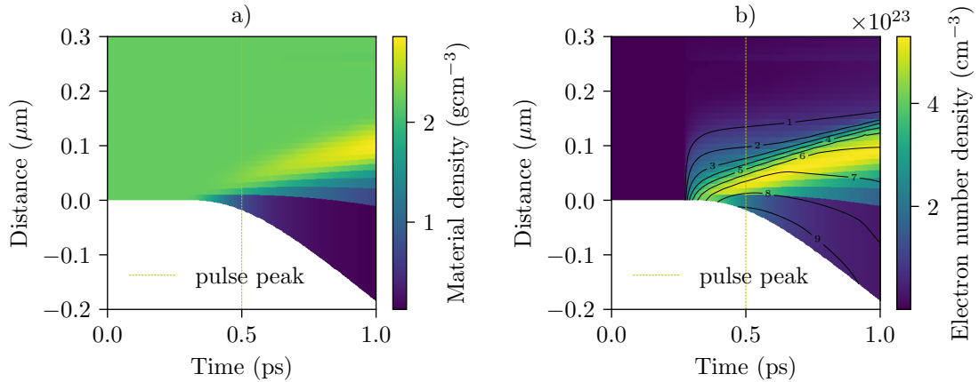
Figure 3.7: Silicon dioxide plasma mirror switch on from irradiation by the SP2 main pulse at 45^\circ angle of incidence and p-polarisation. The main laser pulse intensity profile is taken from Equation 1.9.1 with a peak normalised vector potential of a_0 = 30 . Additional simulation parameters are referred to in the text and laser parameters in Table 3.1. The laser pulse travels in the +\hat{x} -direction. The main pulse peak intensity is marked at 500 ps in the simulation. a) Material density as a function of time, a short preplasma is formed alongside hole-boring. b) Electron number density as a function of time. The contours map the ionisation level.
