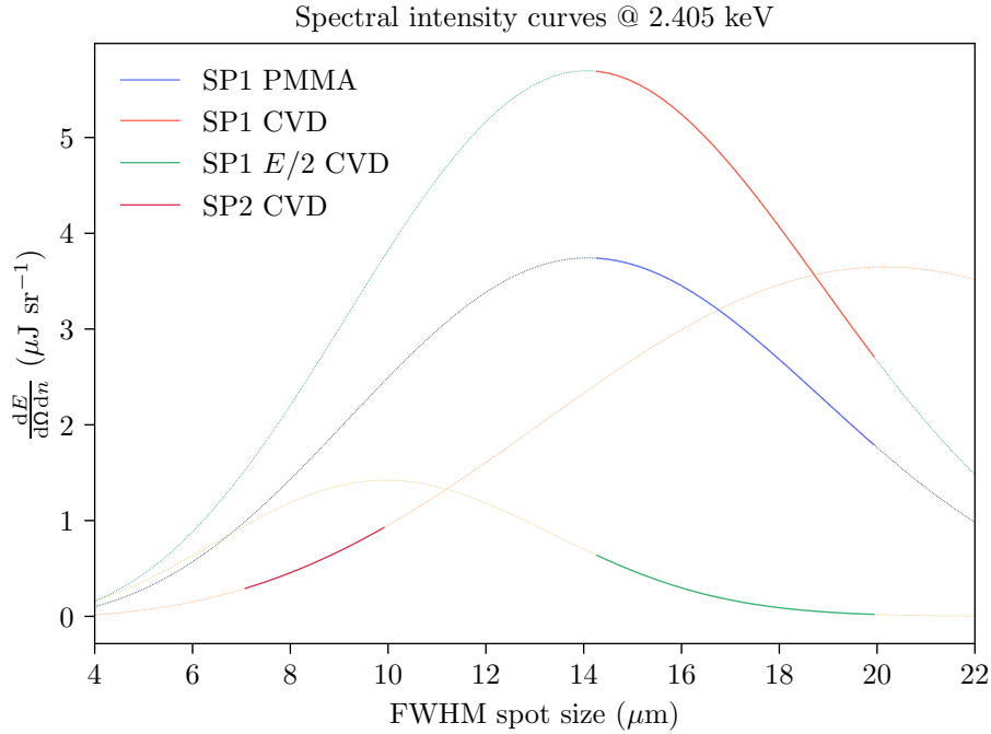
Figure 3.18: Dependence of the harmonic beam spectral intensity on laser spot size at 2.405 keV. Targets and beamlines relevant to the experiment are plotted. Combining the theoretical results of Section 3.2 with the known parameters of the ORION laser system, listed in Table 1.3, the spectral intensity of the harmonic beam can be calculated as a function of laser spot size (the most poorly constrained parameter of the system). The consistent shape of the curves is a result of the balance between hole boring, that reduces divergence with increasing spot size, and the roll off, that reduces the X-ray harmonic conversion efficiency with the reduced intensity from increasing spot size. The half-energy single beamlet SP1 laser is demarcated by E/2 . The thick lines indicate likely values for the laser spot sizes in this experiment. The SP1 harmonic beams are strongly affected by the exponential roll-off, unlike the SP2 beamline.
