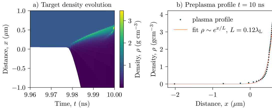
Figure 3.9: Typical preplasma formation from the p-polarised 16^\circ angle of incidence of the ORION SP2 laser prepulse on an HDPE target. In this simulation the laser is modelled from 10 ns before the main pulse with a_0 = 30 and attenuated by a PM of reflectivity 0.004. The laser pulse intensity profile is taken from Equation 1.9.1. Additional simulation parameters are referred to in the text and laser parameters in Table 1.3a) Typical preplasma expansion elucidated via target density. By the time of the main pulse, hole-boring is dominant over plasma expansion. b) An exponential fit ( \rho \sim e^{x/L} ) for the preplasma scale length, L , at the time of arrival of the main pulse. For this simulation the optimum fit is L = 0.12\lambda_L .
