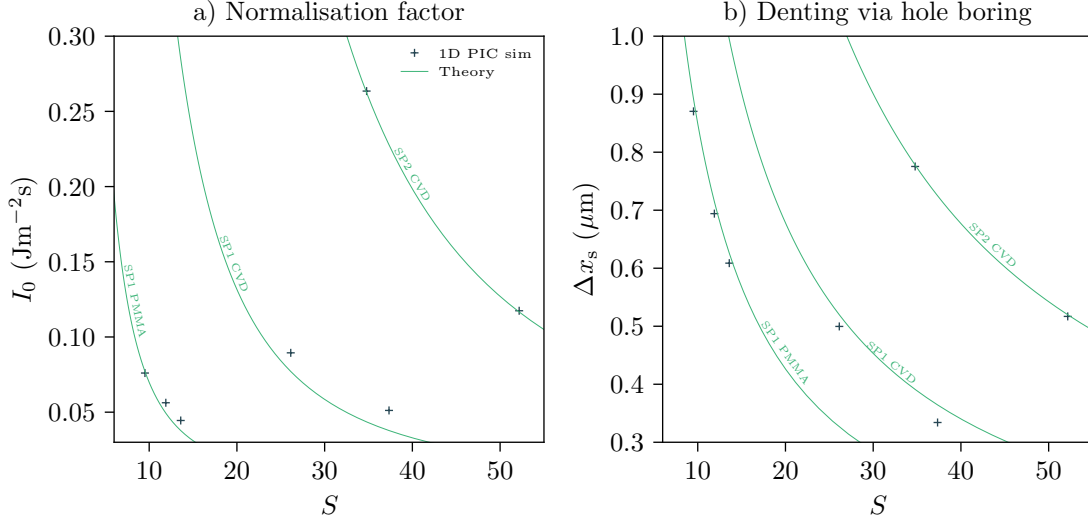
Figure 3.3: Comparison between simulation and analytical predictions of hole-boring and SHHG normalisation factor in the ORION laser facility parameter space for CVD and PMMA targets. Additional simulation parameters are given in Table 3.1, real laser parameters are listed in Table 1.3. a) The normalisation factor, I_0 , where the spectral intensity, I = I_0 n^{-p} for low order harmonics. b) The depth of hole-boring compared to the initialised plasma surface. Note that the steep density gradient as visible in Figure 3.2a ensures the surface position is well-defined. Both parameters are expressed in the laboratory frame.
