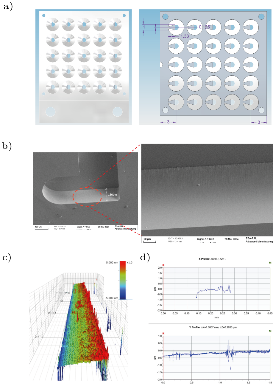
Figure 4.6: Targets designed for observation of ZVP electron bunches. a) Target array design with conical array holder and tapered finger, lengths in mm. b) Scan of the etched wafer, striations develop towards target rear due to etching technique. c) A 3D plot of surface variation. Scalping and striations are visible but too small to interfere with laser pulse transmission at 45^\circ . d) Lineouts of c), the y -profile is along the target edge of interest.
