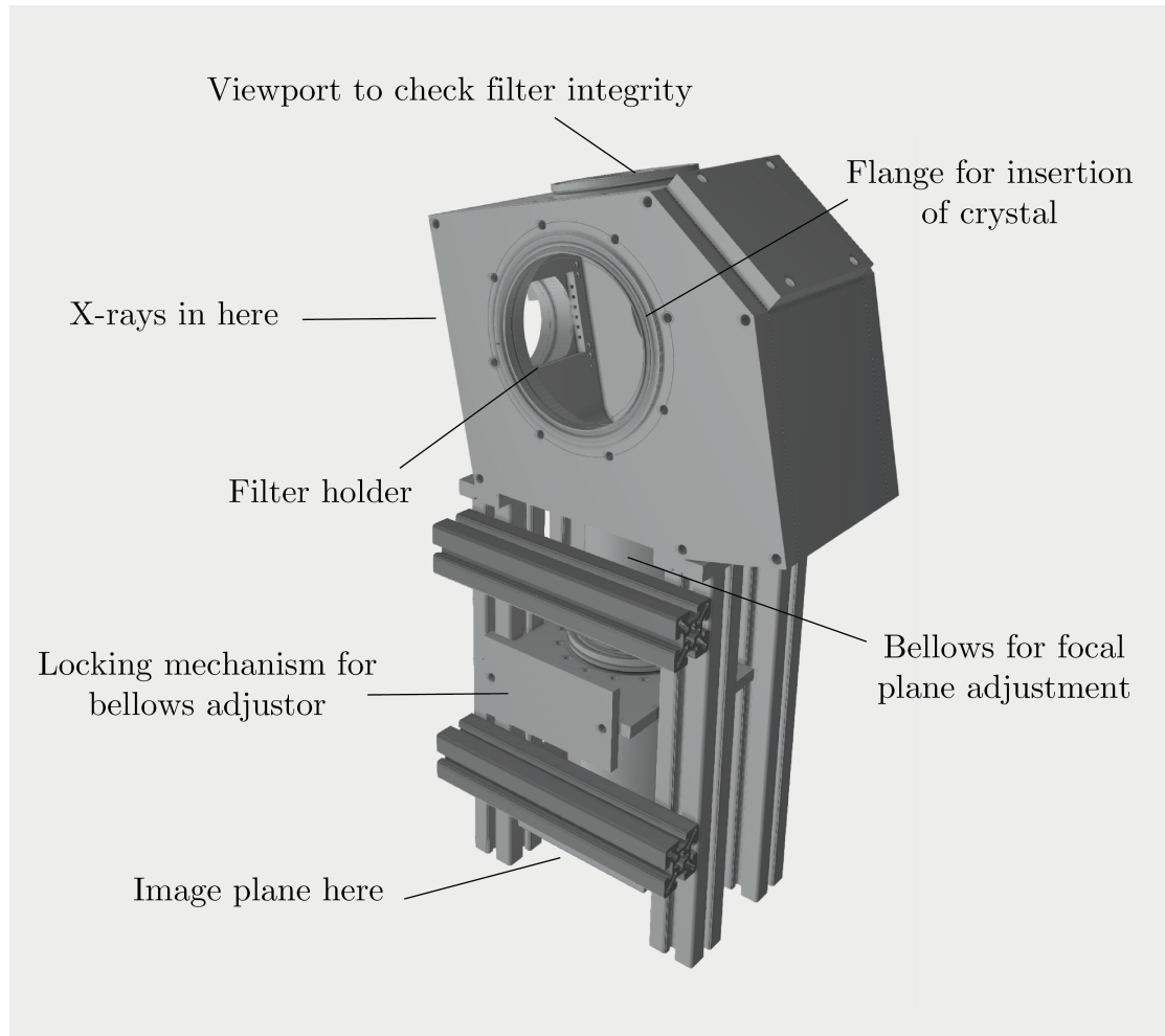
Figure 4.2: Replica OHREX (the OxHREX) spectrometer designed and built for the measurement of X-ray harmonics at GEMINI. Designed for compatibility with existing OHREX flange mounted crystals.
