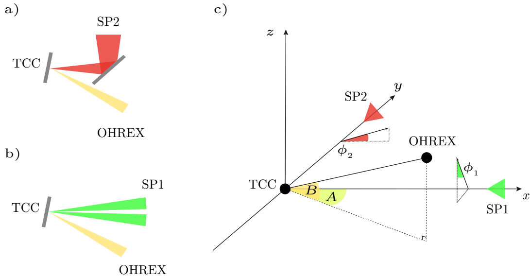
Figure 3.12: ORION target chamber geometry and schematics of the experiment beamlines. a) The SP2 beamline (infra-red) is reflected from a plasma mirror at 45^\circ before the main target incidence to increase the laser contrast. The specularly reflected harmonic beam (yellow) was then directed towards the OHREX spectrometer by varying the target angle as required. b) The SP1 beamline is composed of two beamlets with their centres separated by 10.3^\circ . The non-linear interaction produces a single harmonic beam (yellow) as with non-collinear gating [153]. Since the two pulses are fully coherent with respect to one another, the propagation direction of the harmonic beam remains constant and in the direction of the sum of the the two individual beamlets' reflections in the linear case. When using only one beamlet, the target angle was adjusted accordingly to direct the harmonic beam to the OHREX. c) ORION target chamber geometry with the location of the target, OHREX spectrometer and the SP1 (green) and SP2 (infra-red) beamlines and their corresponding polarisations, \phi_1 = 11.8^\circ and \phi_2 = 16.4^\circ .
