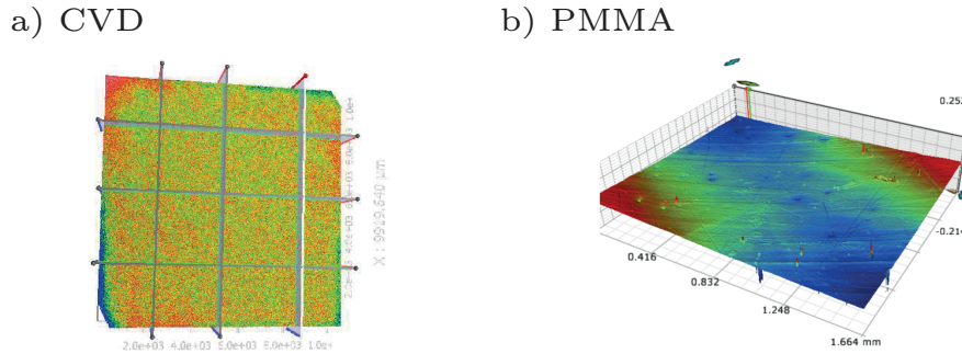
Figure 3.14: ORION experiment 3D scans of target roughness. a) CVD with roughness \Delta s = 4 nm and S \approx 26, 35 for SP1 and SP2 beamlines respectively. b) PMMA with roughness \Delta s = 11.2 nm and S \approx 10, 13 for SP1 and SP2 beamlines respectively.
