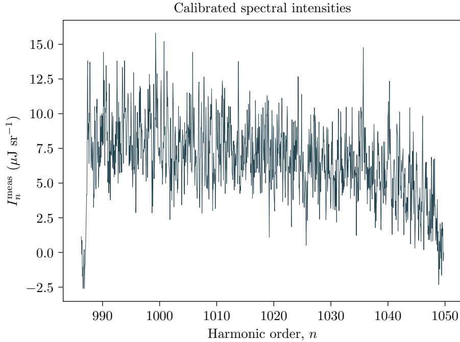
Figure 3.17: Typical (SP1, PMMA) ORION experiment calibrated IP response for the quartz ( 10\bar{1}1 ) crystal. SP1 laser parameters are listed in Table 1.3.
