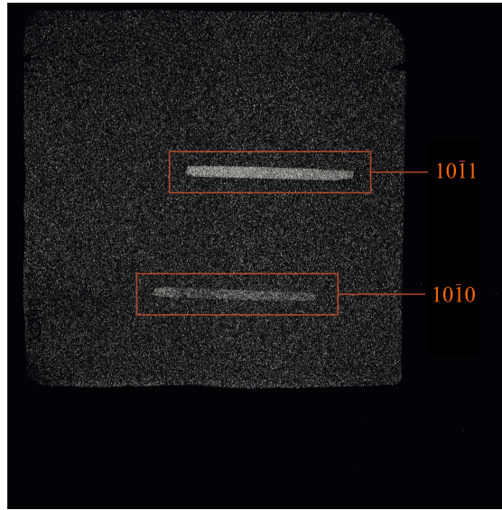
Figure 3.15: Unprocessed shot data from a FLA7000 scanned image plate converted to PSLs. The image plate and two crystal images are clearly visible.
