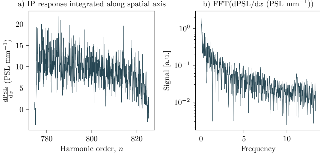
Figure 3.16: Typical (SP1, PMMA) uncalibrated shot data for the quartz (10 \bar{1} 0) image SP1 laser parameters are listed in Table 1.3. a) IP spatial axis integrated signal with dispersion axis. b) Fourier transform of a) with no evidence of harmonics.
