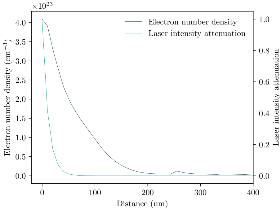
Figure 3.8: The attenuation of the SP2 laser pulse is calculated as it propagates through a switched-on PM. The main laser pulse intensity profile is taken from Equation 1.9.1 with a peak normalised vector potential of a_0 = 30 . Additional simulation parameters are referred to in the text and real laser parameters in Table 1.3.
