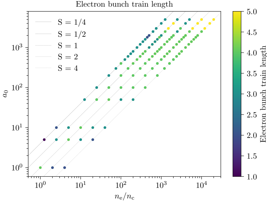
Figure 2.11: Mass-limited electron bunch train length as a function of laser intensity and plasma density. Additional simulation parameters are given in Table B.1. Lines of constant peak S parameter are plotted for reference. Clearly, decreasing S reduces the bunch length.
