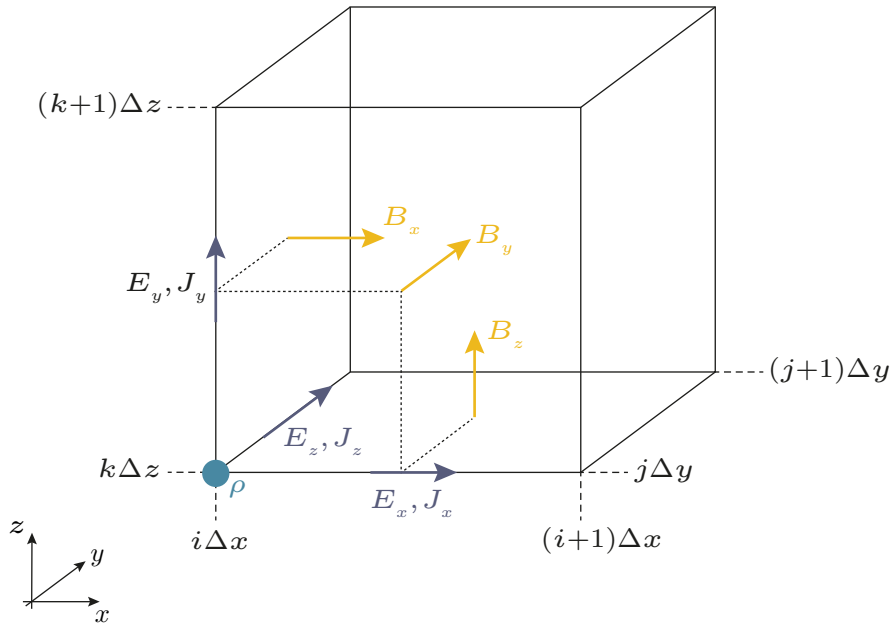
Figure 1.4: A representation of the staggered 3D Yee grid. For the cell at (i\Delta x, j\Delta y, k\Delta z) for spatial centring of the curl operations, including the locations where all system properties are defined.
