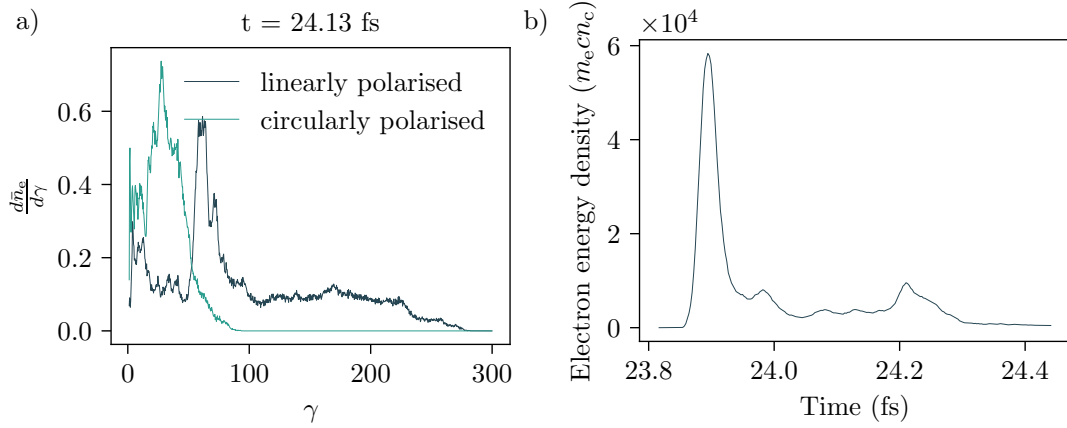
Figure 2.9: Energy spectra for transversally-limited electron bunches formed via linearly and circularly polarised laser pulses. Here, a_0 = 100 , \bar{n}_e = 100 and other simulation parameters are given in Table B.1. a) Energy spectra for transversally-limited electron bunches formed via linearly and circularly polarised laser pulses. b) Mean energy density in a cell as the centre of a transversally-limited ZVP electron bunch propagates through it, demonstrating the attosecond duration in time of the electron bunch.
