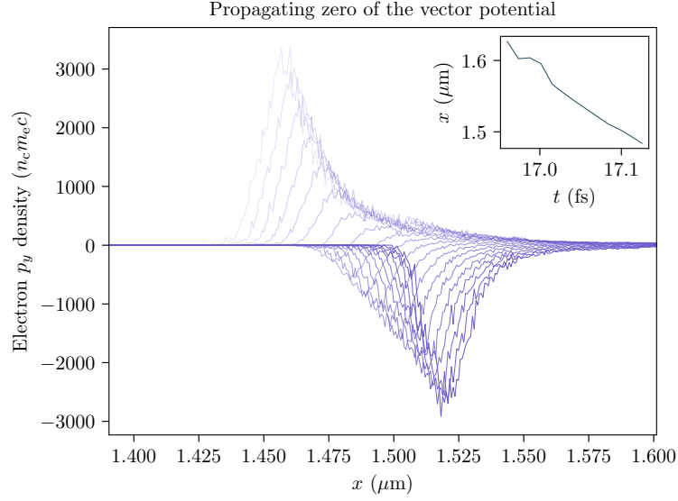
Figure 2.5: Propagation of a vector potential zero through the ablating ZVP electron bunch via the proxy of transverse momentum conservation. Here, a_0 = 100 , \bar{n}_e = 100 and other simulation parameters are given in Table 2.1. Plotted is the mean transverse momentum of the ZVP electron bunch as a function of x . Each line represents a timestep ( \Delta t = 2.51 as) with time increasing with decreasing opacity. As time increases the bunch moves in the -\hat{x} -direction away from the target surface. By conservation of transverse momentum, the zero of the vector potential exists where the transverse momentum is macroscopically zero, i.e. where p_y = 0 within the bunch. With increasing time the bunch and the zero move in the -\hat{x} -direction with the zero overtaking the electron bunch. The inset tracks the position of the zero of the vector potential with time.
