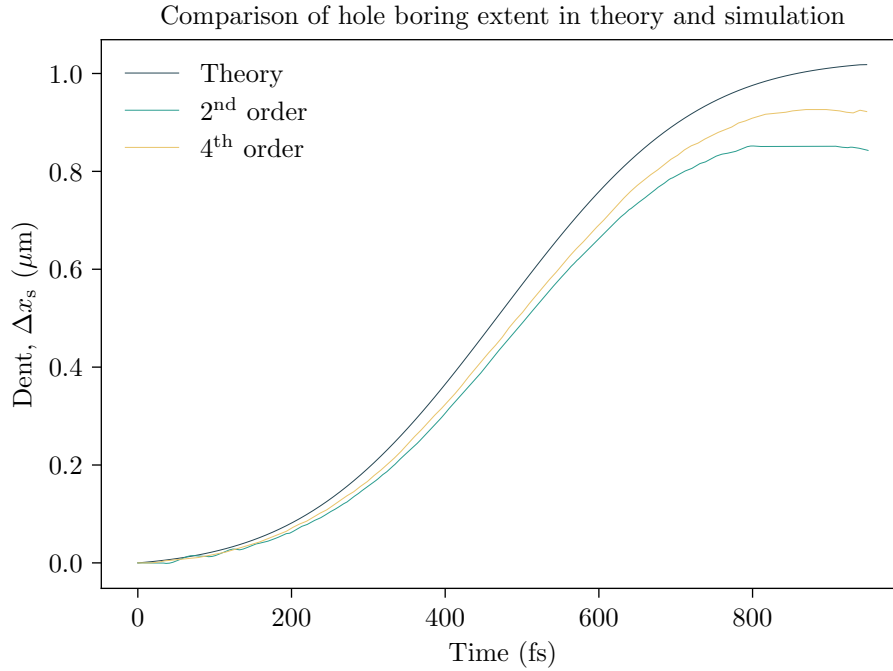
Figure 3.4: The effect of the PIC code particle shape function on numerical heating demonstrated via the extent of hole-boring. Additional simulation parameters are given in Table 3.1, real laser parameters are listed in Table 1.3. The deviation from the theoretical prediction increases with time, and the error decreases for increasing order of the shape function.
