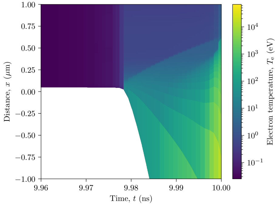
Figure 3.11: The typical electron temperature of a plastic target after irradiation by a petawatt class laser prepulse. This is the same simulation as presented in Figure 3.9. Namely, an a_0 = 30 p-polarised laser pulse attenuated by a plasma mirror of reflectivity 0.004 incident on an HDPE target at 16^\circ . The bulk and preplasma temperatures differ by multiple orders of magnitude.
