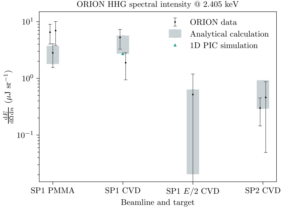
Figure 3.19: X-ray harmonic spectral intensities at 2.405 keV measured on the ORION experiment compared to theory and simulation. The analytical calculation corresponds to the thick lines marked in Figure 3.18. The 1D PIC simulation result is derived from Figure 3.5 and scaled to the ORION laser pulse duration. Beamline parameters are listed in Table 1.3.
