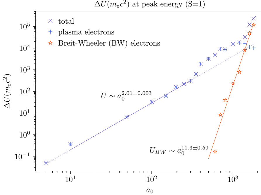
Figure 2.13: Peak instantaneous bulk electron bunch total energies after escaping to the plasma bulk rear. Additional simulation parameters are given in Table B.1. Energies begin to deviate from the anticipated scaling at approximately a_0 = 300 . Above a_0 = 1000 , BW pair-produced electrons begin to dominate and the peak energies rise rapidly.
