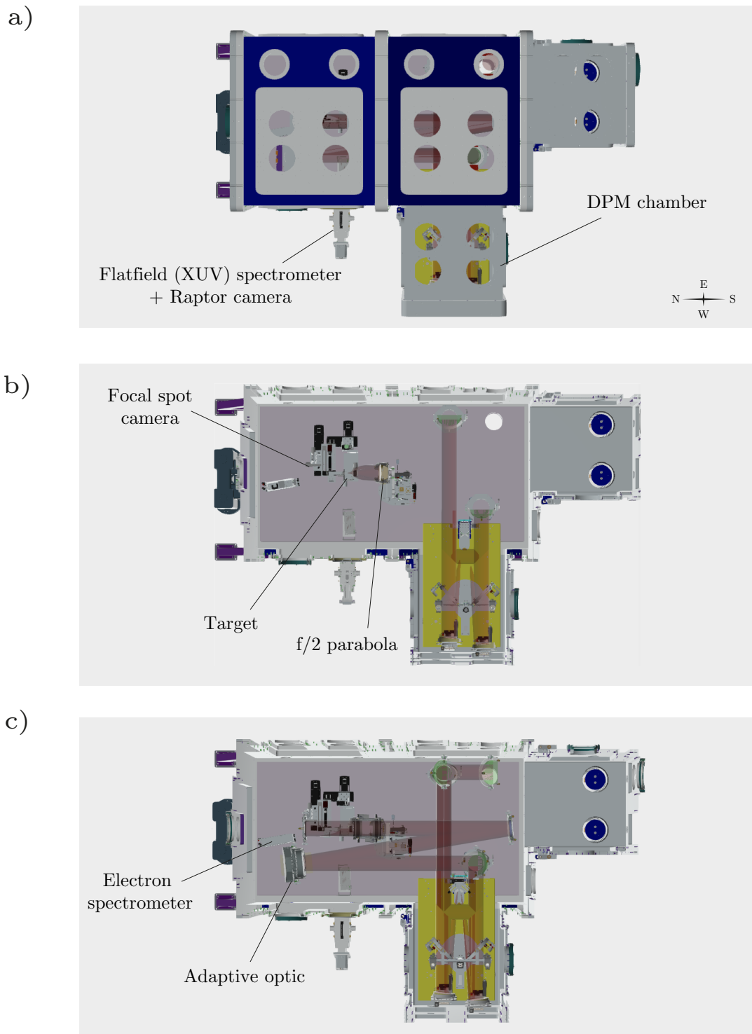
Figure 4.1: A 3D model of the GEMINI PW target chamber layout for this experiment produced by CLF engineers. a) Outer body of the target chamber. b) Lower level of the target chamber including the target at TCC. c) Upper level of the target chamber.
