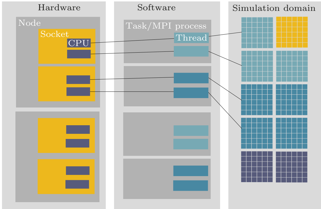
Figure 1.6: Representation of the interaction of the ARCHER2 hardware and software components when running SMILEI. Each CPU is assigned a thread, each task is carried out by one socket. A task tackles one MPI patch collection with threads working through patches.
