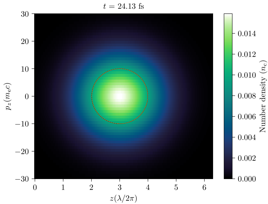
Figure A.1: Emittance calculation for an ideal Gaussian distribution in phase space, f_n(z, p_z) = 1/(2\pi s_z s_{pz}) \exp[-((z - m_z)^2/(2s_z^2) + (p_z - m_{pz})^2/(2s_{pz}^2))] , centred at (m_z, m_{pz}) = (3, 0) with standard deviations (s_z, s_{pz}) = (1, 10) .
