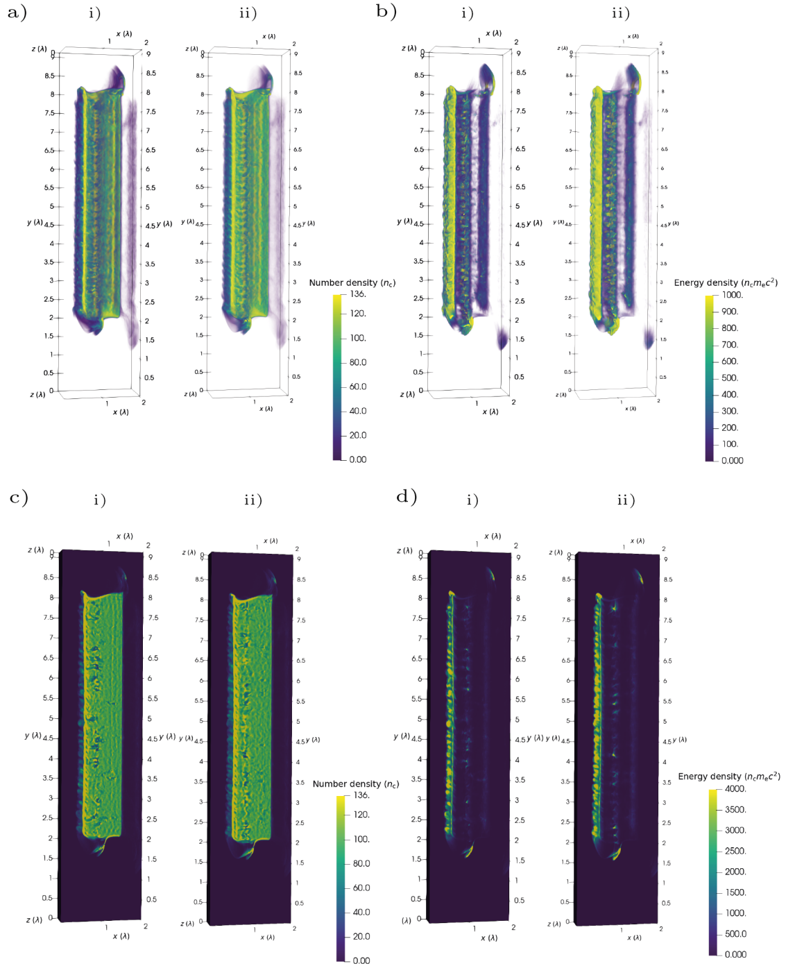
Figure B.1: Comparison between the initial 3D simulation and a lower resolution version. a) Electron number density. b) Kinetic energy density. c) and d) are slices of a) and b) respectively. i) Initial simulation. ii) Lower resolution simulation. Good convergence is demonstrated.
