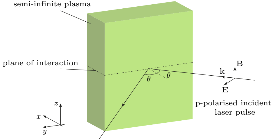
Figure 2.1: Diagram of a p-polarised laser pulse incident at angle \theta specularly reflected from a solid density plasma. From consideration of the Lorentz force equation, it is clear that all forces and therefore all plasma particle dynamics are confined to a plane.
