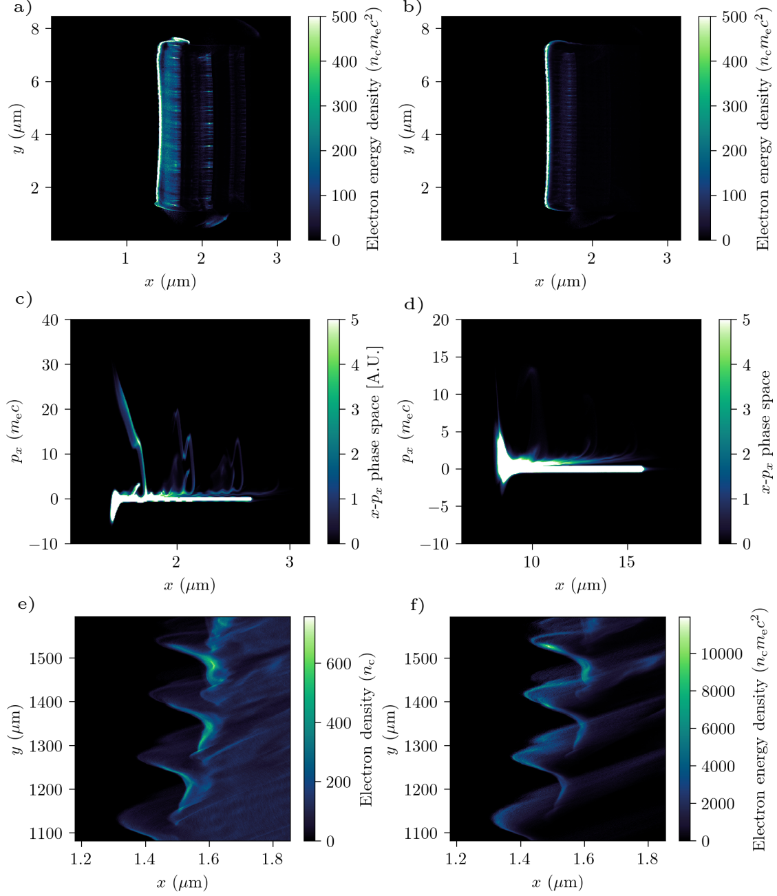
Figure 2.6: Electron dynamics in a 3D PIC simulation. Here, a_0 = 100 , \bar{n}_e = 100 and other simulation parameters are given in Table 2.1. a) and b) Electron energy density for linearly and circularly polarised laser pulses respectively. c) and d) Electron longitudinal momentum for linearly and circularly polarised laser pulses respectively. e) Electron density at the plasma surface streaked in time. f) Electron energy density at the plasma surface streaked in time.
