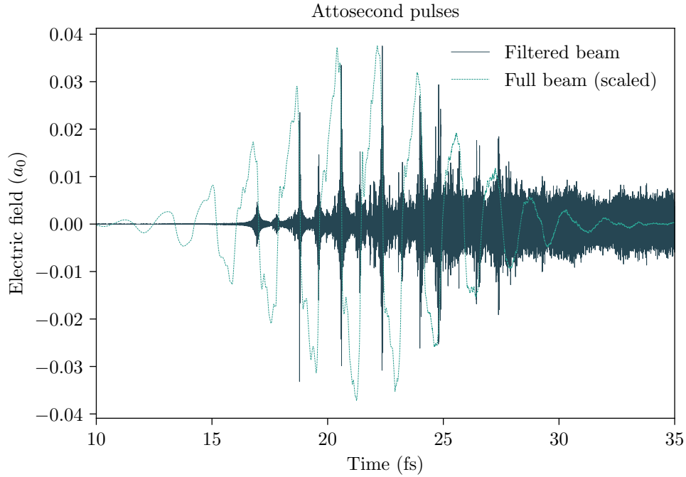
Figure 3.6: Attosecond pulse train from the filtered reflected laser pulse. Here, a_0 = 10 and \bar{n}_e = 294 , differences between this high resolution simulation and the previous simulations are discussed in the text, real laser parameters are listed in Table 1.3. The filtered beam contains only harmonics above n = 50 .
