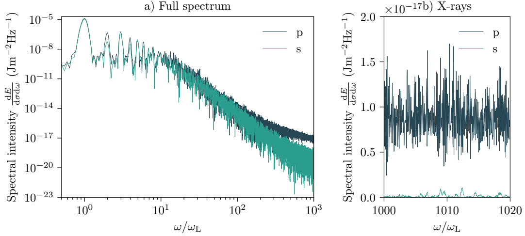
Figure 3.5: Reflected beam harmonic content up to the keV range in a high-resolution 1D PIC simulation of a test pulse with SP1 ORION beam geometry incident on a CVD target. Here, a_0 = 10 and \bar{n}_e = 294 , differences between this high resolution simulation and the previous simulations are discussed in the text, real laser parameters are listed in Table 1.3. The absolute spectral intensity is calculated from the Fourier transform of the reflected beam electric field. The s- and p-polarised components of the beam are analysed separately for both a) the full spectrum and b) the X-ray harmonics accessible with the OHREX quartz (10 \bar{1} 1) crystal.
