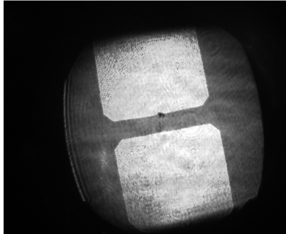
Figure 1.7: Image of the ORION SP1 double beamlet structure in the near-field. The two beamlets are then superimposed on the target.
