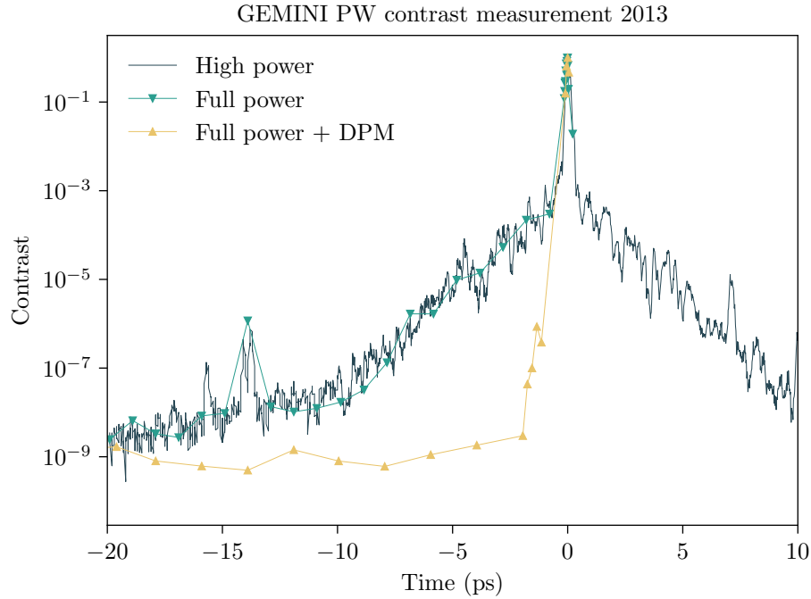
Figure 4.7: Native contrast of the GEMINI PW laser system measured using the Sequoia third order autocorrelator scans. The noise floor of the detector is \approx 1 \times 10^{-9} . The resolution is 100 fs, thus the main pulse is not resolved by the detector.
