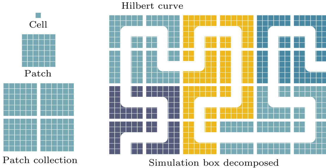
Figure 1.5: SMILEI simulation box decomposition into cells, patches and MPI patch collections. Cells are grouped into patches, patches are grouped into MPI patch collections. These collections are assigned patches contiguously along the Hilbert curve.
