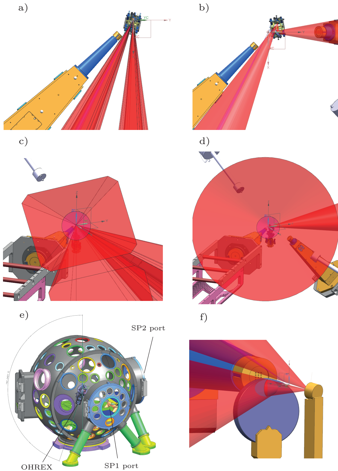
Figure 3.13: CAD images of the ORION target chamber set up for this experiment. a) and b) SP1 and SP2 beamlines respectively from parabola to TCC to OHREX spectrometer. c) and d) SP1 and SP2 beamlines respectively looking from OHREX to TCC. e) Annotated ORION target chamber model. f) SP2 beamline reflecting off plasma mirror before main target incidence.
