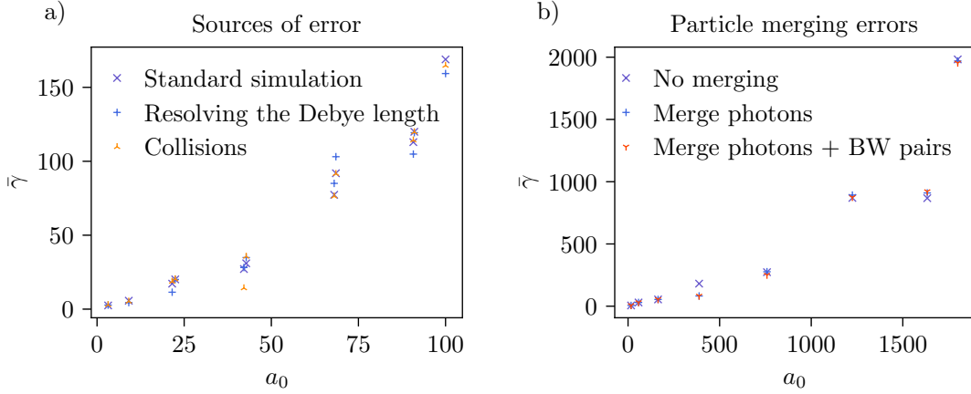
Figure 2.14: An exploration of ZVP 2D PIC simulation stability and assumptions. Additional simulation parameters are given in Table B.1. a) Electron bunch mean energies extracted from simulations with a_0 , \bar{n}_e = 100 . Here, the x -axis is the normalised vector potential of the laser pulse cycle that made them, this is why there appears to be results stacked. b) Electron bunch mean energies extracted from simulations with a_0 , \bar{n}_e = 1800 both with and without particle merging.
