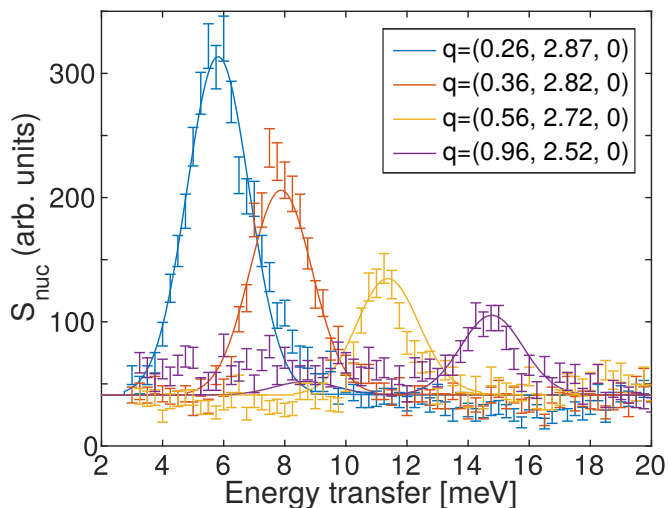
FIG. 8. Measured phonon spectra (error bars) at T = 100 K in direct comparison to the model of acoustic phonons (solid lines) on a triangular lattice, Eq. (B1), calculated using Eq. (C3) setting \sqrt{C/m} = 6.05 meV.
