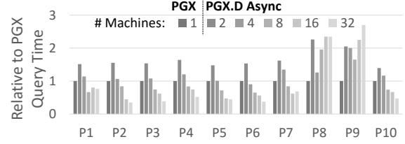
Figure 5. Relative (to PGX) time to complete BSBM queries.
