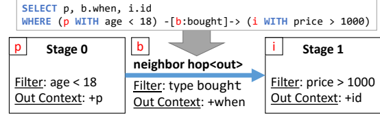
Figure 1. Example: From a PGQL query to PGX.D Async stages.
