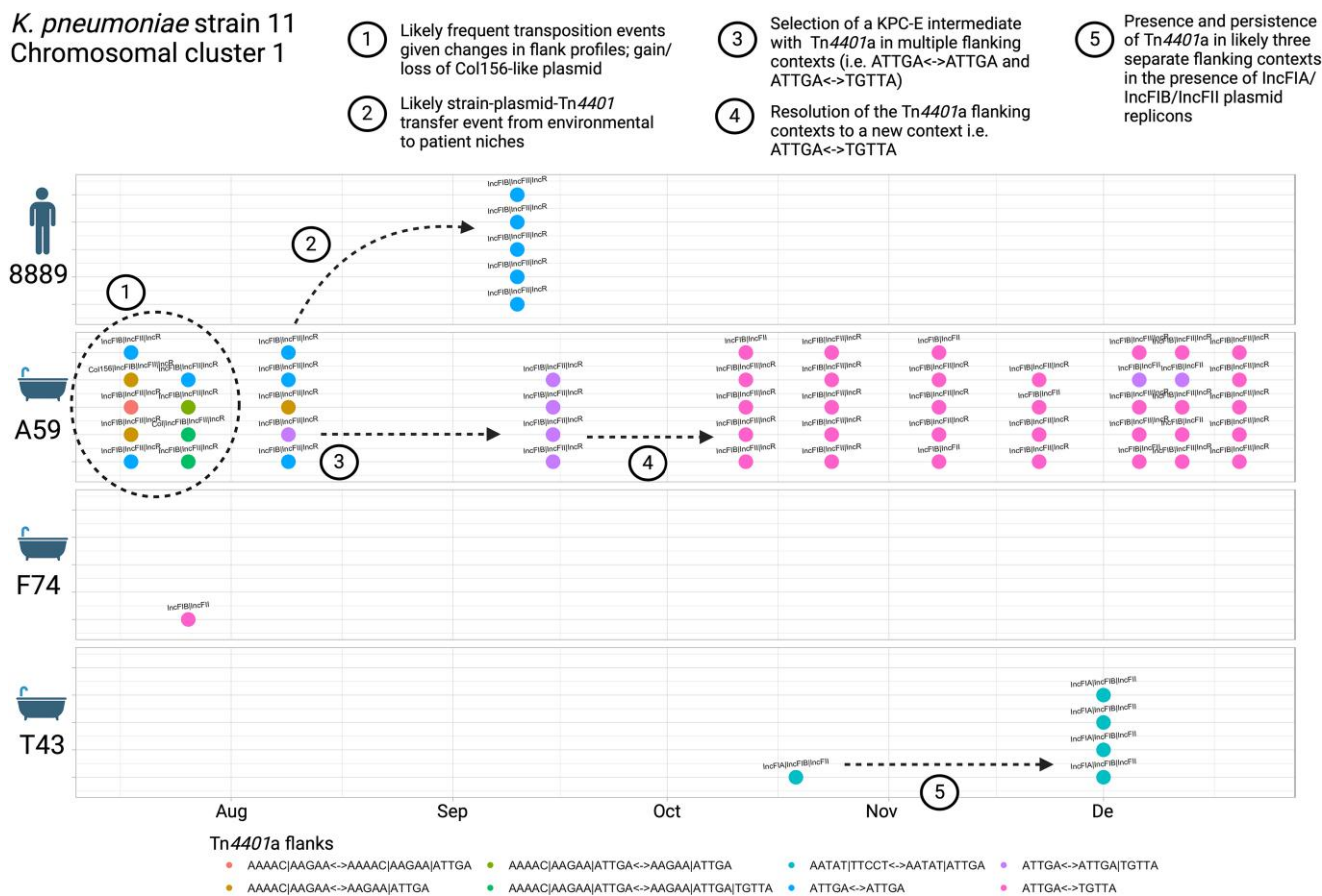
Figure 8. Klebsiella pneumoniae strain 11 cluster 1: features of population structure and transmission dynamics—multiple Tn4401 transposition events. Examples of possible transmission/genetic events are annotated on the figure. Each isolate sequenced is represented as a dot, with colour denoting the TSS profiles observed. Plasmid replicon profiles are annotated as text. (Figure generated in ggplot and www.biorender.com).
