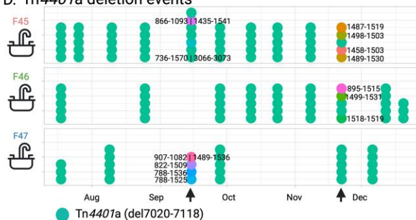
Figure 6. Enterobacter cloacae strain 10: features of population structure and transmission dynamics—niche restriction, persistence and genetic turn-over. Summaries of (a) chromosomal SNP distances for E. cloacae strain 10 across the three sites it colonized; (bi) AMR and (bii) IS profiles; (c) plasmid replicon profiles; and (d) deletions in Tn4401a in isolates. Each sequenced isolate is plotted as a dot reflecting within-sample diversity at given time-points and longitudinally, with colour in panels (bi) and b(ii) reflecting distinct AMR and IS profiles respectively and numbers within the dots representing the numeric identifier for profiles listed in Supplementary dataset 1 .
