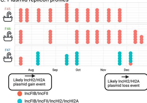
Figure 6. Enterobacter cloacae strain 10: features of population structure and transmission dynamics—niche restriction, persistence and genetic turn-over. Summaries of (a) chromosomal SNP distances for E. cloacae strain 10 across the three sites it colonized; (bi) AMR and (bii) IS profiles; (c) plasmid replicon profiles; and (d) deletions in Tn4401a in isolates. Each sequenced isolate is plotted as a dot reflecting within-sample diversity at given time-points and longitudinally, with colour in panels (bi) and b(ii) reflecting distinct AMR and IS profiles respectively and numbers within the dots representing the numeric identifier for profiles listed in Supplementary dataset 1 .
