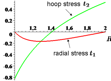
Fig. 1.12 Residual stress in a deformed neo-Hookean tube after anisotropic growth. ( A = 1 , B = 2 , \mu = 1 .)
