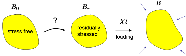
Fig. 1.6 Conceptual schematic for the theory developed here. A stress free reference configuration \mathcal{B}_0 is sought, such that in the deformation from \mathcal{B}_0 to \mathcal{B}_r residual stress develops due to growth of volume elements.
