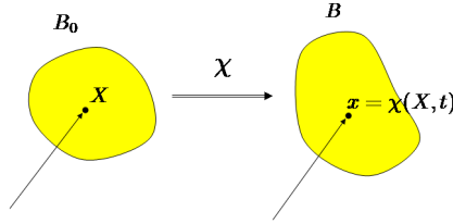
Fig. 1.5 Deformation \chi from reference configuration \mathcal{B}_0 to current configuration \mathcal{B} .
