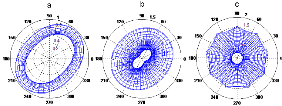
Fig. 1.14 Tube deformation after bifurcation corresponding to the points marked in Figure 1.13. Note that the amplitude has been chosen to illustrate the structure - it has no physical significance since the shapes are produced in a linear stability analysis.
