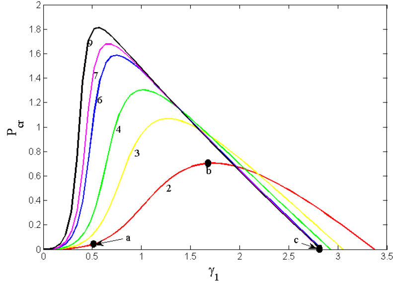
Fig. 1.13 Critical buckling pressure as a function of radial growth \gamma_1 for modes n = 2, 3, 4, 6, 7, 9 .
