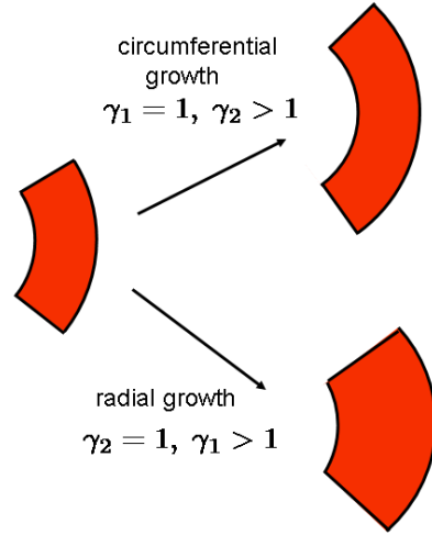
Fig. 1.11 Transformation of an area element under circumferential and radial growth.
