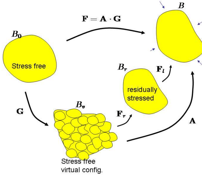
Fig. 1.8 Schematic for the decomposition of the deformation tensor \mathbf{F} into the growth tensor \mathbf{G} and the elastic deformation tensor \mathbf{A} . The tensor \mathbf{A} in turn is comprised of the reorganization deformation \mathbf{F}_r , in which residual stress is introduced, and the deformation due to loading, \mathbf{F}_l .
