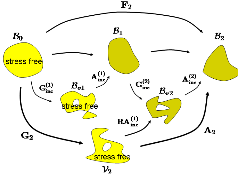
Fig. 1.9 Two incremental steps. The total growth tensor \mathbf{G}_2 is defined after creating a map from the stress free virtual configuration \mathcal{V}_2 to the stressed virtual configuration \mathcal{B}_{v2} .
