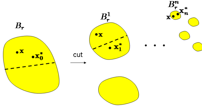
Fig. 1.7 The residually stressed body \mathcal{B}_r is repeatedly cut, relieving stress. As the number of cuts n \rightarrow \infty , the distance between the point \mathbf{x} and the stress free point \mathbf{x}^* goes to zero.
