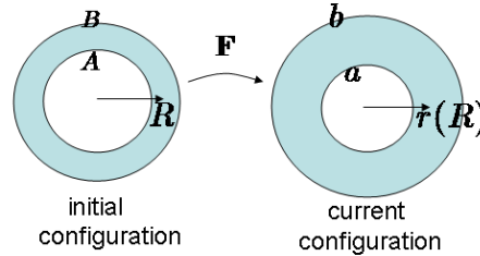
Fig. 1.10 Geometry for the growing cylindrical tube before and after deformation.
