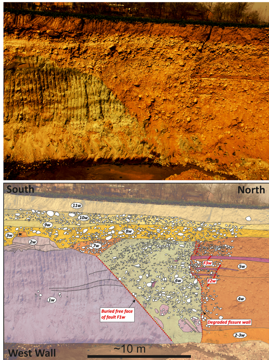
Figure 8. Interpretation of the western trench wall at the Chishui site. (top) Original photograph. (bottom) Trench log. The fault surface F1w was exhumed as a free face and then buried by fissure infill (6w). This buried free face and the degraded fissure wall to the north are shown as dotted red lines. White filled polygons are gravel clasts.
